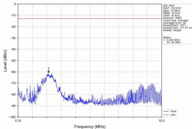
Band25_20MHz_16QAM_MCH_1882.5MHz_RB_1_0_NTNV
