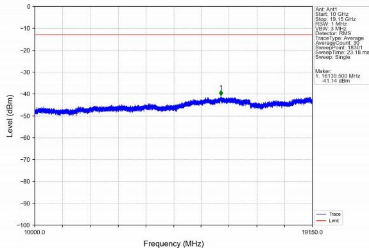
Band25_20MHz_QPSK_MCH_1882.5MHz_RB_1_0_NTNV
