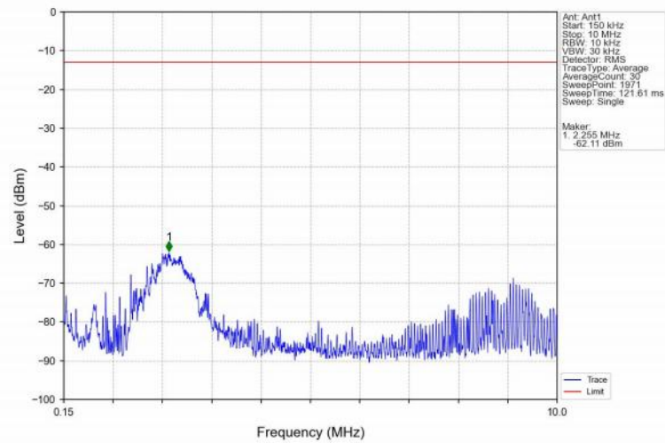
Band25_20MHz_16QAM_HCH_1905MHz_RB_1_0_NTNV
