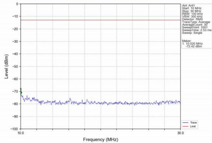
Band25_3MHz_16QAM_LCH_1851.5MHz_RB_1_0_NTNV
