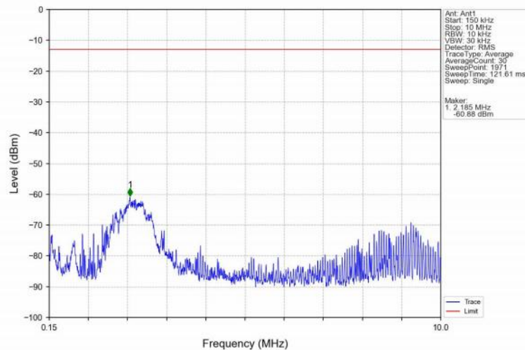
Band25_15MHz_16QAM_MCH_1882.5MHz_RB_1_0_NTNV
