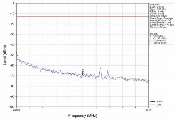
Band25_10MHz_16QAM_LCH_1855MHz_RB_1_0_NTNV
