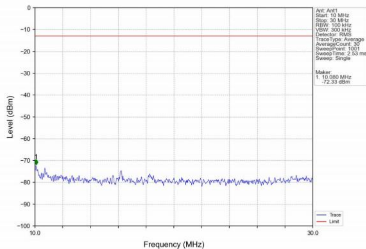
Band25_5MHz_QPSK_MCH_1882.5MHz_RB_1_0_NTNV
