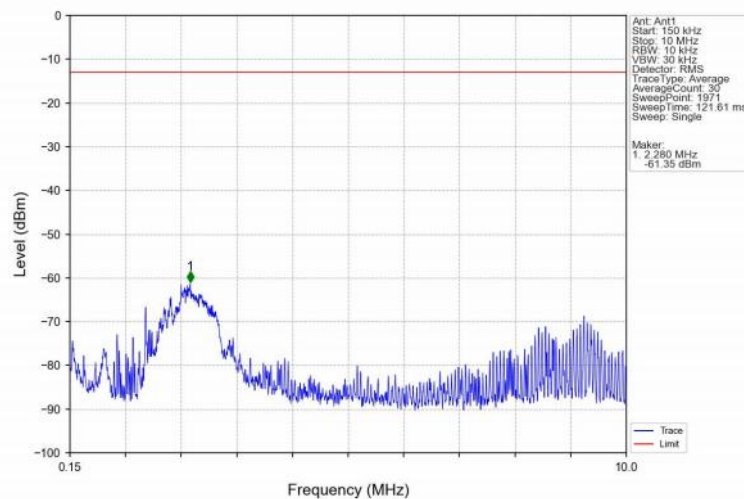
Band25_5MHz_16QAM_MCH_1882.5MHz_RB_1_0_NTNV
