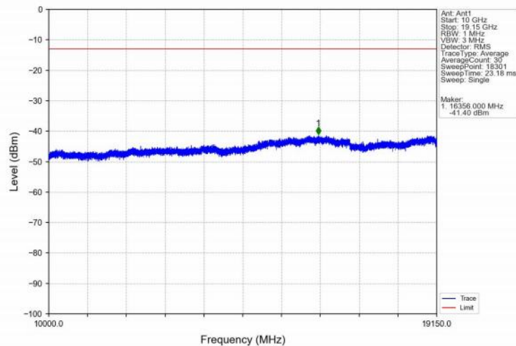
Band25_3MHz_QPSK_MCH_1882.5MHz_RB_1_0_NTNV
