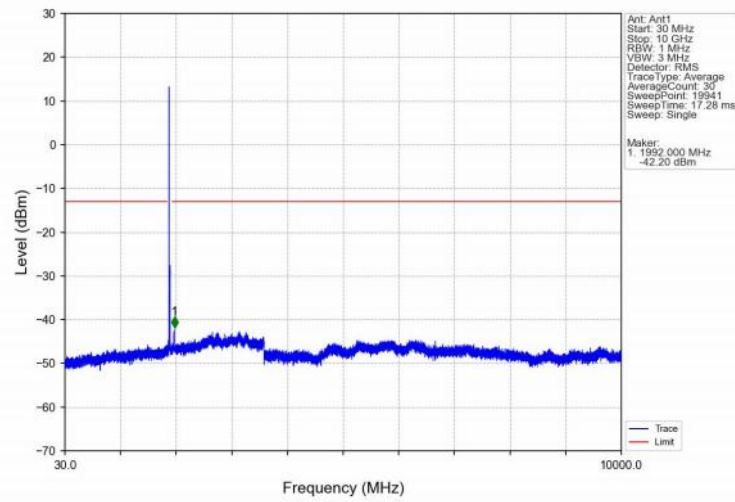
Band25_20MHz_16QAM_HCH_1905MHz_RB_1_0_NTNV
