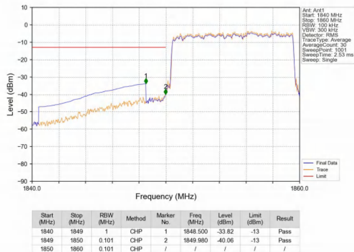
Band25_10MHz_16QAM_LCH_1855MHz_RB_50_0_NTNV
