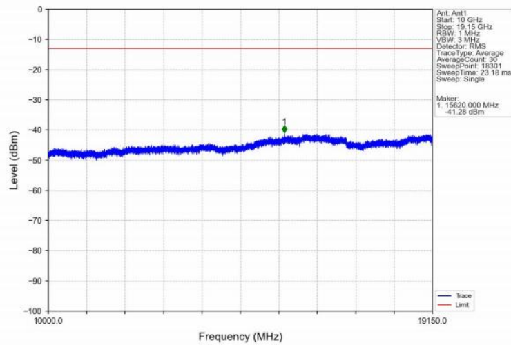
Band25_20MHz_16QAM_LCH_1860MHz_RB_100_0_NTNV
