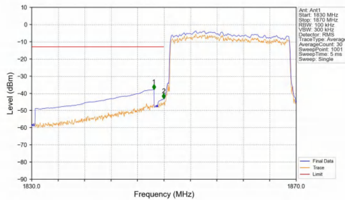
Band25_20MHz_16QAM_LCH_1860MHz_RB_100_0_NTNV
