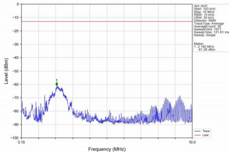
Band25_3MHz_16QAM_MCH_1882.5MHz_RB_1_0_NTNV
