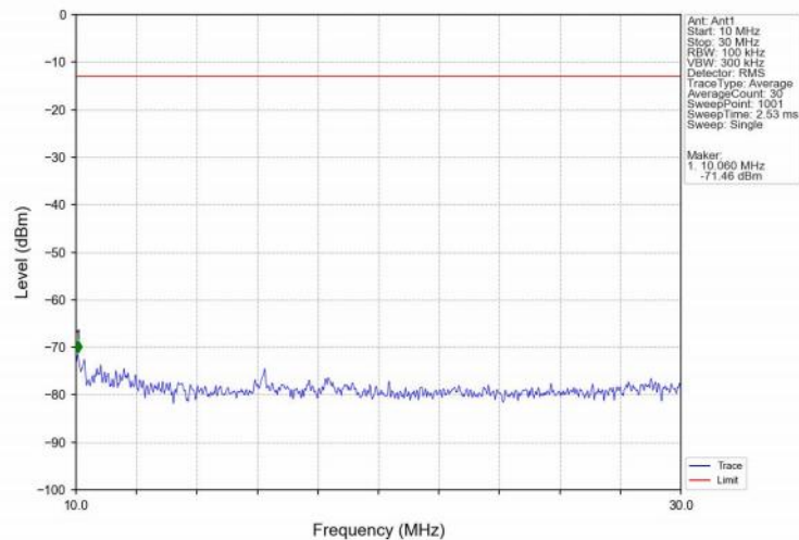
Band25_20MHz_QPSK_MCH_1882.5MHz_RB_1_0_NTNV
