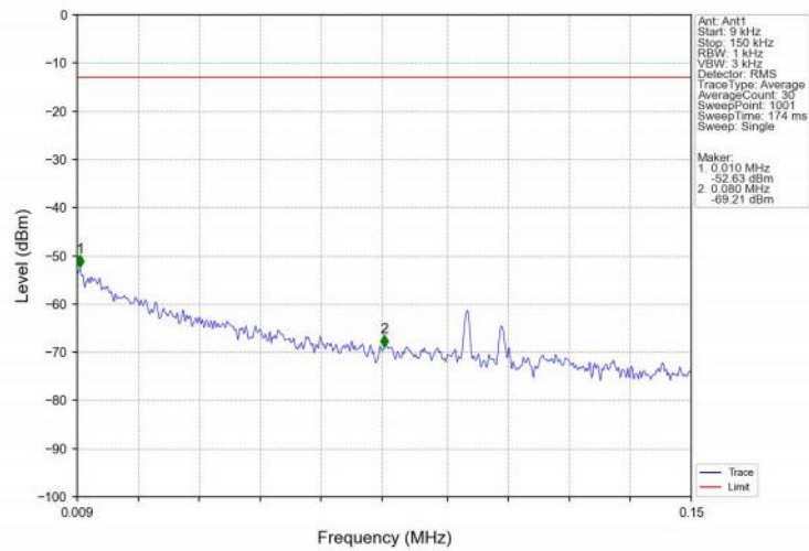
Band25_3MHz_16QAM_MCH_1882.5MHz_RB_1_0_NTNV
