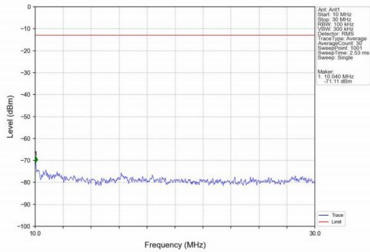
Band25_10MHz_16QAM_MCH_1882.5MHz_RB_1_0_NTNV
