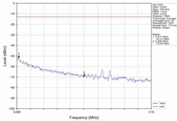
Band66_15MHz_16QAM_LCH_1717.5MHz_RB_1_0_NTNV
