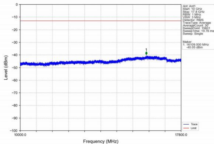
Band66_5MHz_QPSK_MCH_1745MHz_RB_1_0_NTNV
