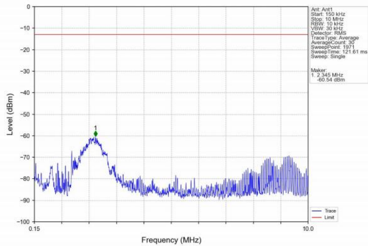
Band66_3MHz_QPSK_MCH_1745MHz_RB_1_0_NTNV
