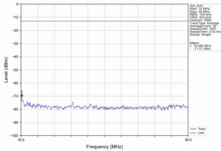
Band66_5MHz_16QAM_MCH_1745MHz_RB_1_0_NTNV
