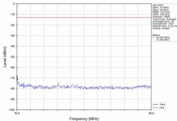
Band66_3MHz_16QAM_HCH_1778.5MHz_RB_1_0_NTNV
