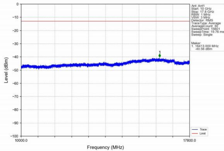
Band66_3MHz_QPSK_HCH_1778.5MHz_RB_1_14_NTNV
