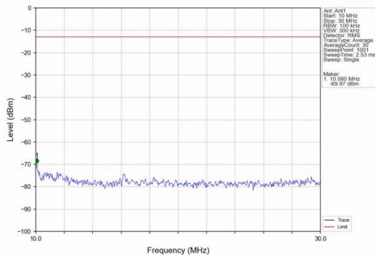
Band66_5MHz_QPSK_MCH_1745MHz_RB_1_0_NTNV
