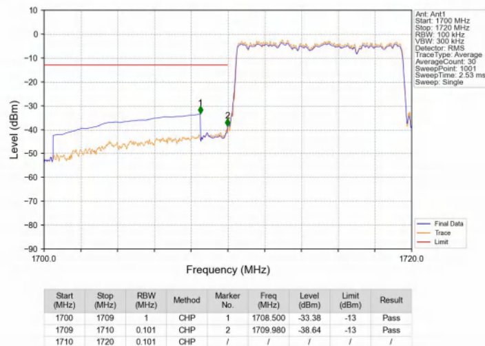
Band66_10MHz_16QAM_LCH_1715MHz_RB_50_0_NTNV
