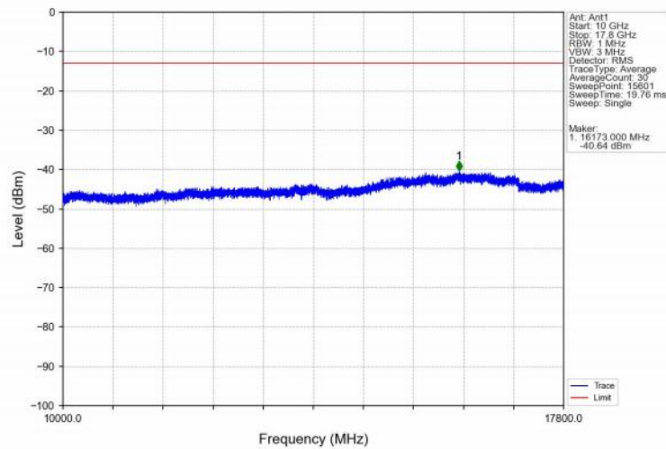
Band66_3MHz_QPSK_MCH_1745MHz_RB_1_0_NTNV
