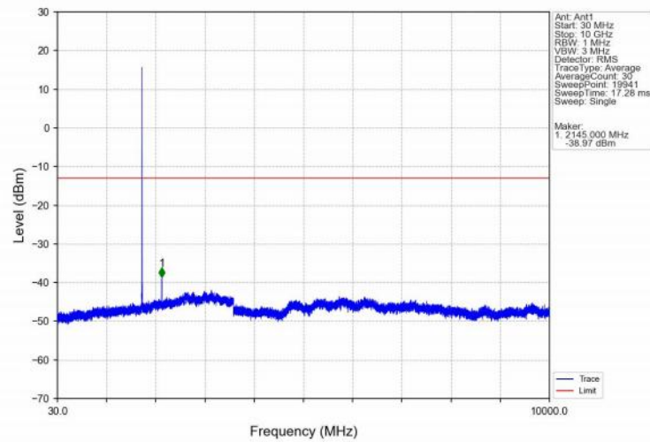
Band66_5MHz_QPSK_MCH_1745MHz_RB_1_0_NTNV
