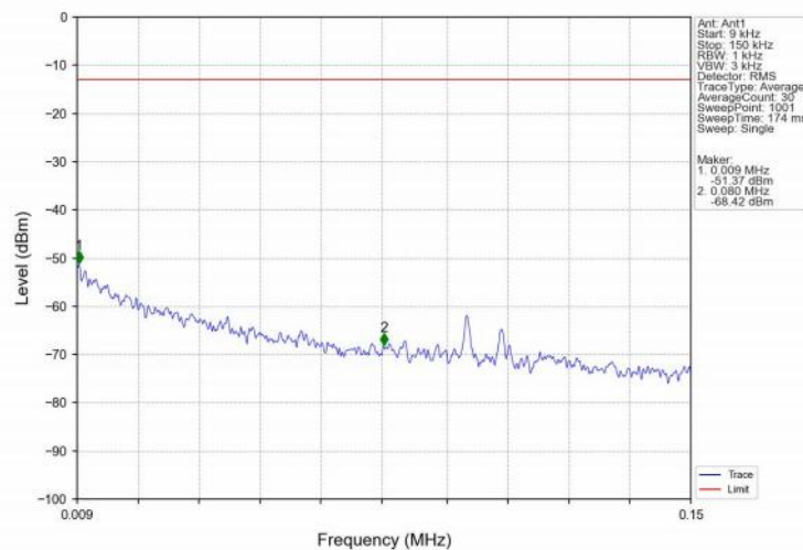
Band66_3MHz_16QAM_HCH_1778.5MHz_RB_1_0_NTNV
