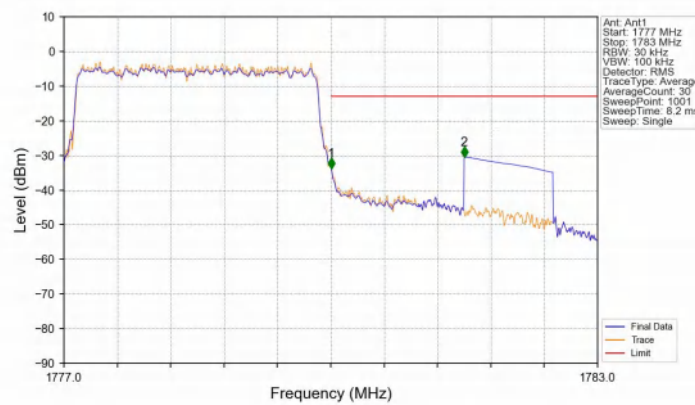
Band66_3MHz_16QAM_HCH_1778.5MHz_RB_15_0_NTNV
