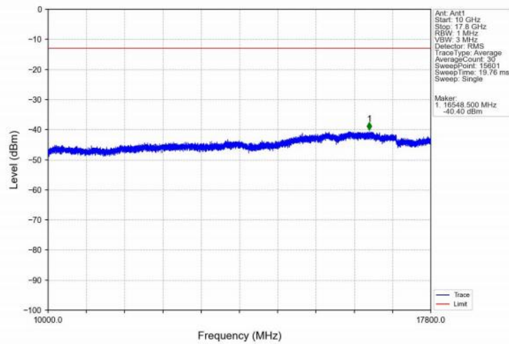
Band66_15MHz_16QAM_LCH_1717.5MHz_RB_75_0_NTNV
