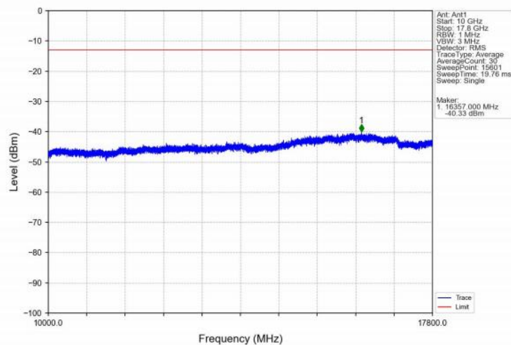
Band66_10MHz_QPSK_LCH_1715MHz_RB_1_0_NTNV
