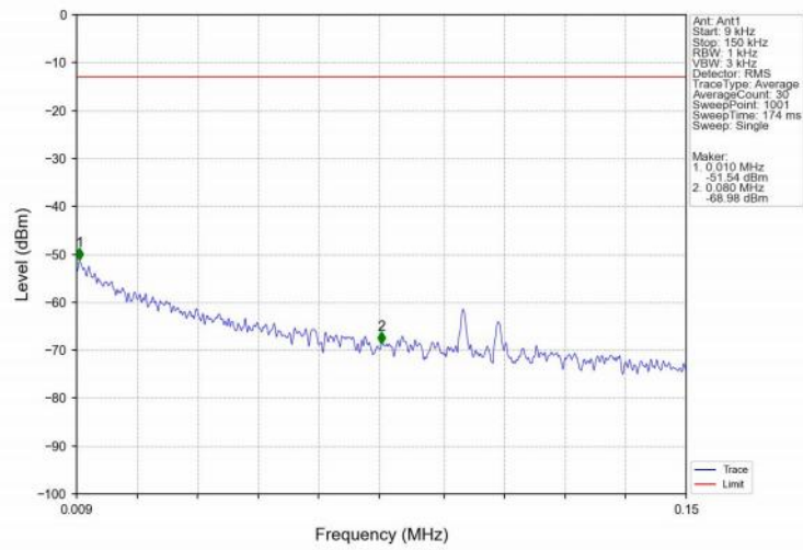
Band66_10MHz_16QAM_LCH_1715MHz_RB_1_0_NTNV
