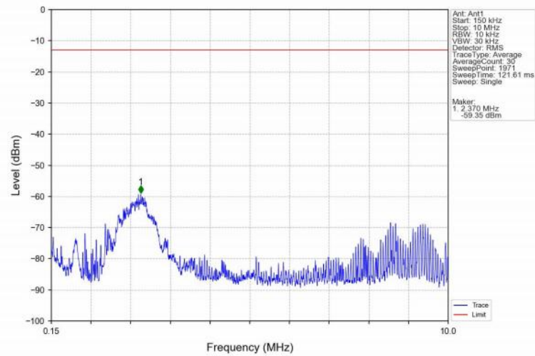
Band66_10MHz_QPSK_LCH_1715MHz_RB_1_0_NTNV
