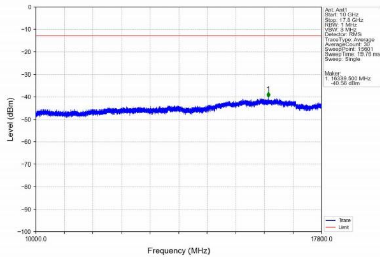
Band66_15MHz_QPSK_HCH_1772.5MHz_RB_1_74_NTNV
