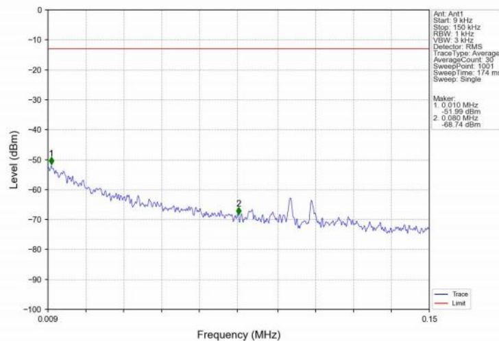
Band66_15MHz_QPSK_LCH_1717.5MHz_RB_1_0_NTNV
