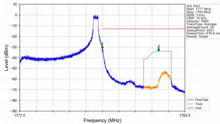
Band66_3MHz_16QAM_HCH_1778.5MHz_RB_1_14_NTNV
