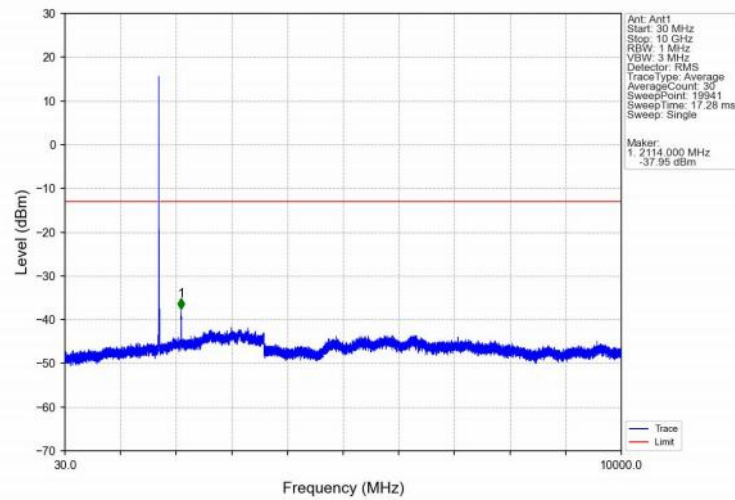
Band66_10MHz_QPSK_LCH_1715MHz_RB_1_0_NTNV
