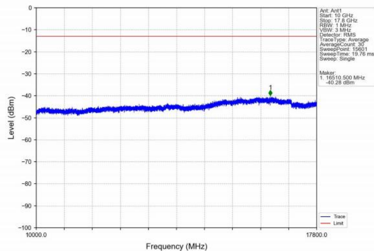
Band66_15MHz_QPSK_LCH_1717.5MHz_RB_1_0_NTNV
