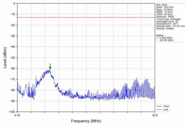
Band66_5MHz_QPSK_MCH_1745MHz_RB_1_0_NTNV
