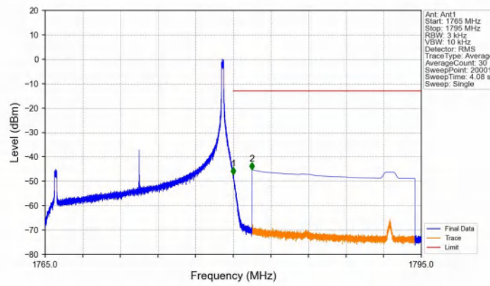
Band66_15MHz_QPSK_HCH_1772.5MHz_RB_1_74_NTNV
