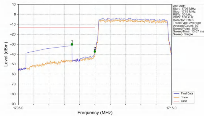
Band66_5MHz_16QAM_LCH_1712.5MHz_RB_25_0_NTNV
