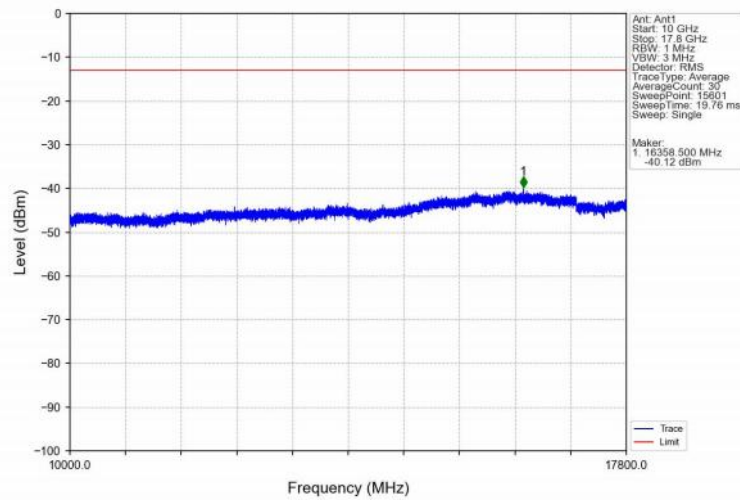
Band66_3MHz_16QAM_HCH_1778.5MHz_RB_1_0_NTNV
