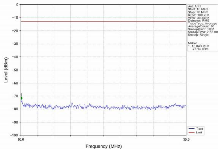
Band66_3MHz_QPSK_MCH_1745MHz_RB_1_0_NTNV
