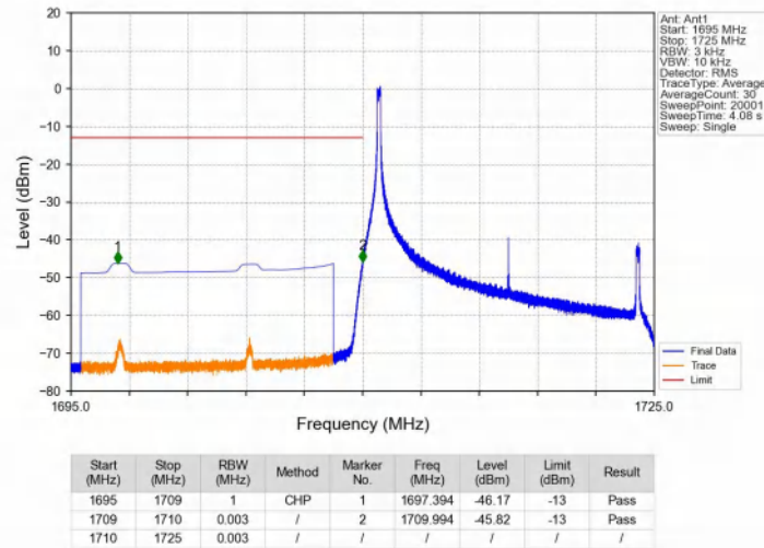
Band66_15MHz_QPSK_LCH_1717.5MHz_RB_1_0_NTNV
