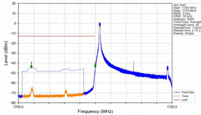
Band66_10MHz_QPSK_LCH_1715MHz_RB_1_0_NTNV
