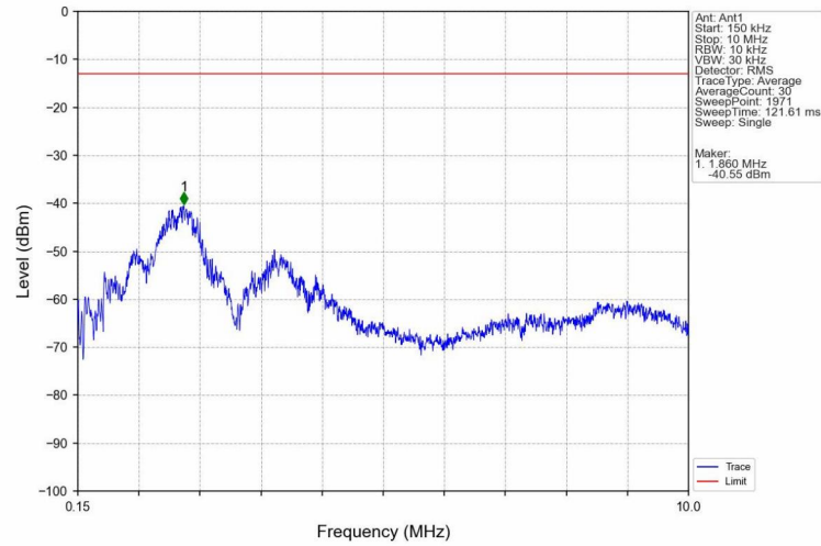
Band2_HSDPA_HCH_1907.6MHz_Subtest 1_NTNV
