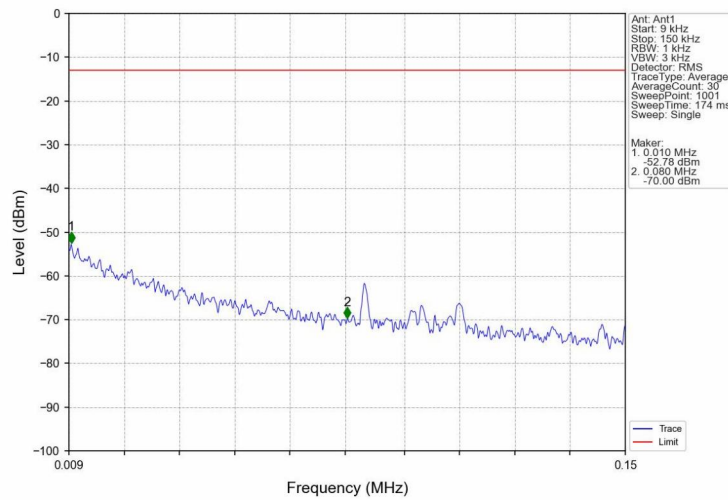
Band2_HSUPA_LCH_1852.4MHz_Subtest 1_NTNV
