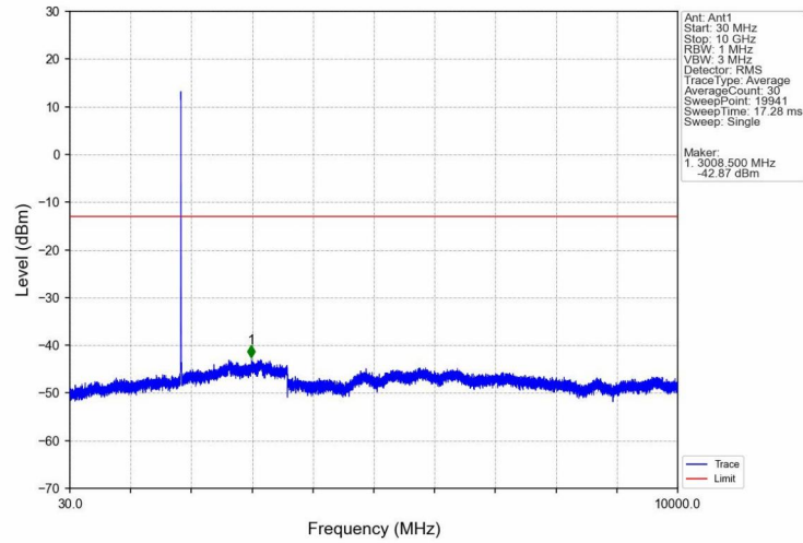
Band2_HSUPA_LCH_1852.4MHz_Subtest 1_NTNV
