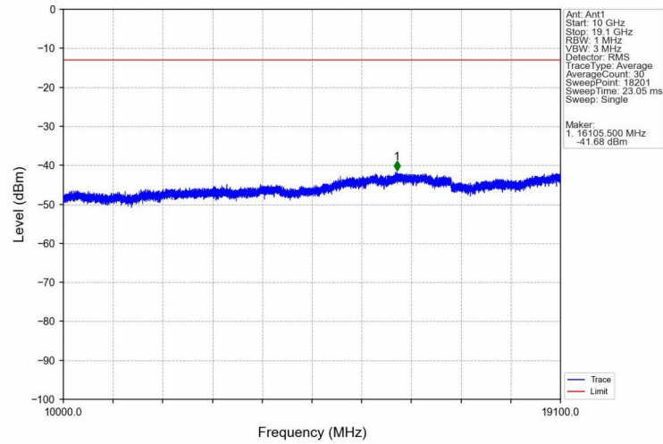
Band2_HSUPA_HCH_1907.6MHz_Subtest 1_NTNV
