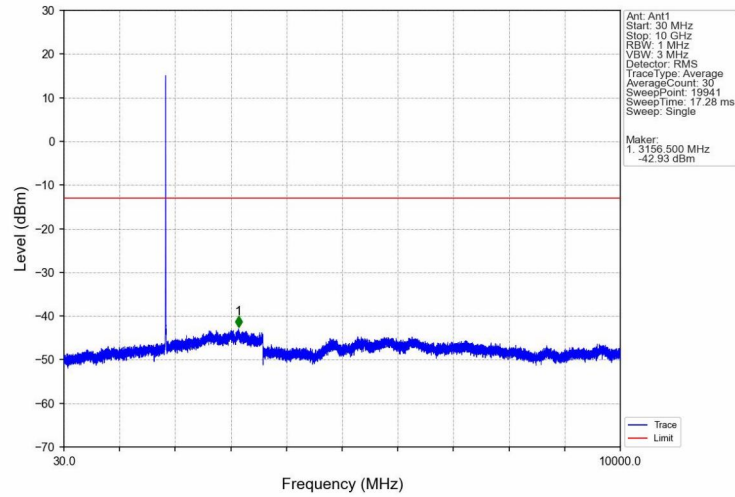
Band2_RMC_LCH_1852.4MHz_12.2kbps RMC_NTNV
