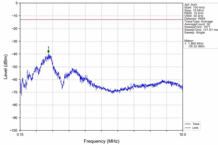
Band2_HSDPA_MCH_1880MHz_Subtest 1_NTNV
