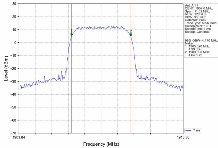
Band2_HSUPA_HCH_1907.6MHz_Subtest 1_NTNV
