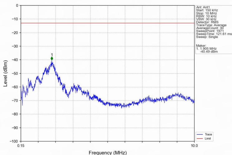
Band2_RMC_MCH_1880MHz_12.2kbps RMC_NTNV
