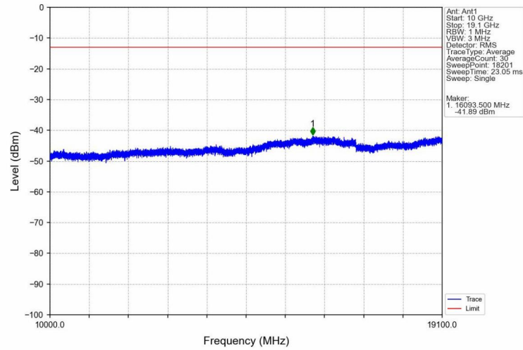
Band2_HSDPA_LCH_1852.4MHz_Subtest 1_NTNV
