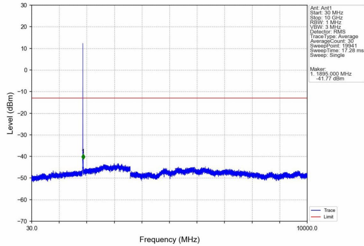
Band2_HSDPA_MCH_1880MHz_Subtest 1_NTNV
