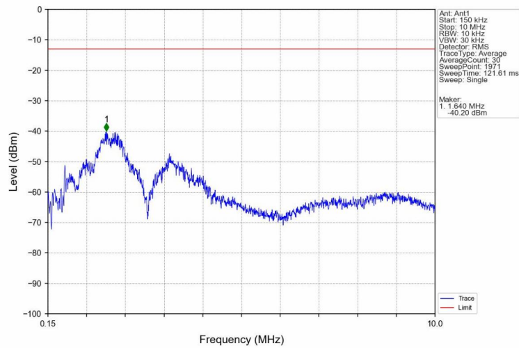
Band4_HSDPA_LCH_1712.4MHz_Subtest 1_NTNV
