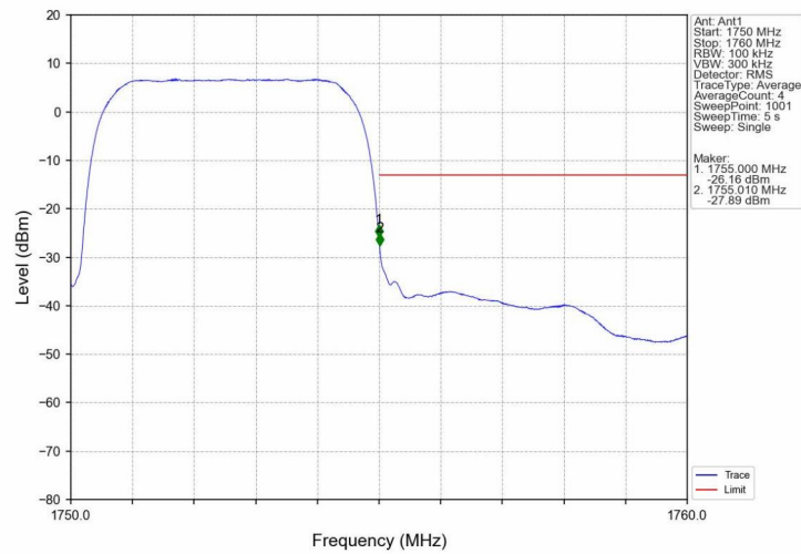
Band4_RMC_HCH_1752.6MHz_12.2kbps_RMC_NTNV
