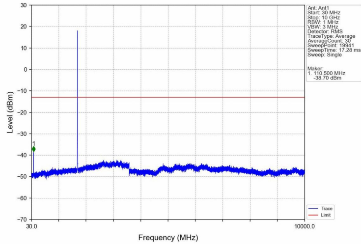
Band4_RMC_LCH_1712.4MHz_12.2kbps RMC_NTNV
