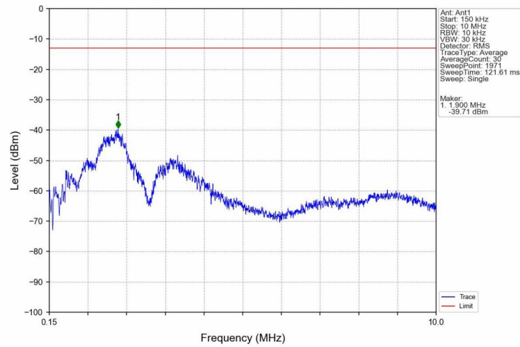
Band4_HSDPA_HCH_1752.6MHz_Subtest 1_NTNV
