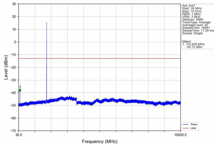
Band4_HSUPA_HCH_1752.6MHz_Subtest 1_NTNV
