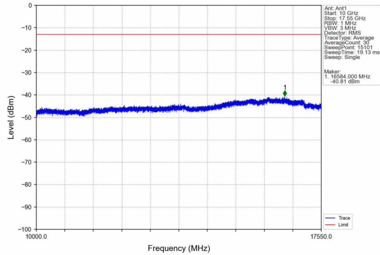
Band4_HSDPA_LCH_1712.4MHz_Subtest 1_NTNV
