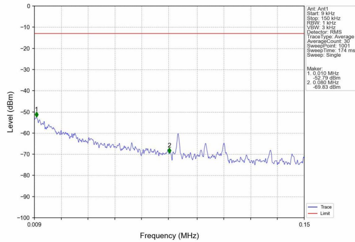
Band4_RMC_HCH_1752.6MHz_12.2kbps RMC_NTNV
