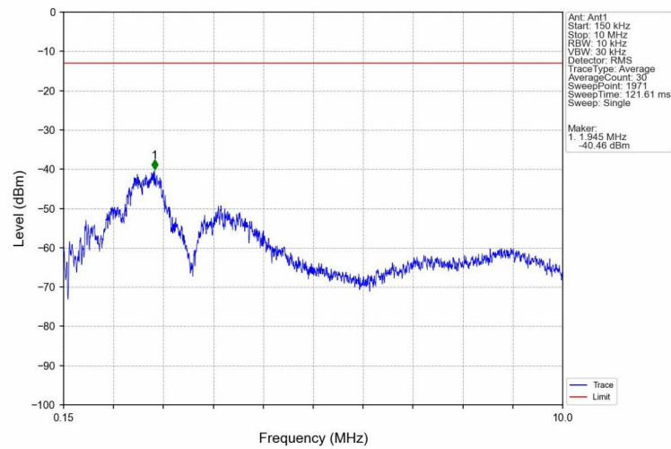
Band4_RMC_HCH_1752.6MHz_12.2kbps RMC_NTNV
