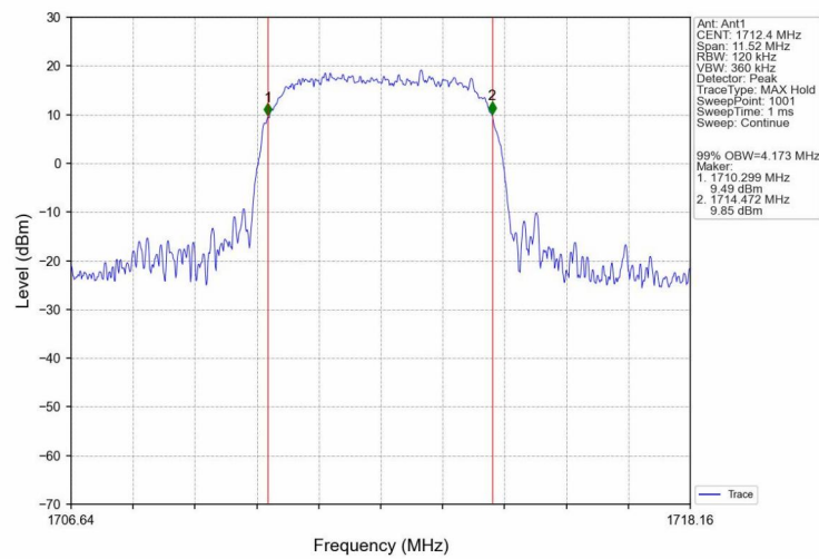
Band4_HSDPA_LCH_1712.4MHz_Subtest 1_NTNV
