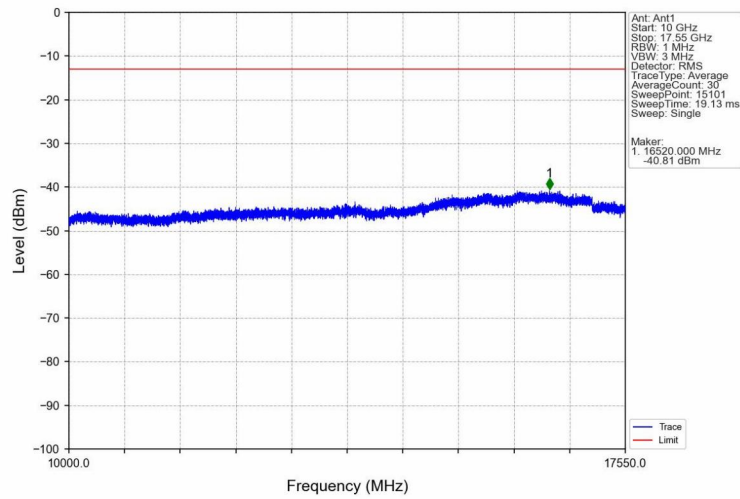
Band4_HSDPA_MCH_1732.6MHz_Subtest 1_NTNV
