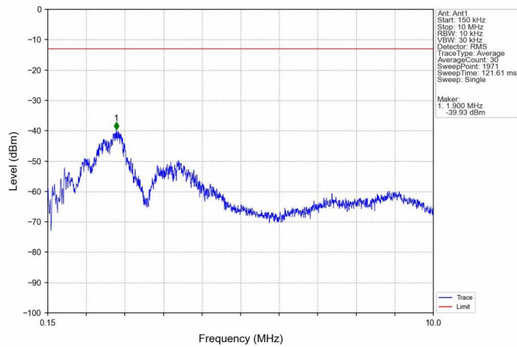
Band4_HSUPA_MCH_1732.6MHz_Subtest 1_NTNV
