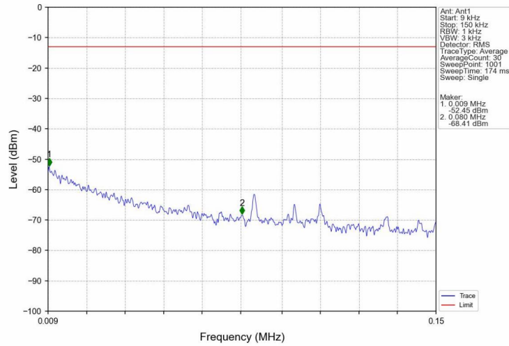
Band4_HSUPA_MCH_1732.6MHz_Subtest 1_NTNV
