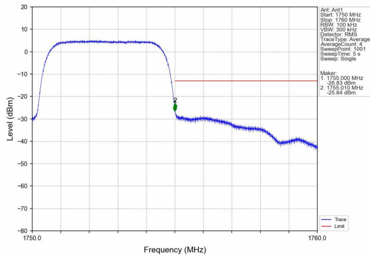
Band4_HSUPA_HCH_1752.6MHz_Subtest 1_NTNV
