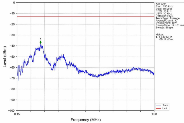
Band4_HSDPA_MCH_1732.6MHz_Subtest 1_NTNV
