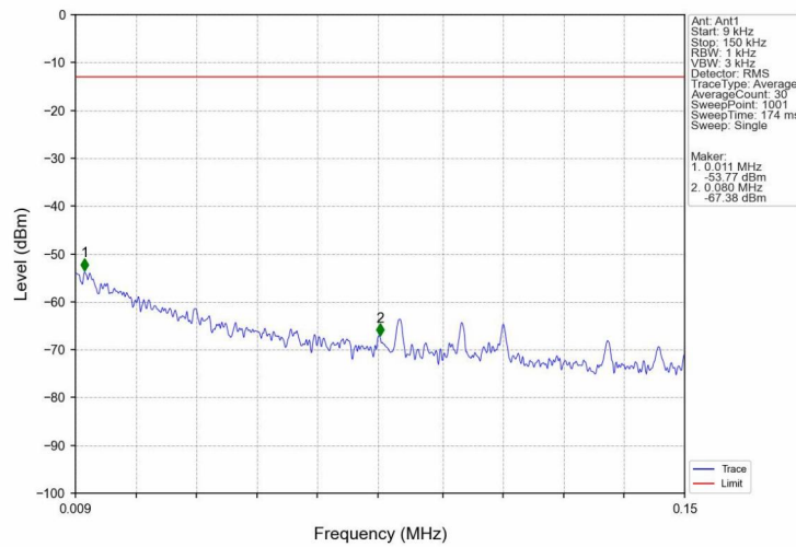
Band4_HSDPA_HCH_1752.6MHz_Subtest 1_NTNV
