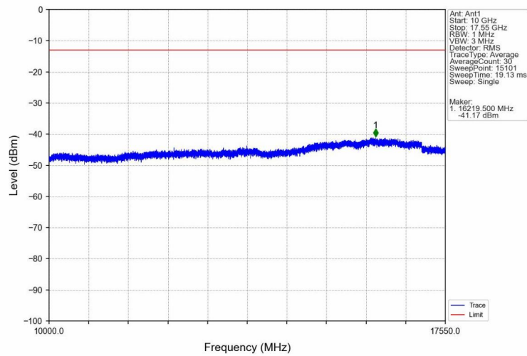
Band4_HSDPA_HCH_1752.6MHz_Subtest 1_NTNV
