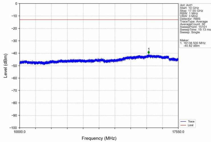
Band4_HSUPA_HCH_1752.6MHz_Subtest 1_NTNV
