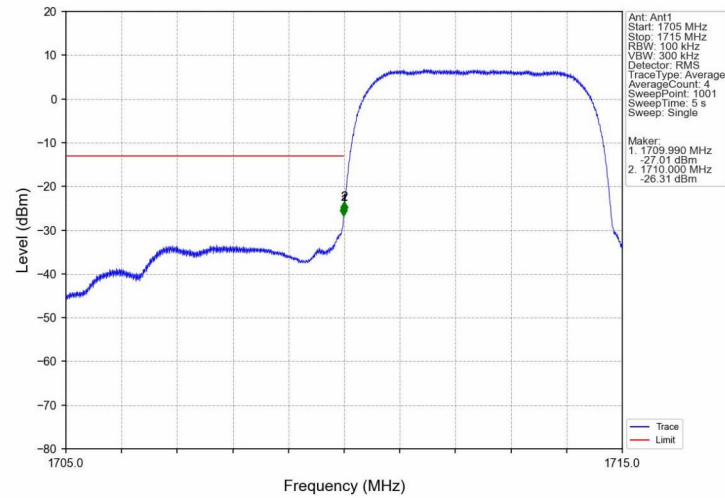
Band4_HSDPA_LCH_1712.4MHz_Subtest 1_NTNV
