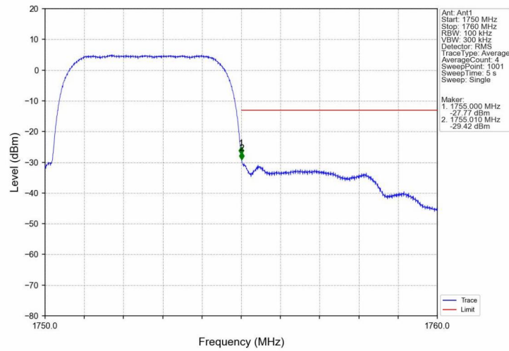
Band4_HSDPA_HCH_1752.6MHz_Subtest 1_NTNV
