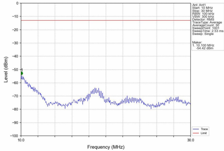
Band4_RMC_HCH_1752.6MHz_12.2kbps RMC_NTNV
