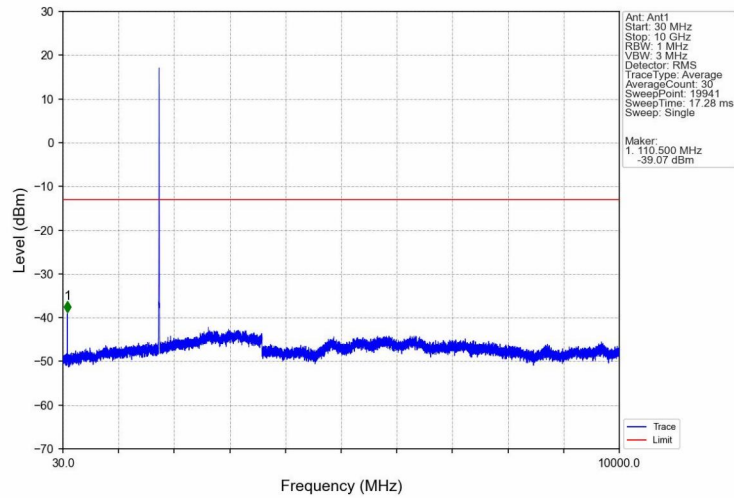
Band4_RMC_HCH_1752.6MHz_12.2kbps RMC_NTNV
