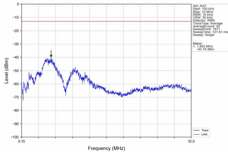
Band4_RMC_MCH_1732.6MHz_12.2kbps_RMC_NTNV
