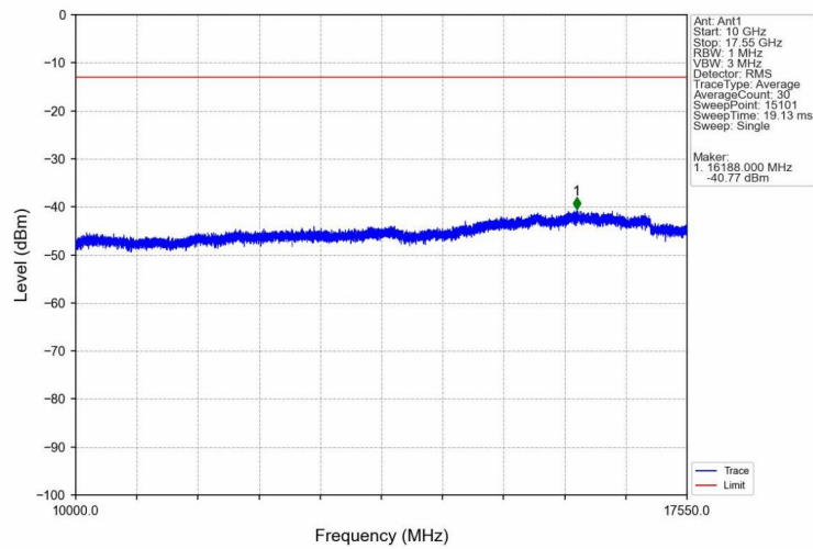
Band4_RMC_LCH_1712.4MHz_12.2kbps RMC_NTNV
