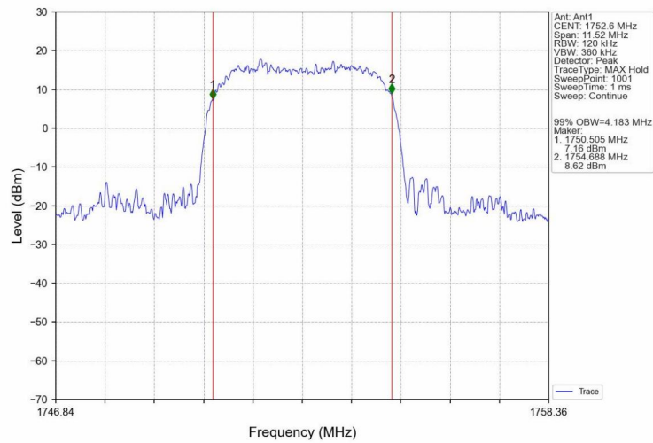
Band4_HSDPA_HCH_1752.6MHz_Subtest 1_NTNV
