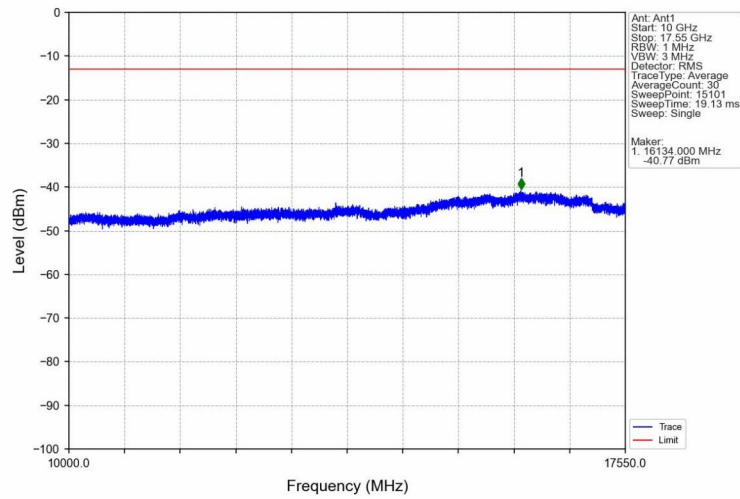
Band4_RMC_HCH_1752.6MHz_12.2kbps_RMC_NTNV
