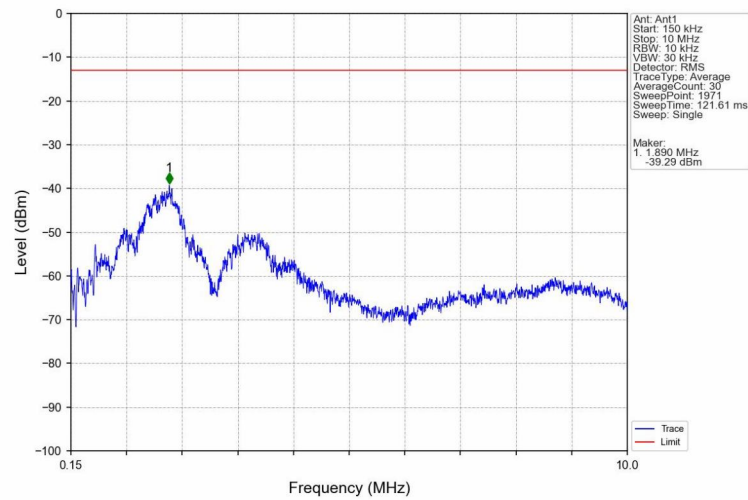
Band4_HSUPA_HCH_1752.6MHz_Subtest 1_NTNV
