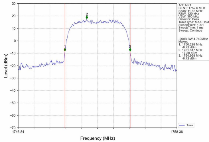
Band4 HSUPA HCH 1752.6MHz_Subtest 1_NTNV
