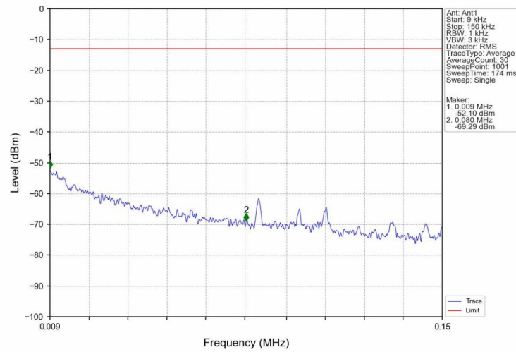
Band4_HSUPA_HCH_1752.6MHz_Subtest 1_NTNV
