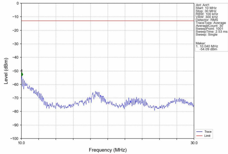
Band4_HSDPA_LCH_1712.4MHz_Subtest 1_NTNV
