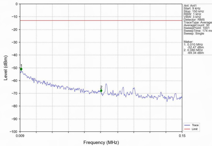
Band4_HSDPA_MCH_1732.6MHz_Subtest 1_NTNV
