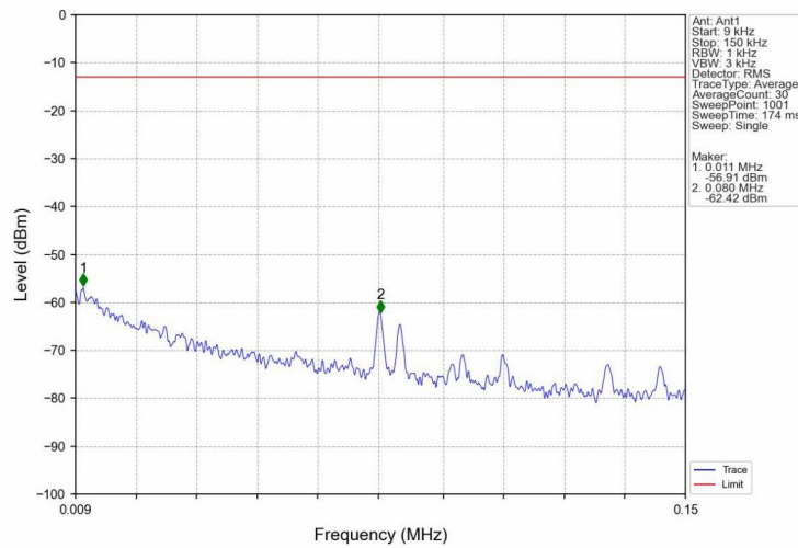
Band5_HSDPA_MCH_836.6MHz_Subtest 1_NTNV
