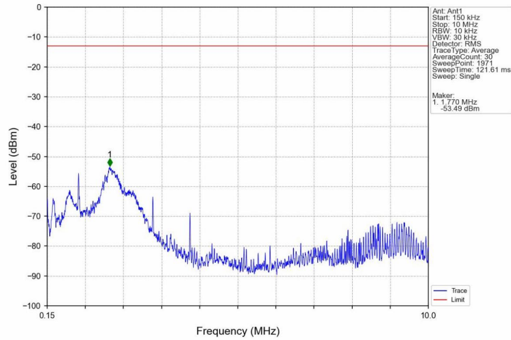
Band5_HSDPA_MCH_836.6MHz_Subtest 1_NTNV
