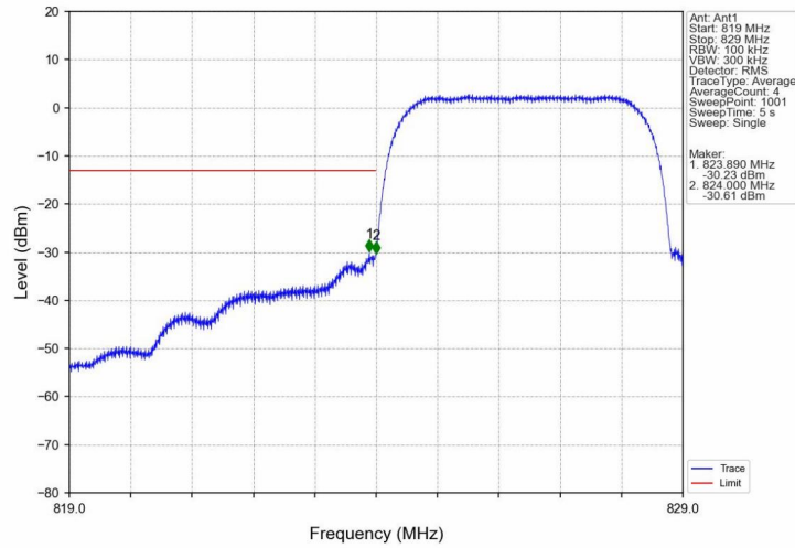
Band5_HSDPA_LCH_826.4MHz_Subtest 1_NTNV
