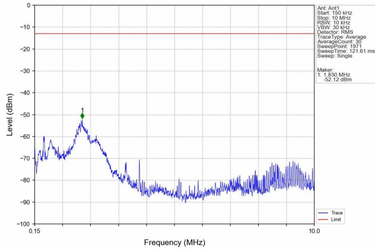
Band5_HSUPA_LCH_826.4MHz_Subtest 1_NTNV
