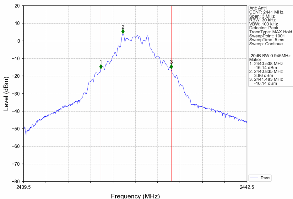
GFSK_DH5_MCH_2441MHz_Ant1_NTNV
