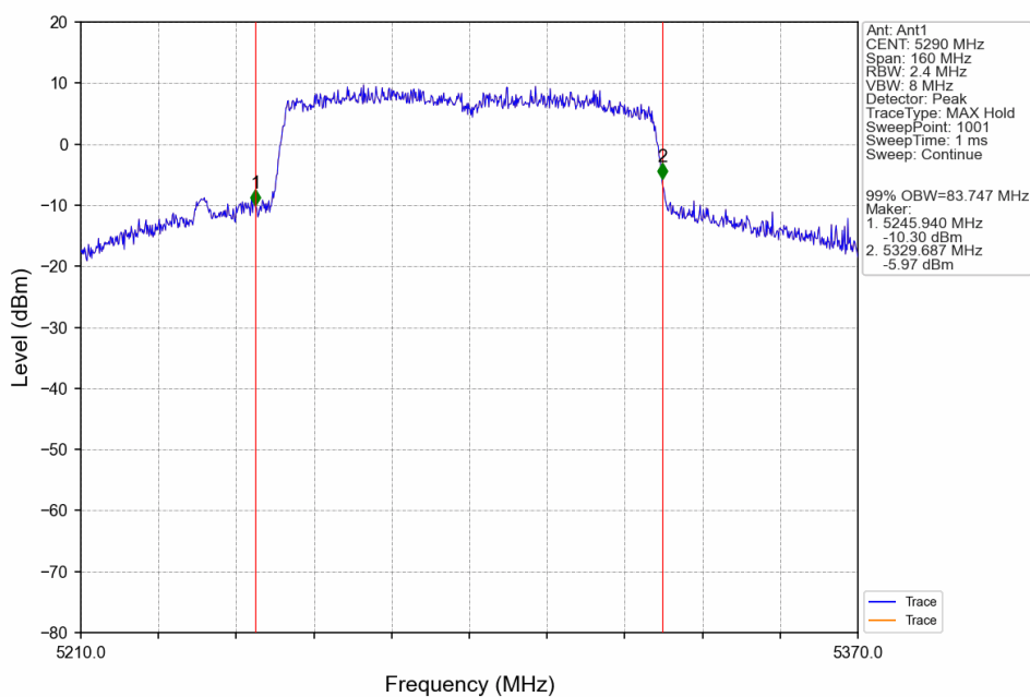
802.11ac(VHT80)_MCH_5290MHz_Ant1_NTNV
