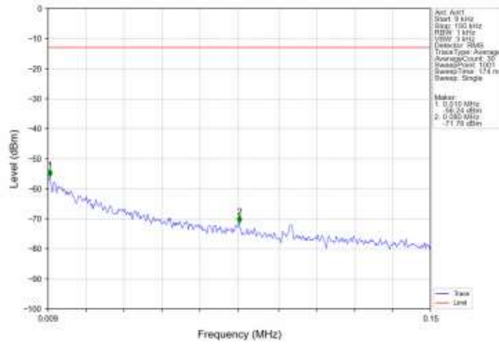
Band17_5MHz_QPSK_MCH_710MHz_RB_1_0_NTNV
