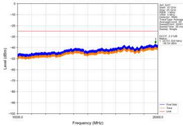
Band41_15MHz_16QAM_HCH_2682.5MHz_RB_1_0_NTNV
