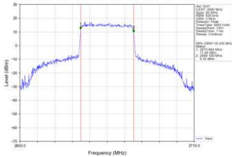
Band41_20MHz_16QAM_HCH_2680MHz_RB_100_0_NTNV
