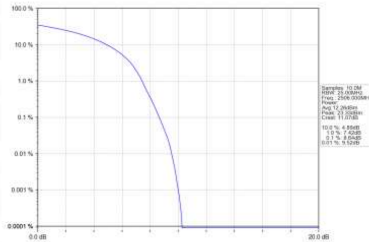
Band41_20MHz_16QAM_LCH_2506MHz_RB_100_0 NTN
