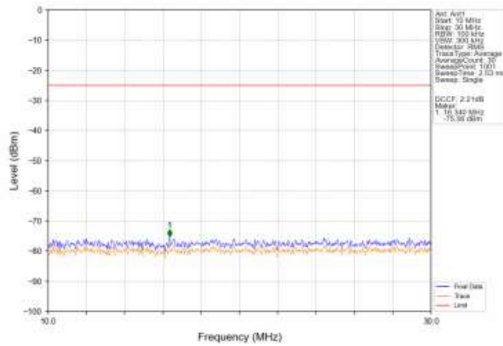
Band41_15MHz_16QAM_LCH_2503.5MHz_RB_1_0_NTNV
