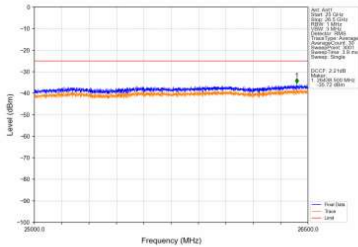
Band41_5MHz_16QAM_HCH_2687.5MHz_RB_1_0_NTNV
