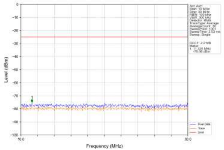
Band41_5MHz_16QAM_LCH_2498.5MHz_RB_1_0_NTNV
