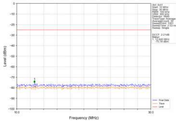
Band41_20MHz_16QAM_LCH_2506MHz_RB_1_0_NTNV
