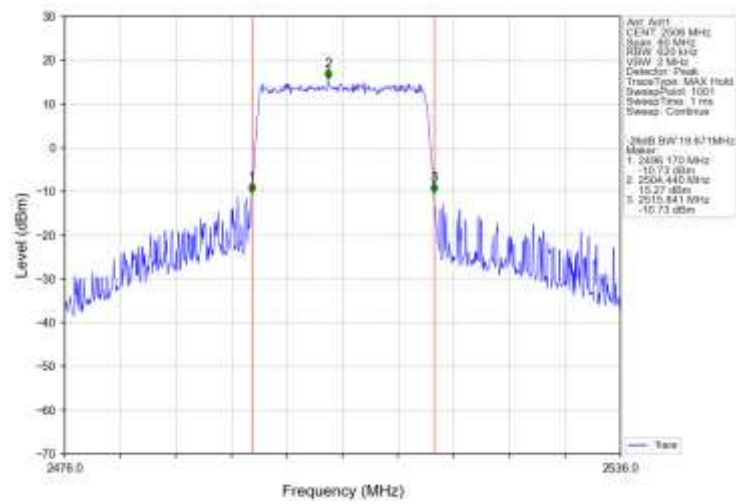
Band41_20MHz_16QAM_LCH_2506MHz_RB_100_0_NTNV
