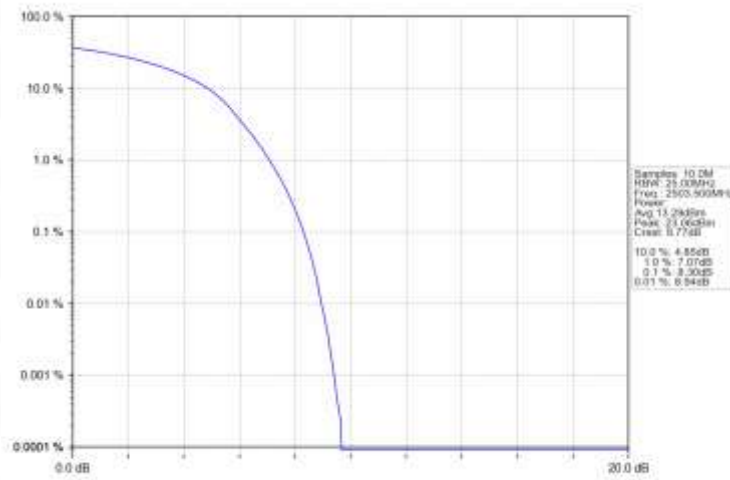
Band41_15MHz_16QAM_LCH_2503.5MHz_RB_75_0_NTNV
