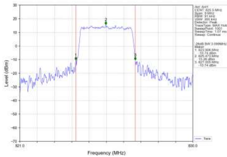
Band5_3MHz_16QAM_LCH_825.5MHz_RB_15_0_NTNV
