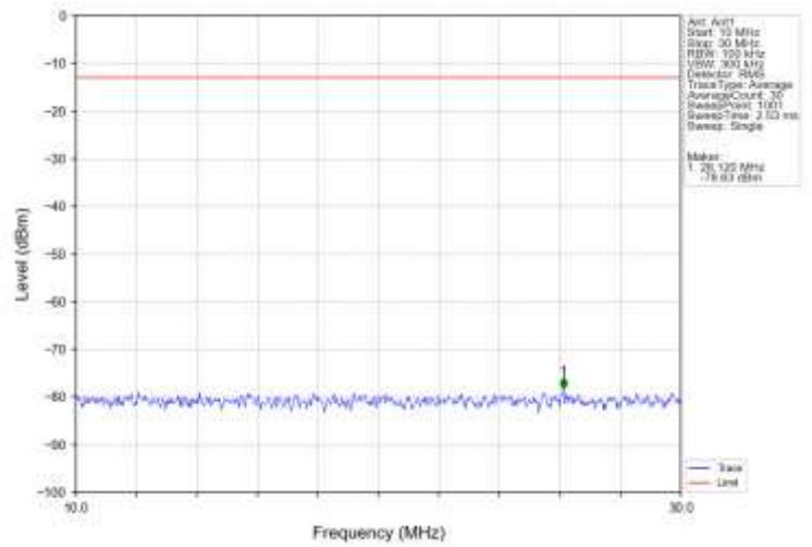
Band5 1.4MHz QPSK LCH 824.7MHz RB 1 0 NTN
