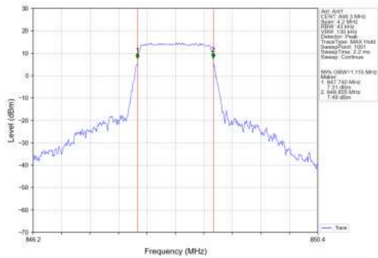
Band5 1.4MHz 16QAM HCH 848.3MHz RB 6 0 NTV
