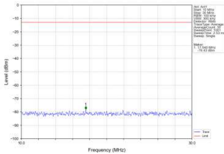
Band5_10MHz_16QAM_LCH_829MHz_RB_1_0_NTNV
