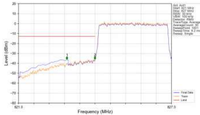
Band5_3MHz_16QAM_LCH_825.5MHz_RB_15_0_NTNV
