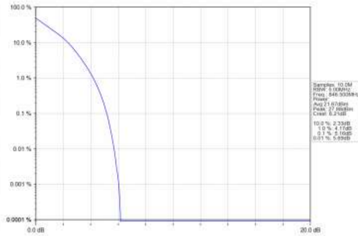
Band5 5MHz QPSK HCH 846.5MHz RB 25 0 NTN
