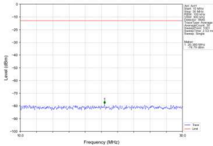
Band5_5MHz_16QAM_LCH_826.5MHz_RB_1_0_NTNV
