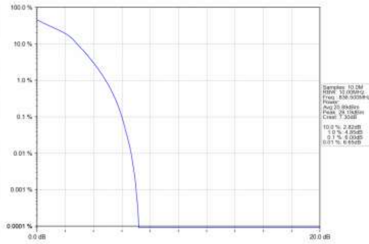
Band5_10MHz_16QAM_MCH_836.5MHz_RB_50_0_NTNV
