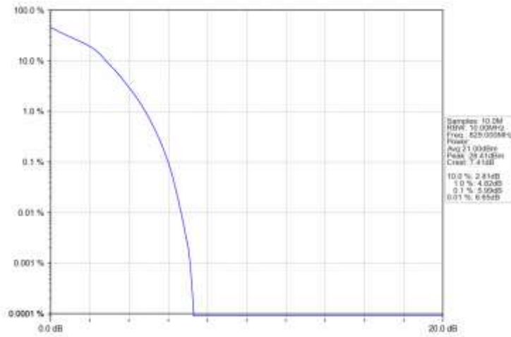
Band5_10MHz_16QAM_LCH_829MHz_RB_50_0_NTNV
