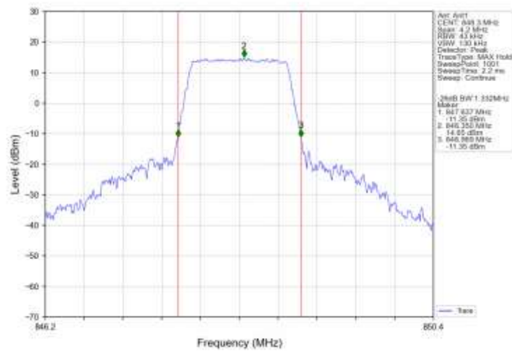
Band5 1.4MHz 16QAM HCH 848.3MHz RB 6 0 NTV
