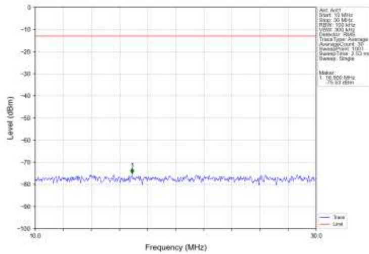
Band66_1.4MHz_QPSK_MCH_1745MHz_RB_1_0_NTNV
