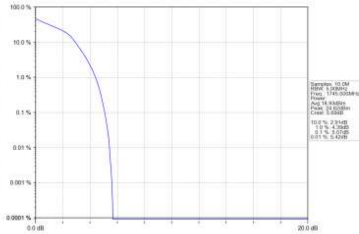
Band66_3MHz_16QAM_MCH_1745MHz_RB_15_0_NTNV
