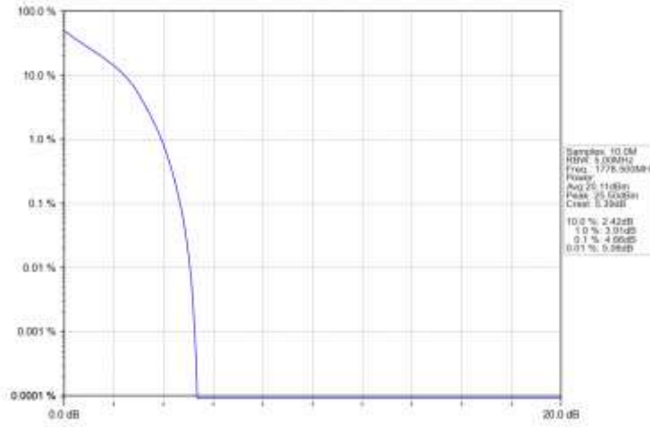
Band66 3MHz QPSK HCH 1778.5MHz RB 15 0 NTN
