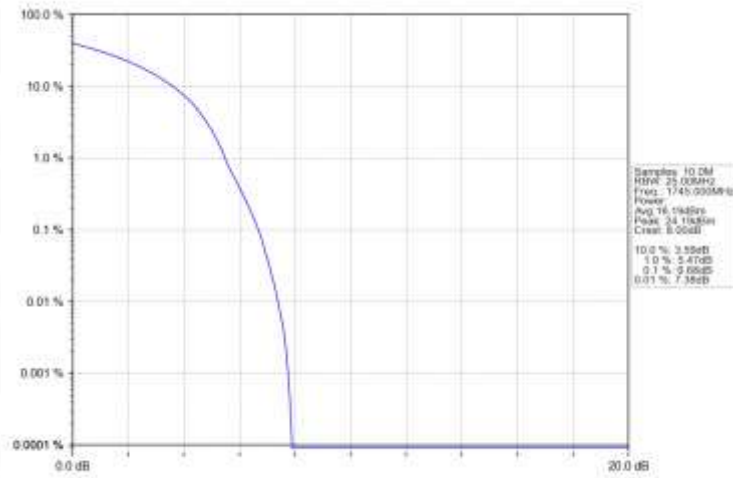
Band66_20MHz_16QAM_MCH_1745MHz_RB_100_0_NTNV
