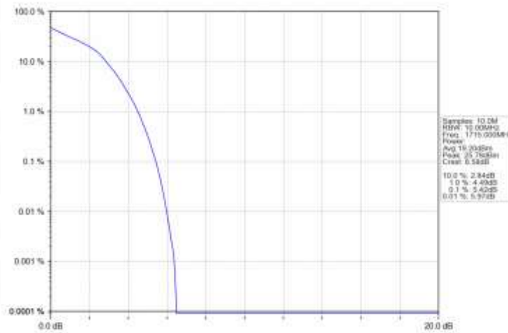
Band66_10MHz_16QAM_LCH_1715MHz_RB_50_0_NTNV
