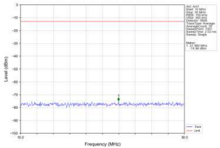
Band66_10MHz_QPSK_MCH_1745MHz_RB_1_0_NTNV
