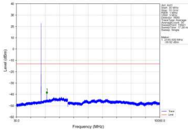
Band66_3MHz_16QAM_MCH_1745MHz_RB_1_0_NTNV
