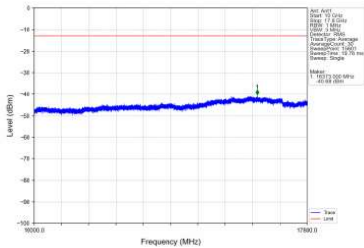
Band66_20MHz_QPSK_MCH_1745MHz_RB_1_0_NTV
