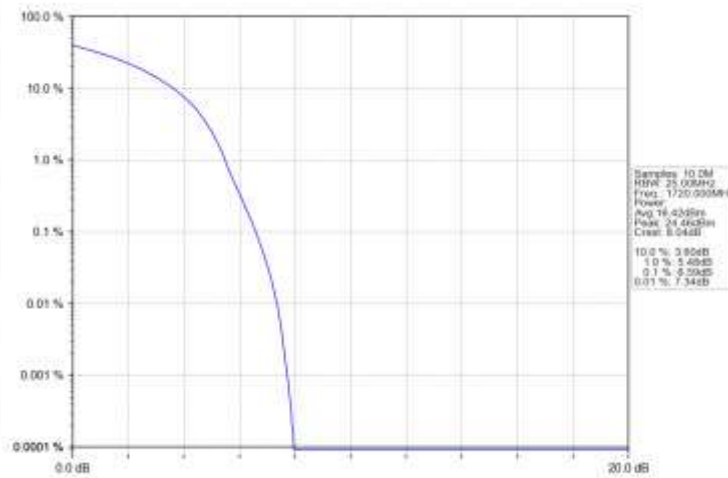
Band66_20MHz_16QAM_LCH_1720MHz_RB_100_0_NTN
