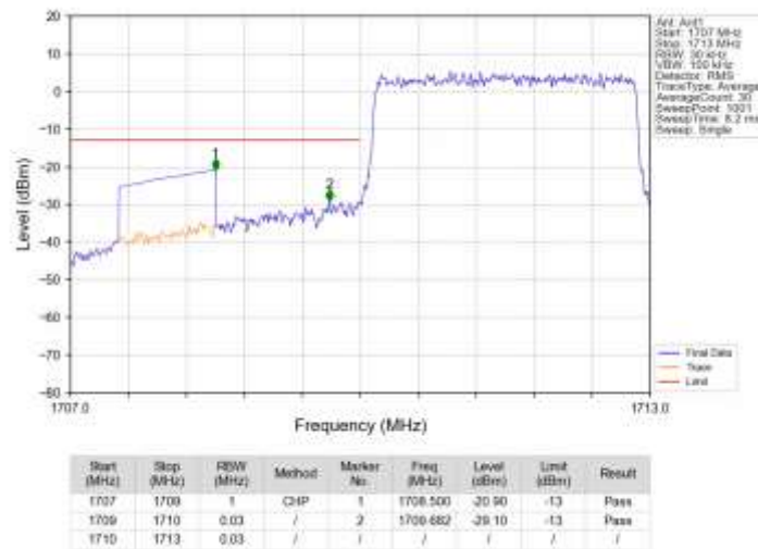
Band66_3MHz_16QAM_LCH_1711.5MHz_RB_15_0_NTNV
