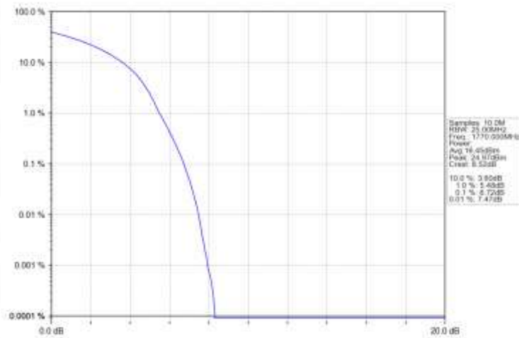
Band66_20MHz_16QAM_HCH_1770MHz_RB_100_0_NTNV
