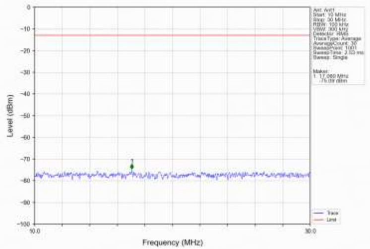
Band66_5MHz_QPSK_LCH_1712.5MHz_RB_1_0_NTNV
