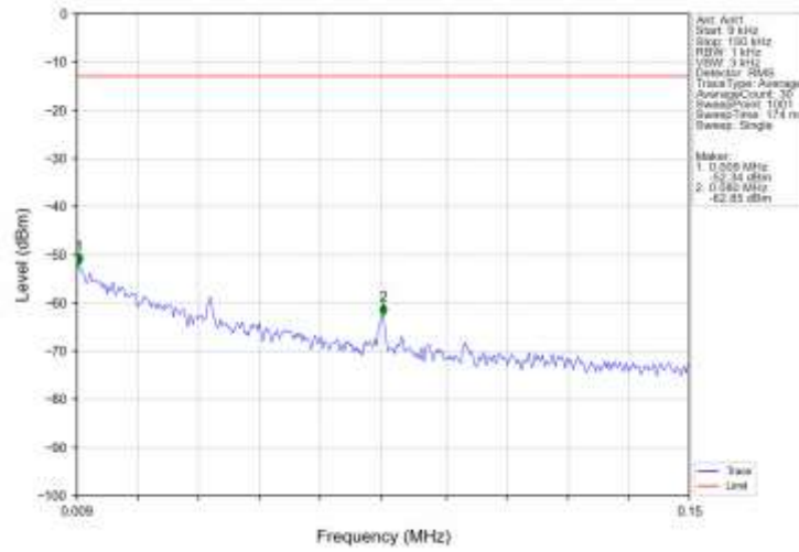
Band66 15MHz 16QAM LCH 1717.5MHz RB 1 0 NTNV
