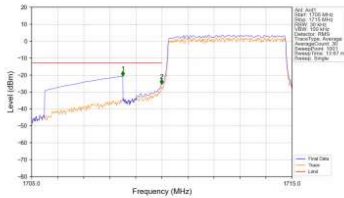
Band66_5MHz_16QAM_LCH_1712.5MHz_RB_25_0_NTNV
