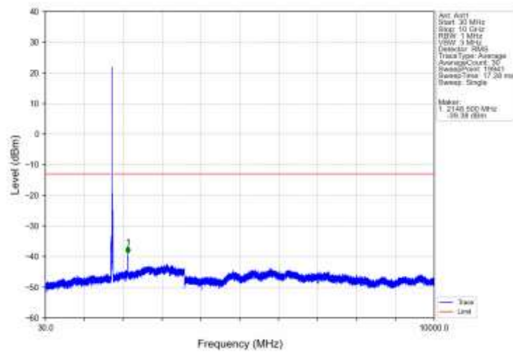
Band66_15MHz_16QAM_MCH_1745MHz_RB_1_0_NTNV
