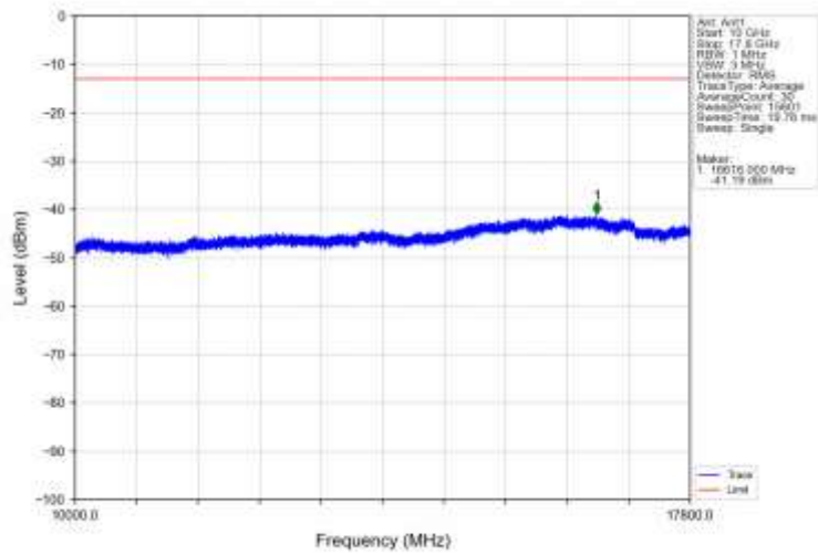
Band66_5MHz_16QAM_HCH_1777.5MHz_RB_1_0_NTNV
