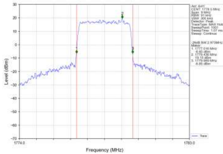
Band66_3MHz_16QAM_HCH_1778.5MHz_RB_15_0_NTNV
