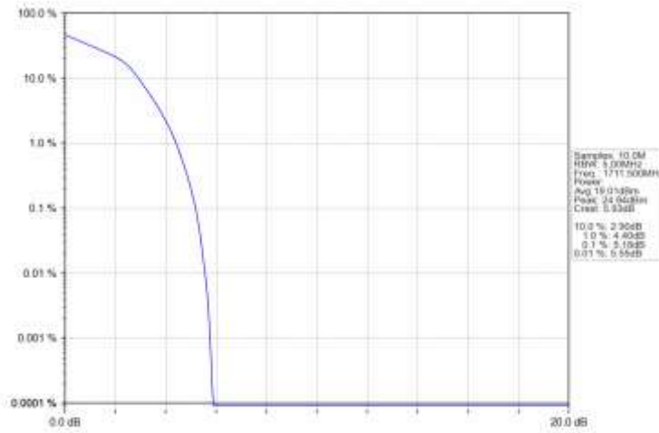
Band66 3MHz 16QAM LCH 1711.5MHz RB 15 0 NTN
