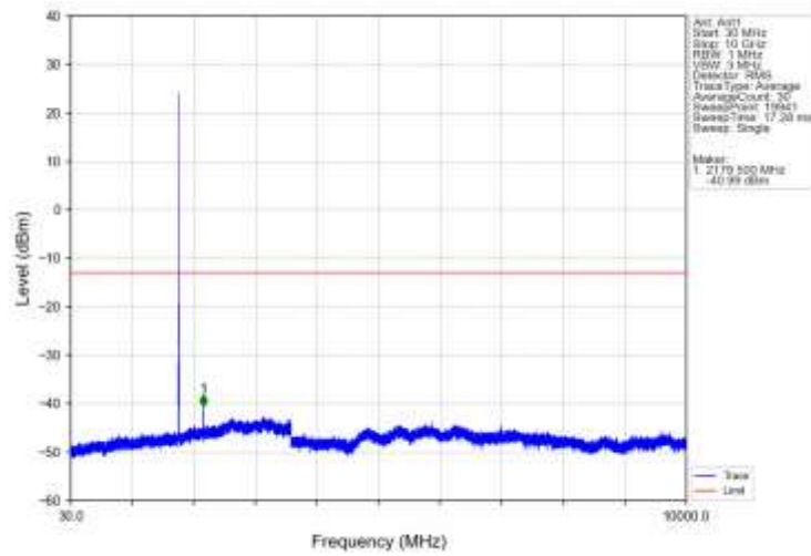
Band66_3MHz_QPSK_HCH_1778.5MHz_RB_1_0_NTV
