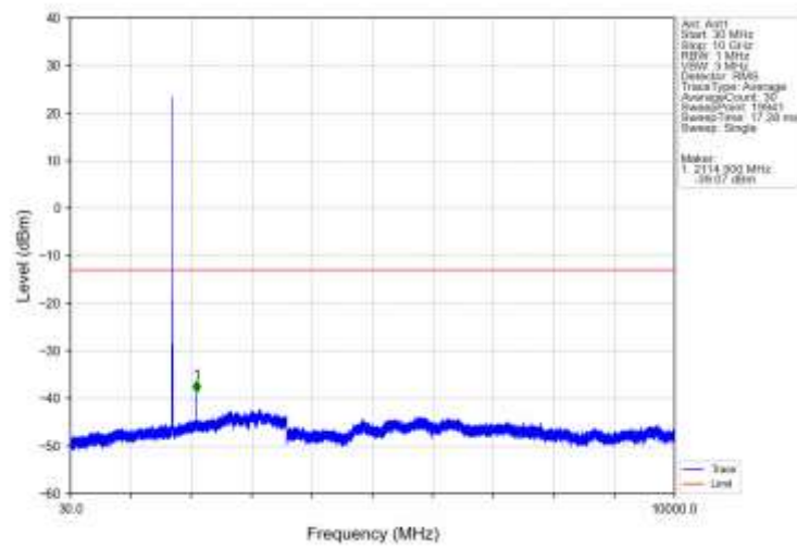
Band66_5MHz_16QAM_LCH_1712.5MHz_RB_1_0_NTNV
