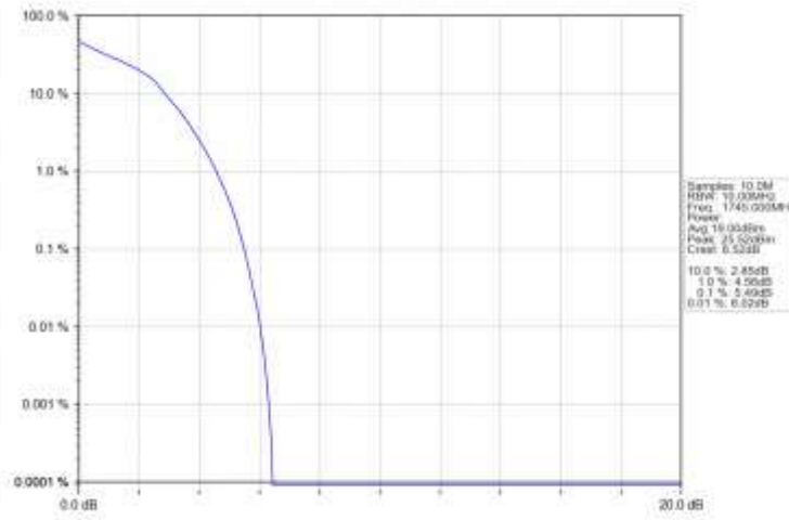
Band66 10MHz 16QAM MCH 1745MHz RB 50 0 NTN
