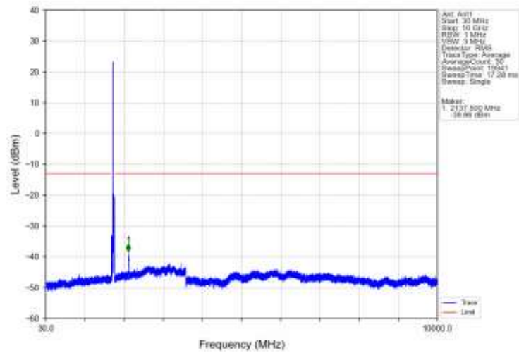
Band66_20MHz_QPSK_MCH_1745MHz_RB_1_0_NTV
