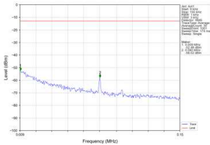
Band66_5MHz_16QAM_HCH_1777.5MHz_RB_1_0_NTNV
