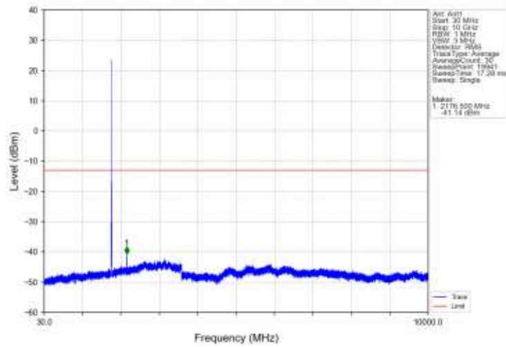
Band66_5MHz_QPSK_HCH_1777.5MHz_RB_1_0_NTNV
