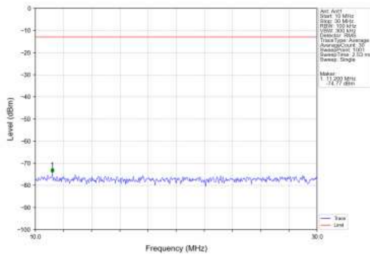
Band66_15MHz_QPSK_MCH_1745MHz_RB_1_0_NTNV
