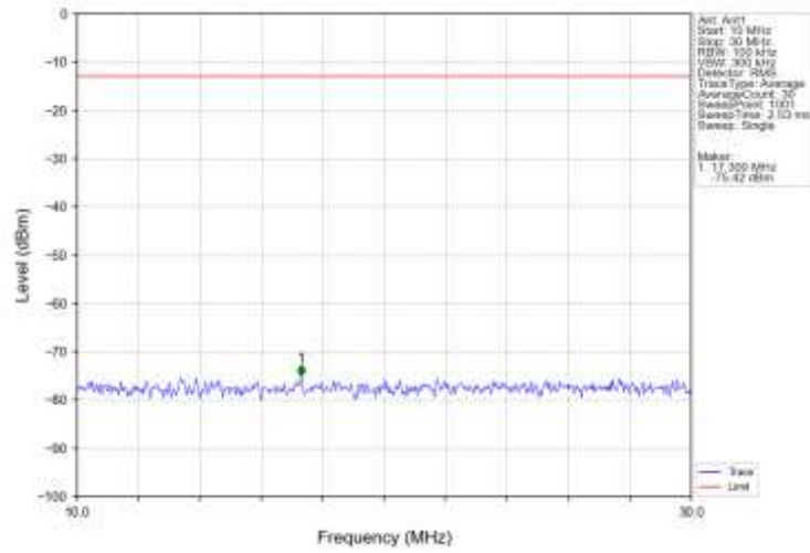
Band66_3MHz_QPSK_HCH_1778.5MHz_RB_1_0_NTV
