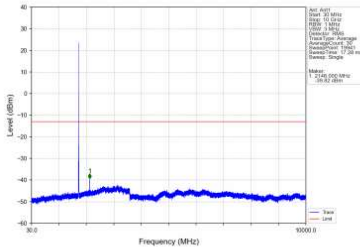
Band66_5MHz_16QAM_MCH_1745MHz_RB_1_0_NTNV
