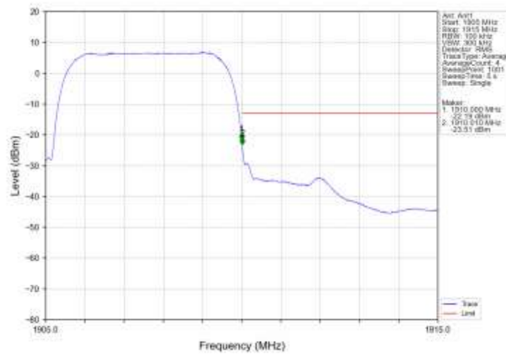
Band2_RMC_HCH_1907.6MHz_12.2kbps_RMC_NTNV
