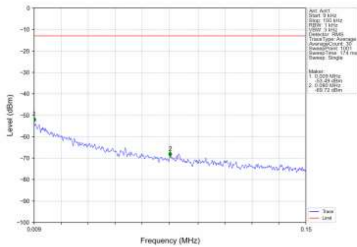
Band2_HSUPA_LCH_1852.4MHz_Subtest 1_NTNV
