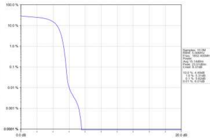
Band2_HSDPA_LCH_1852.4MHz_Subtest 1_NTNV
