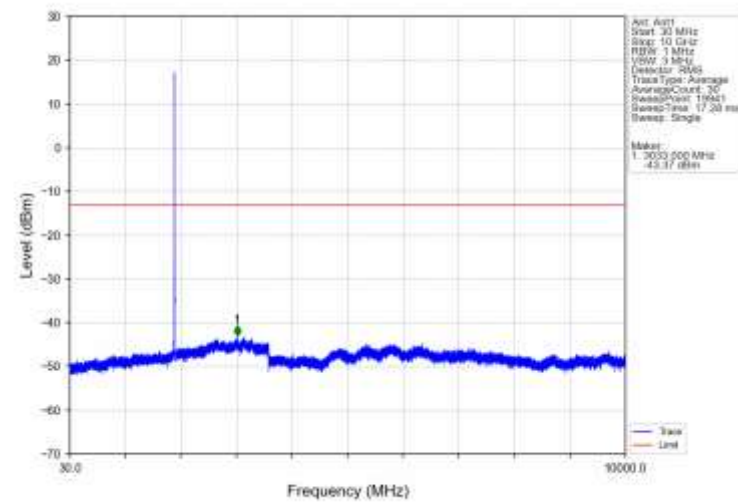
Band2_RMC_HCH_1907.6MHz_12.2kbps_RMC_NTNV
