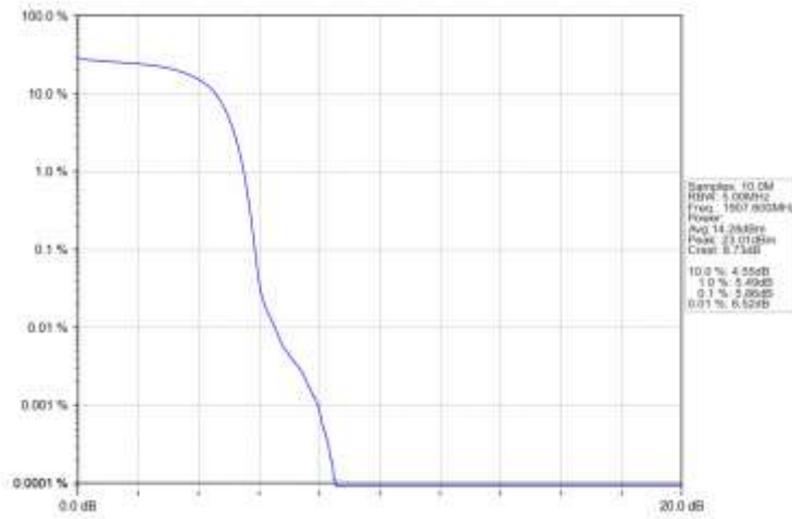
Band2_HSDPA_HCH_1907.6MHz_Subtest 1_NTNV
