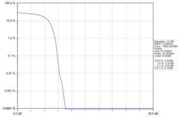
Band2_HSDPA_MCH_1880MHz_Subtest 1_NTNV
