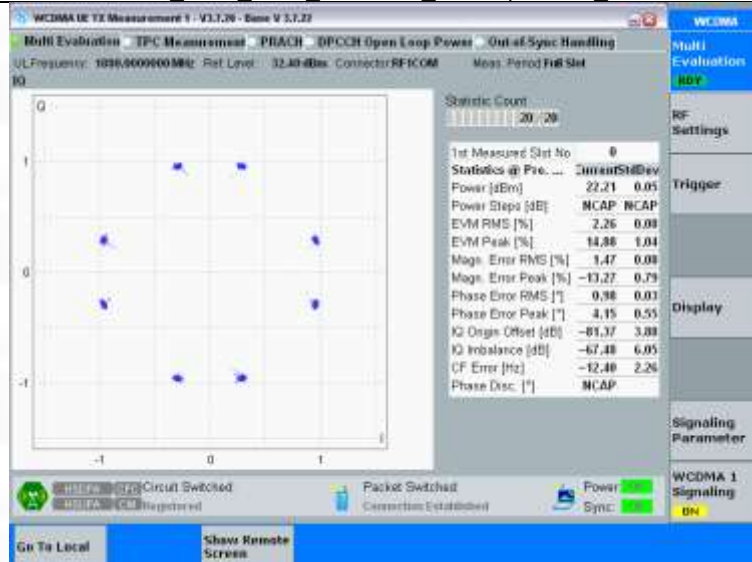
Band2_HSDPA_MCH_1880MHz_Subtest 1_NTNV
