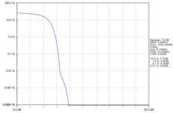
Band2_HSUPA_LCH_1852.4MHz_Subtest 1_NTNV
