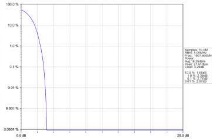
Band2_RMC_HCH_1907.6MHz_12.2kbps_RMC_NTNV
