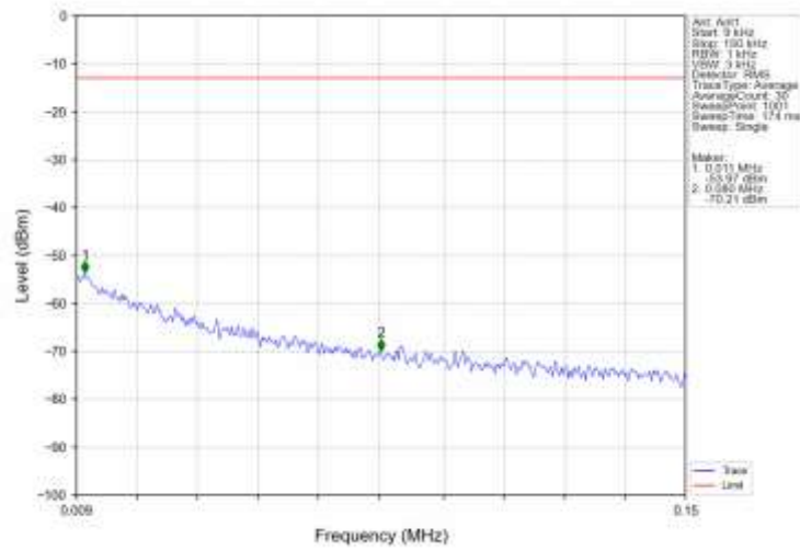
Band2_HSDPA_MCH_1880MHz_Subtest 1_NTNV
