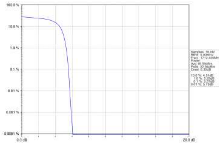
Band4_HSDPA_LCH_1712.4MHz_Subtest 1_NTNV
