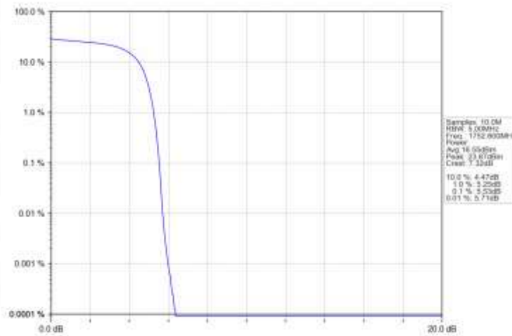
Band4_HSDPA_HCH_1752.6MHz_Subtest 1_NTNV
