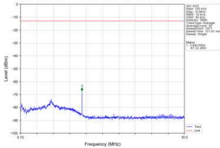
Band4_RMC_MCH_1732.6MHz_12.2kbps_RMC_NTNV
