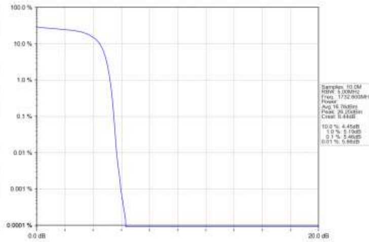
Band4_HSDPA_MCH_1732.6MHz_Subtest 1_NTNV
