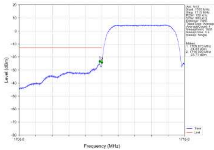
Band4_HSDPA_LCH_1712.4MHz_Subtest 1_NTNV
