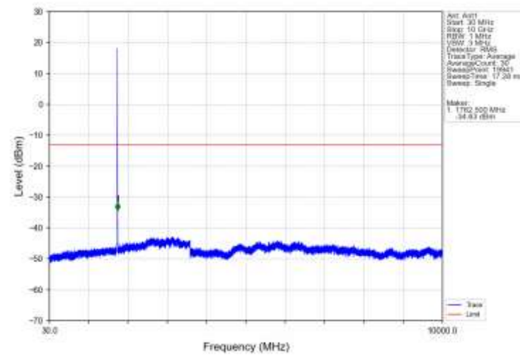
Band4_RMC_HCH_1752.6MHz_12.2kbps_RMC_NTNV
