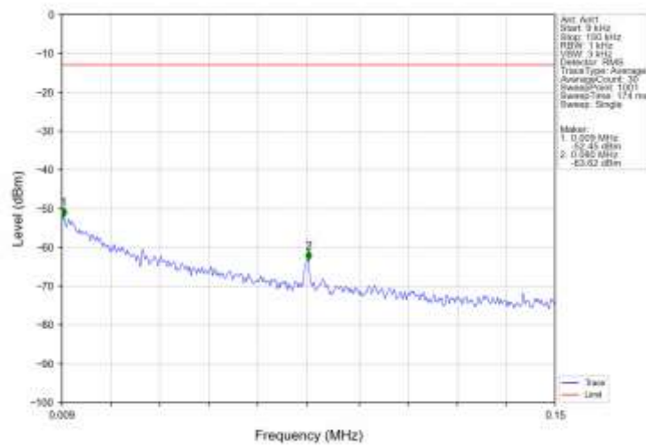
Band4_HSDPA_HCH_1752.6MHz_Subtest 1_NTNV
