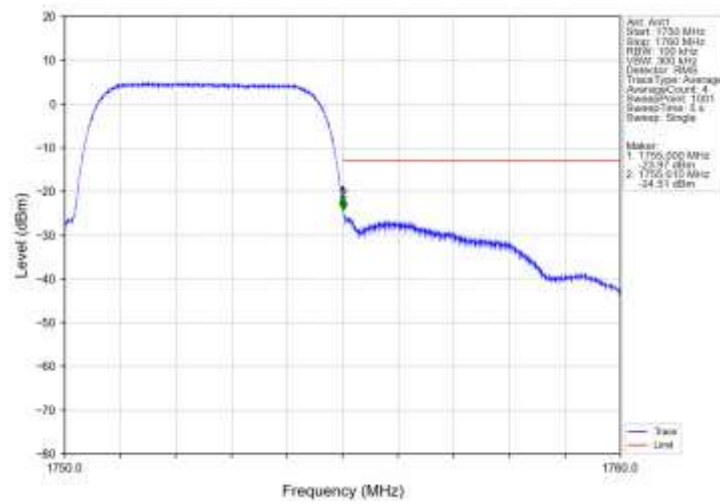
Band4_HSUPA_HCH_1752.6MHz_Subtest 1_NTNV
