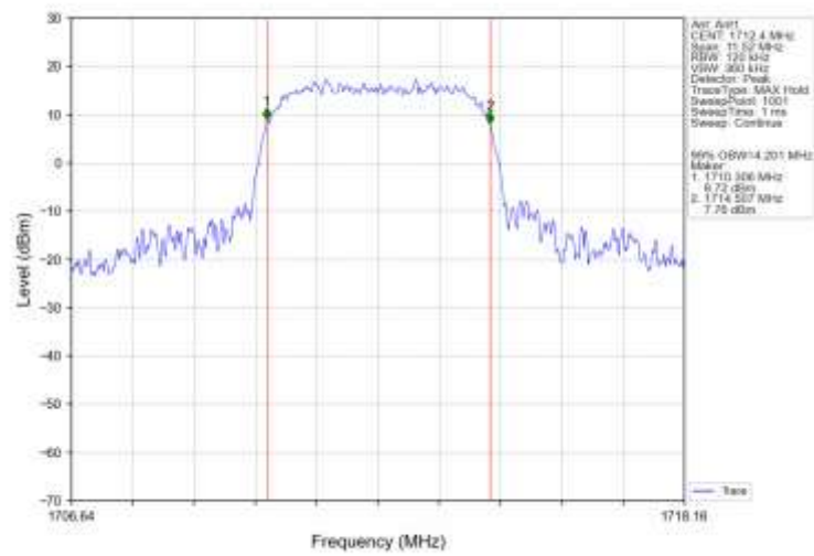
Band4_HSDPA_LCH_1712.4MHz_Subtest 1_NTNV
