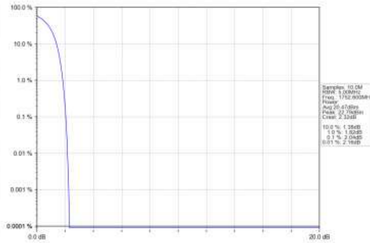
Band4_RMC_HCH_1752.6MHz_12.2kbps_RMC_NTNV
