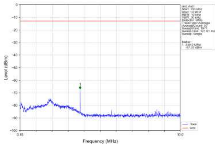
Band4_RMC_HCH_1752.6MHz_12.2kbps_RMC_NTNV
