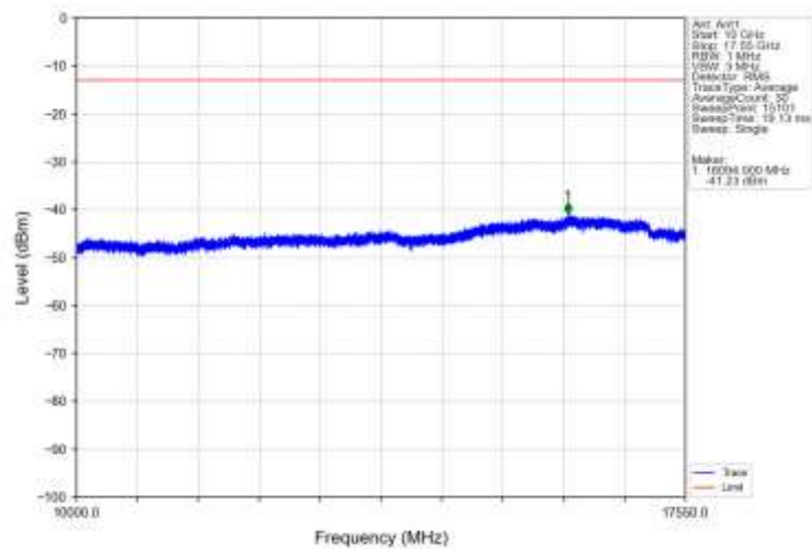
Band4_HSDPA_HCH_1752.6MHz_Subtest 1_NTNV
