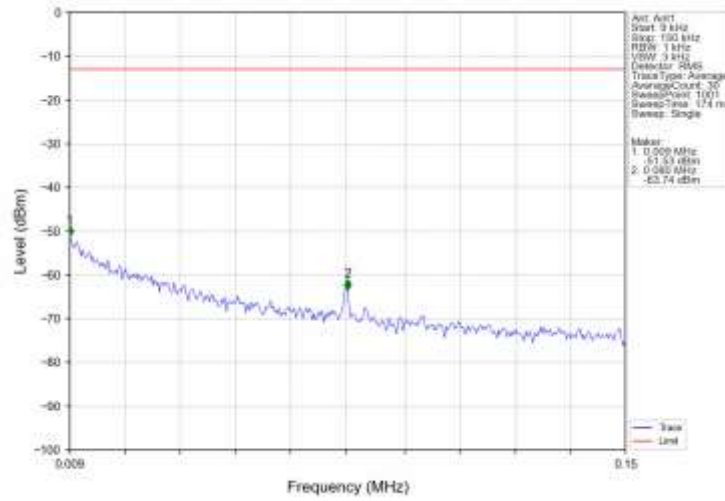
Band4_RMC_MCH_1732.6MHz_12.2kbps_RMC_NTNV
