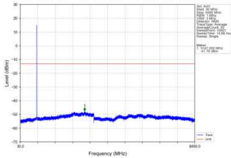
Band5_RMC_MCH_836.6MHz_12.2kbps_RMC_NTNV
