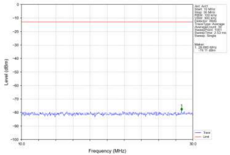
Band5_RMC_MCH_836.6MHz_12.2kbps_RMC_NTNV
