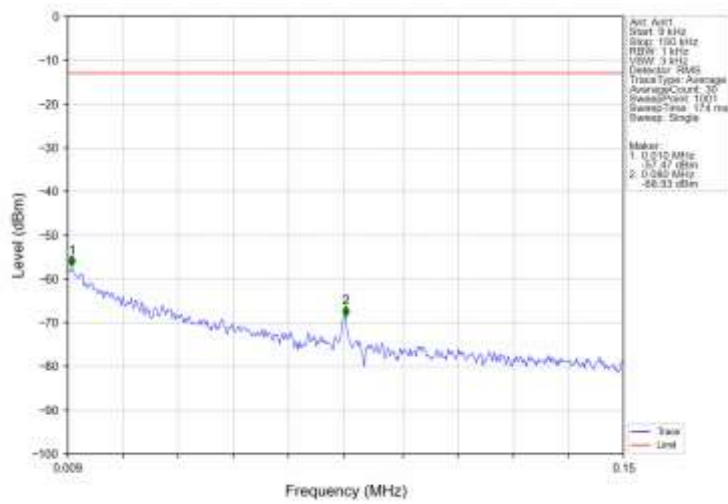
Band5_HSDPA_MCH_836.6MHz_Subtest 1_NTNV
