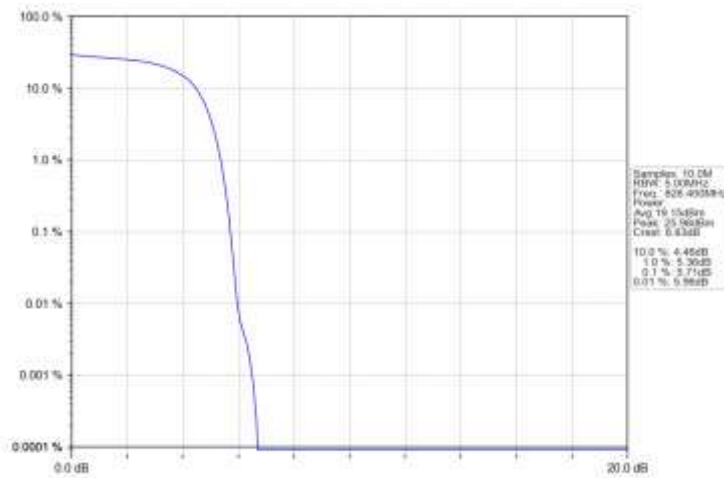
Band5_HSDPA_LCH_826.4MHz_Subtest 1_NTNV
