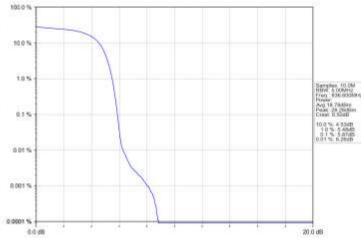
Band5_HSDPA_MCH_836.6MHz_Subtest 1_NTNV
