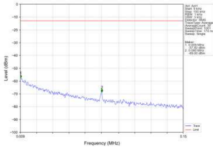
Band5_HSUPA_LCH_826.4MHz_Subtest 1_NTNV
