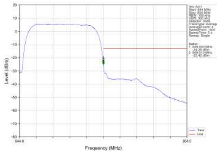
Band5_RMC_HCH_846.6MHz_12.2kbps_RMC_NTNV
