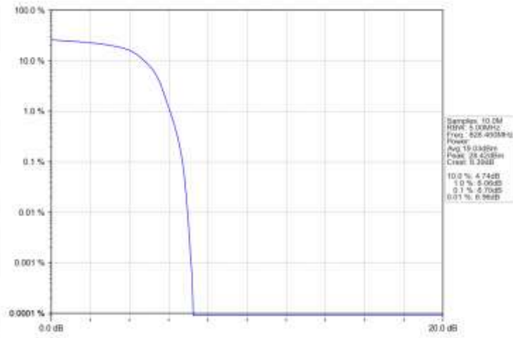
Band5_HSUPA_LCH_826.4MHz_Subtest 1_NTNV
