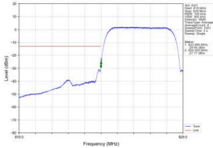
Band5_HSUPA_LCH_826.4MHz_Subtest 1_NTNV
