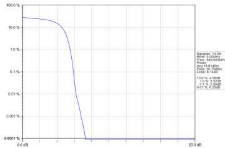
Band5_HSDPA_HCH_846.6MHz_Subtest 1_NTNV
