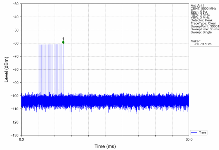
Signal Calibration_802.11a_2C_5500MHz_RadarType3_Trial0
