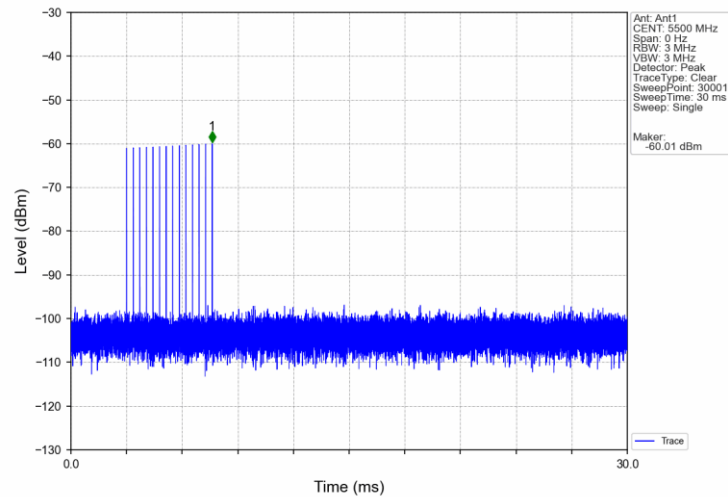
Signal Calibration_802.11a_2C_5500MHz_RadarType5_Trial0
