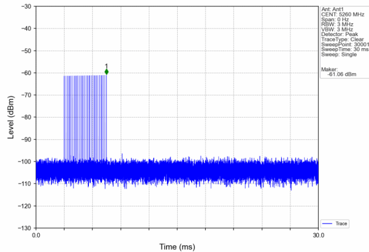
Signal Calibration_802.11a_2A_5260MHz_RadarType3_Trial0
