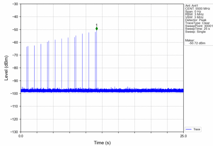
Signal Calibration_802.11a_2C_5500MHz_RadarType5_Trial0
