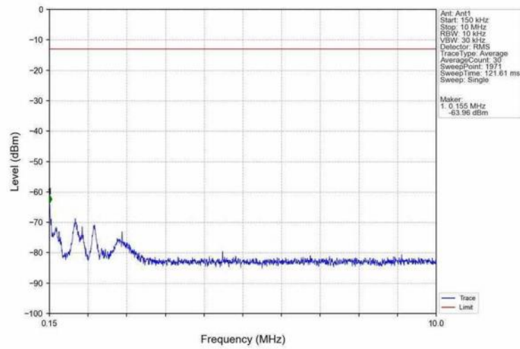
Band25_3MHz_QPSK_HCH_1913.5MHz_RB_1_0_NTNV
