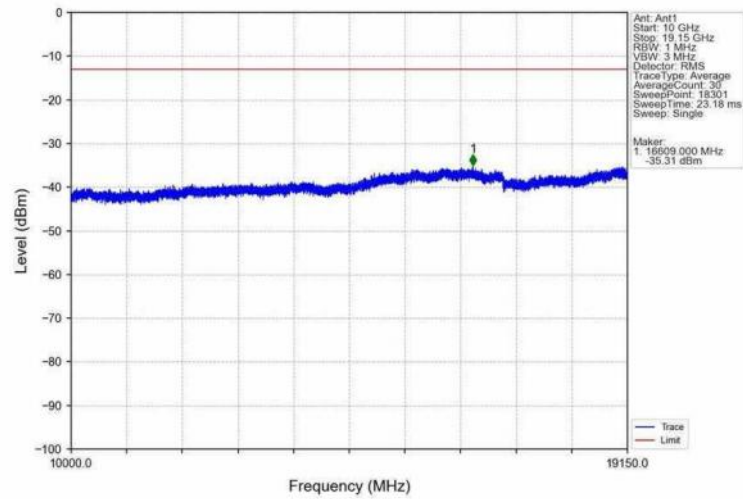
Band25_10MHz_16QAM_HCH_1910MHz_RB_1_0_NTNV
