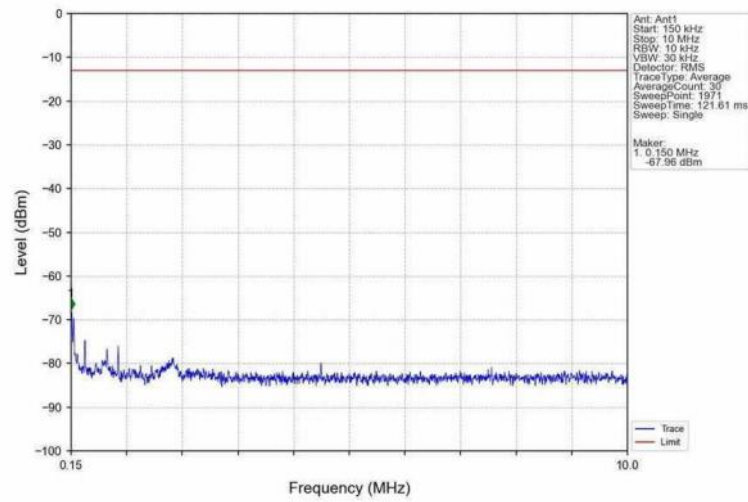
Band25_20MHz_16QAM_LCH_1860MHz_RB_1_0_NTNV
