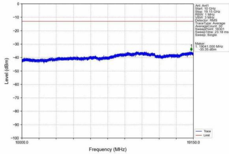
Band25_3MHz_16QAM_HCH_1913.5MHz_RB_1_0_NTNV
