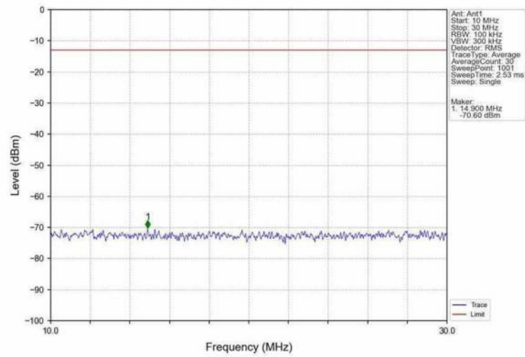
Band25_5MHz_QPSK_MCH_1882.5MHz_RB_1_0_NTNV
