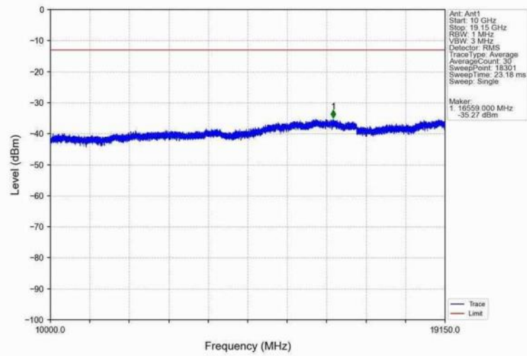
Band25_5MHz_QPSK_LCH_1852.5MHz_RB_1_0_NTNV
