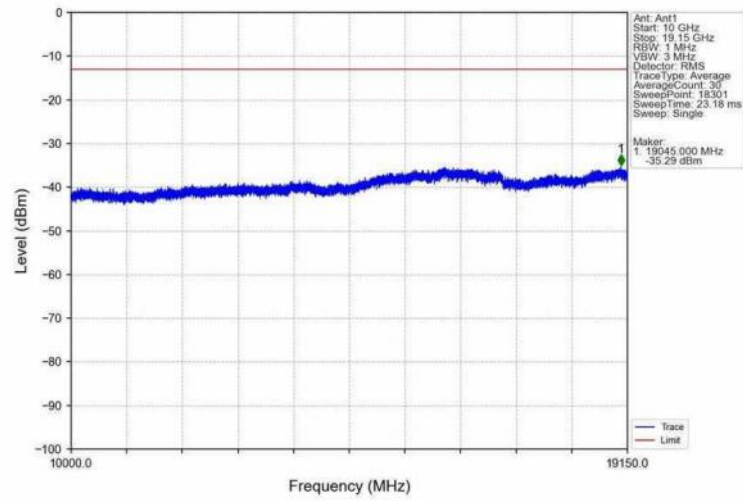
Band25_5MHz_16QAM_HCH_1912.5MHz_RB_1_0_NTNV
