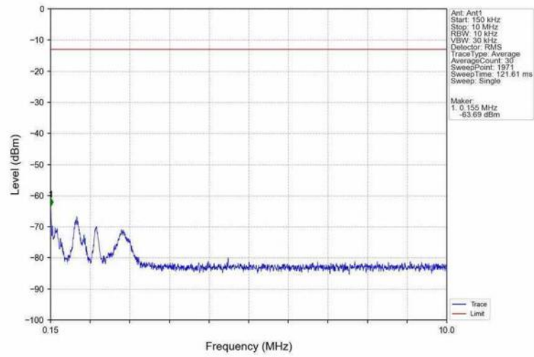
Band25_3MHz_QPSK_MCH_1882.5MHz_RB_1_0_NTNV
