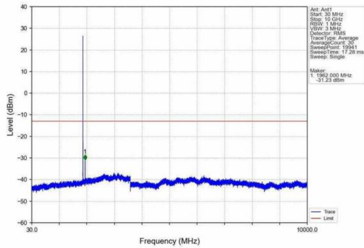
Band25_3MHz_16QAM_MCH_1882.5MHz_RB_1_0_NTNV
