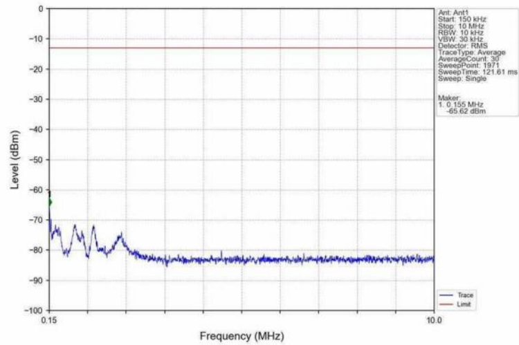
Band25_5MHz_QPSK_LCH_1852.5MHz_RB_1_0_NTNV
