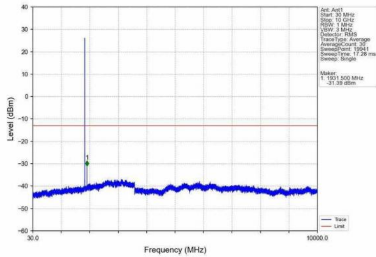
Band25_3MHz_16QAM_LCH_1851.5MHz_RB_1_0_NTNV
