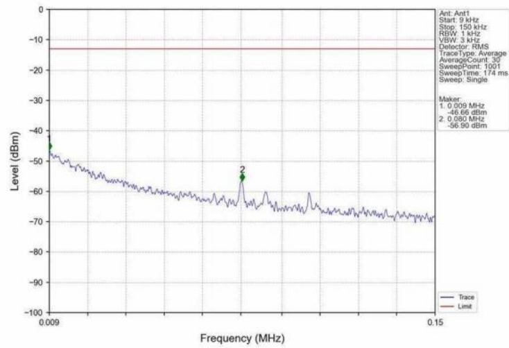
Band25_3MHz_16QAM_HCH_1913.5MHz_RB_1_0_NTNV
