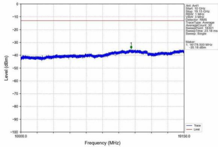
Band25_3MHz_QPSK_MCH_1882.5MHz_RB_1_0_NTNV
