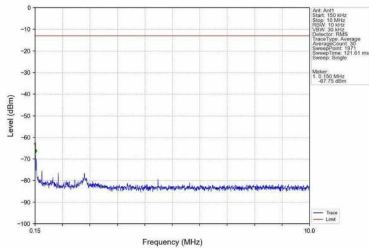
Band25_10MHz_16QAM_LCH_1855MHz_RB_1_0_NTNV
