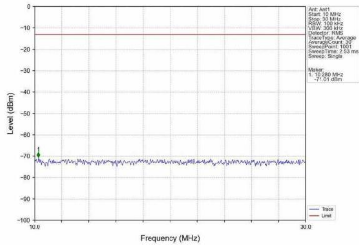
Band25_3MHz_QPSK_MCH_1882.5MHz_RB_1_0_NTNV
