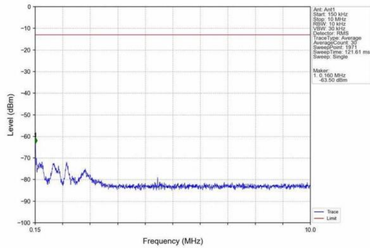
Band25_5MHz_QPSK_HCH_1912.5MHz_RB_1_0_NTNV
