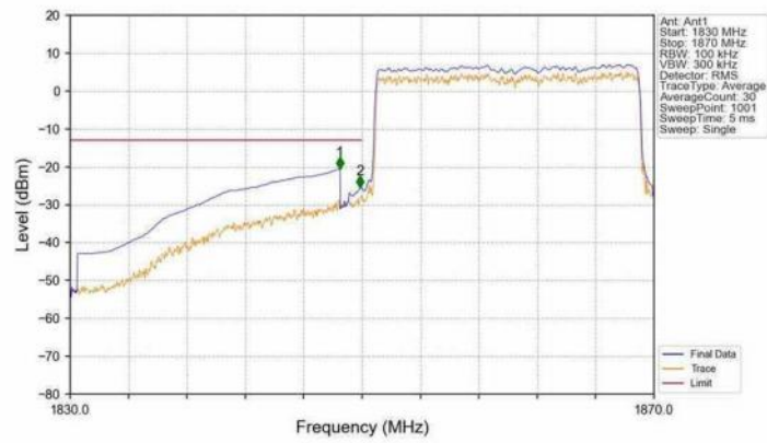
Band25_20MHz_16QAM_LCH_1860MHz_RB_100_0_NTNV
