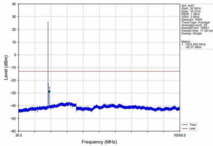
Band25_10MHz_16QAM_LCH_1855MHz_RB_1_0_NTNV
