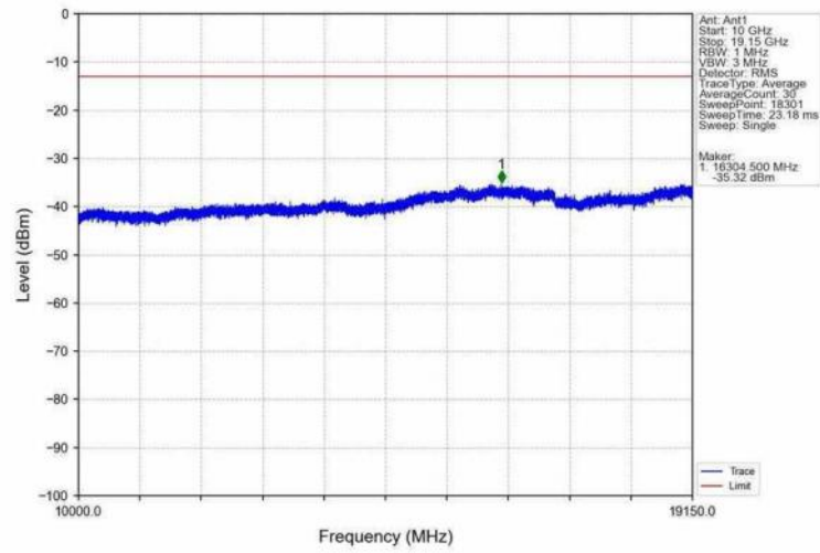
Band25_20MHz_16QAM_HCH_1905MHz_RB_1_0_NTNV
