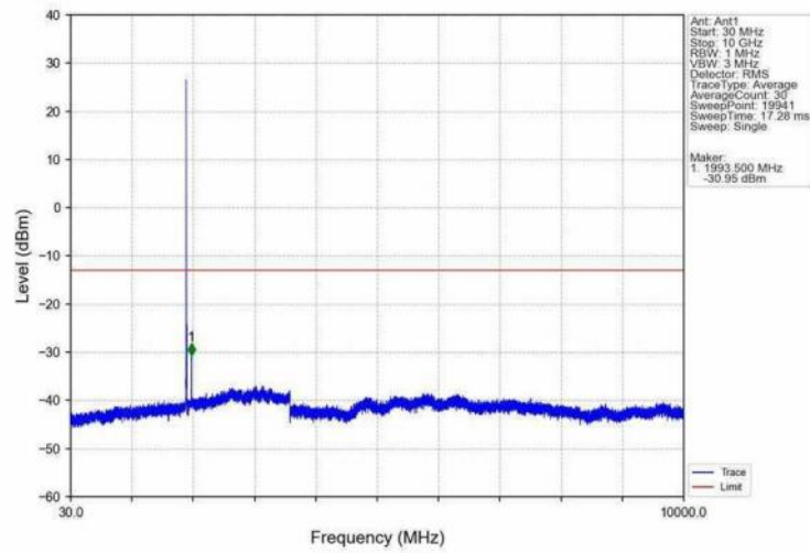
Band25_5MHz_QPSK_HCH_1912.5MHz_RB_1_0_NTNV
