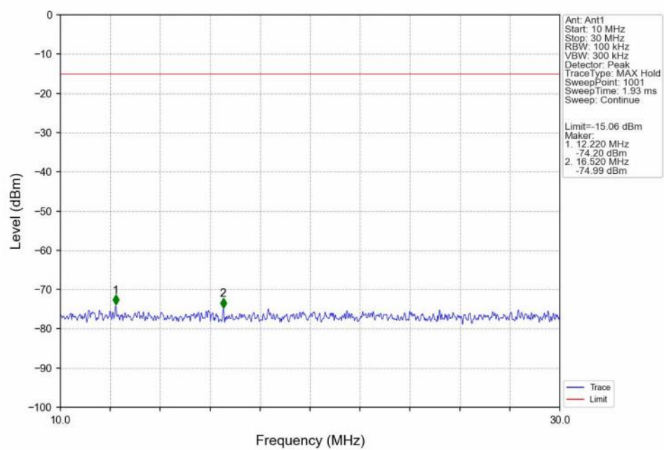
1M_LCH_2402MHz_Ant1_NTNV
