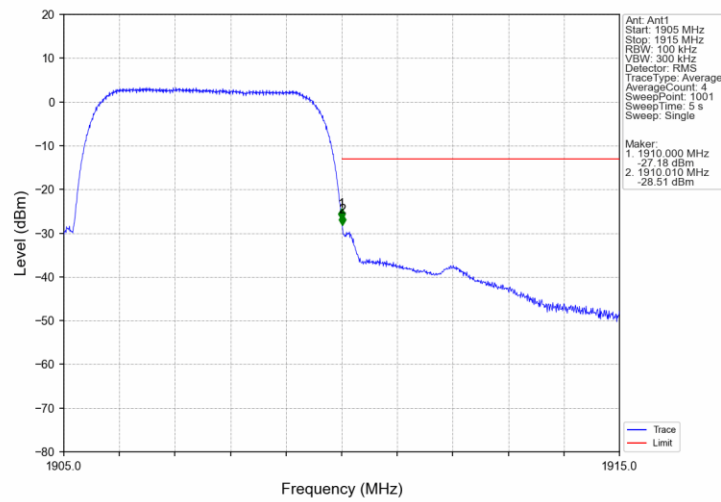
Band2_HSUPA_HCH_1907.6MHz_Subtest 1_NTNV
