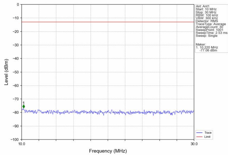
Band2_HSDPA_HCH_1907.6MHz_Subtest 1_NTNV
