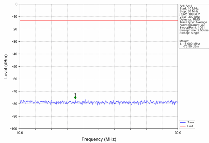
Band2_RMC_LCH_1852.4MHz_12.2kbps_RMC_NTNV
