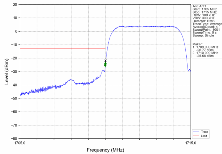
Band4_HSDPA_LCH_1712.4MHz_Subtest 1_NTNV
