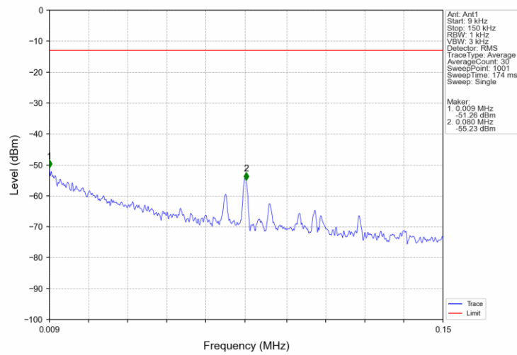
Band4_HSDPA_MCH_1732.6MHz_Subtest 1_NTNV
