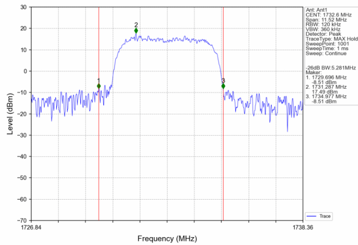
Band4 HSUPA MCH 1732.6MHz Subtest 1 NTN
