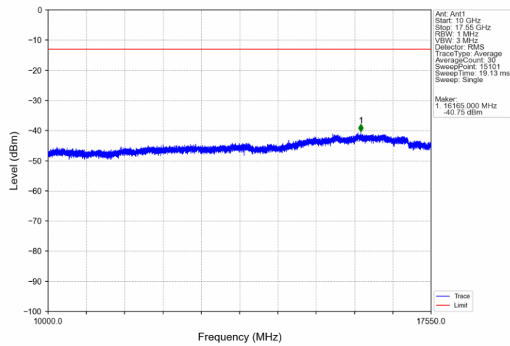
Band4_HSDPA_MCH_1732.6MHz_Subtest 1_NTNV
