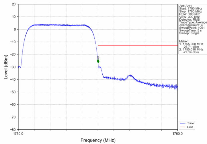
Band4_HSUPA_HCH_1752.6MHz_Subtest 1_NTNV
