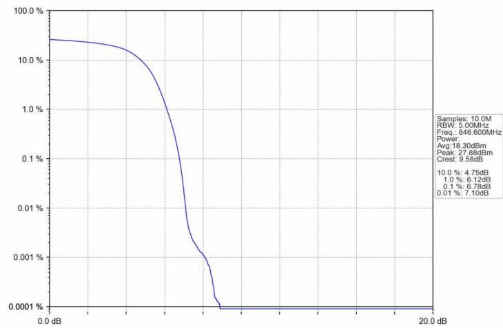
Band5_HSUPA_HCH_846.6MHz_Subtest 1_NTNV
