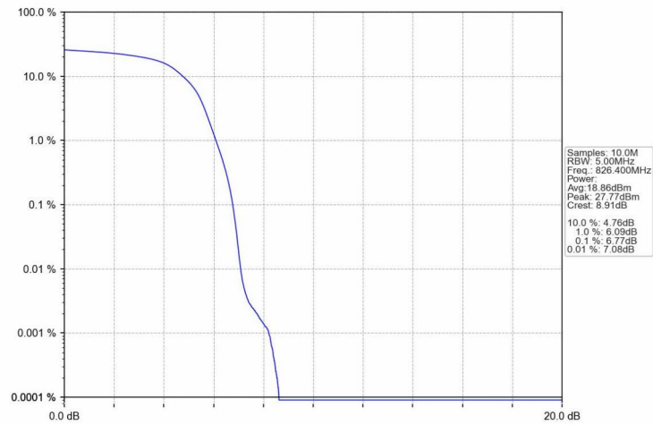
Band5_HSUPA_LCH_826.4MHz_Subtest 1_NTNV
