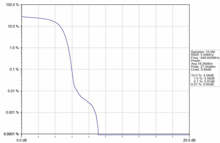
Band5_HSDPA_HCH_846.6MHz_Subtest 1_NTNV
