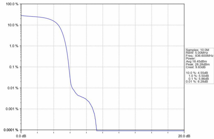
Band5_HSDPA_MCH_836.6MHz_Subtest 1_NTNV
