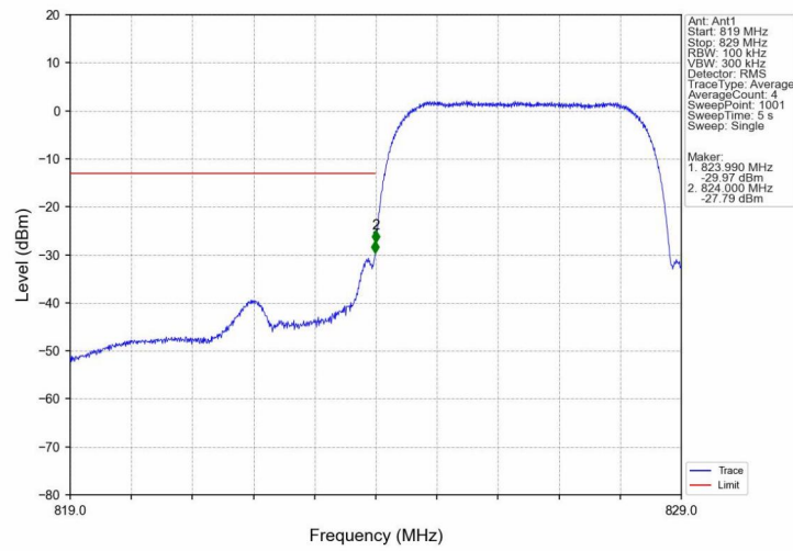
Band5_HSDPA_LCH_826.4MHz_Subtest 1_NTNV
