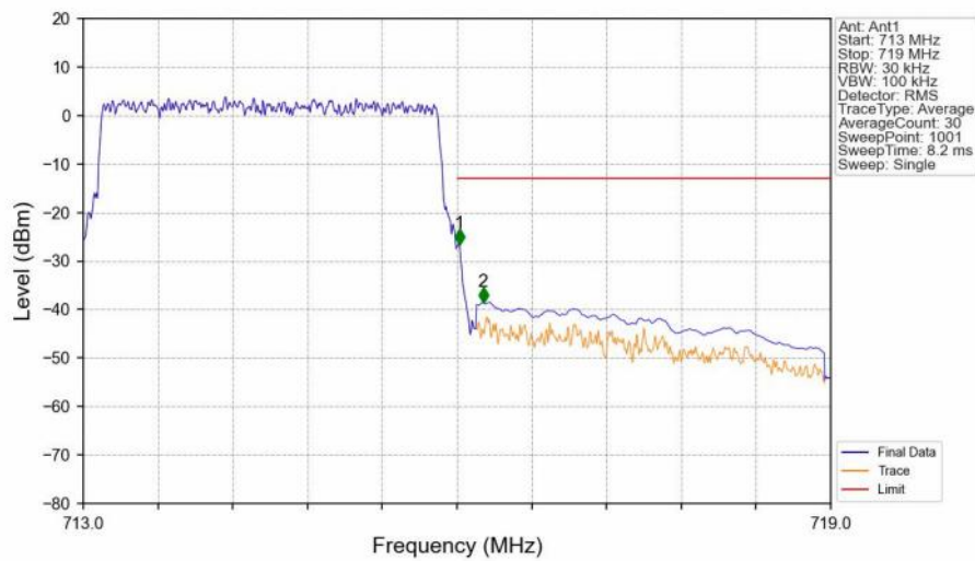
Band12_3MHz_16QAM_HCH_714.5MHz_RB_15_0_NTNV
