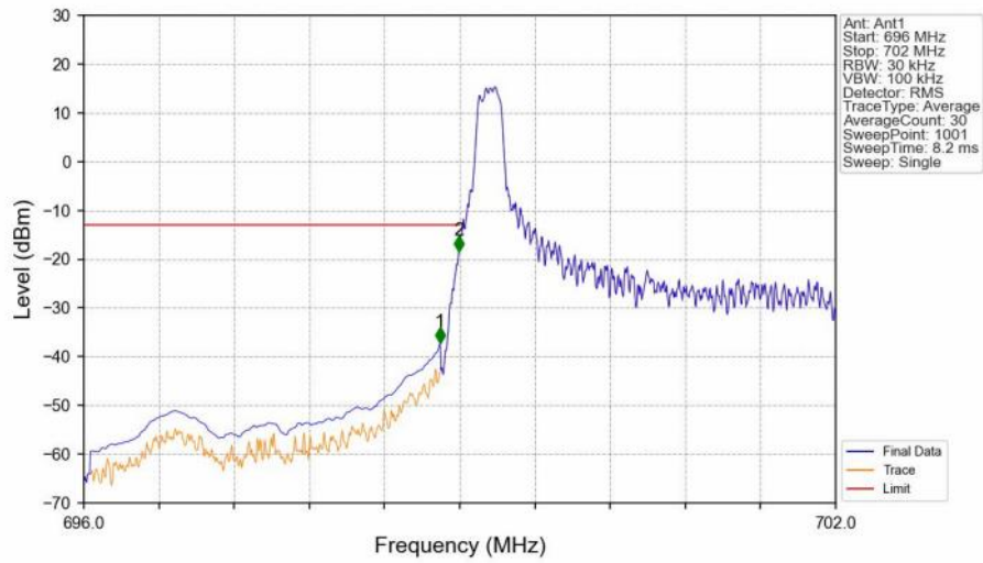
Band12_3MHz_16QAM_LCH_700.5MHz_RB_1_0_NTNV
