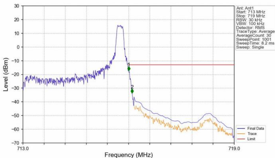
Band12_3MHz_QPSK_HCH_714.5MHz_RB_1_14_NTNV
