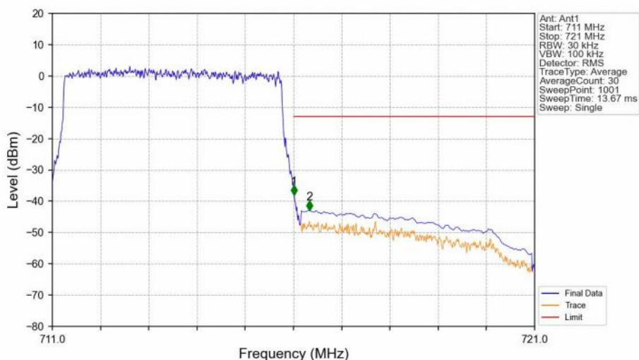
Band12_5MHz_QPSK_HCH_713.5MHz_RB_25_0_NTNV
