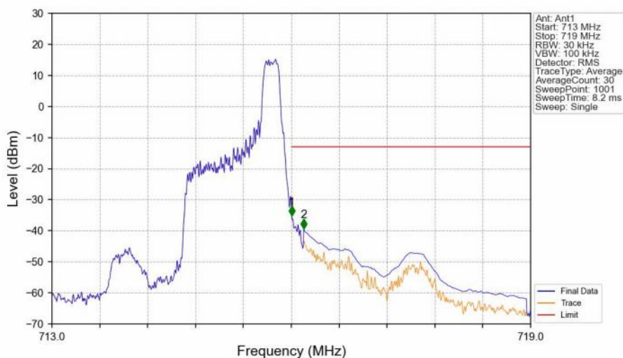
Band12_1.4MHz_16QAM_HCH_715.3MHz_RB_1_5_NTNV
