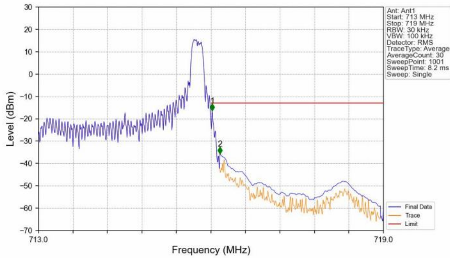
Band12_3MHz_16QAM_HCH_714.5MHz_RB_1_14_NTNV
