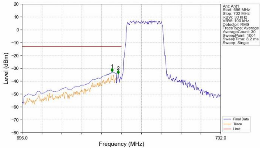
Band12_1.4MHz_16QAM_LCH_699.7MHz_RB_6_0_NTNV
