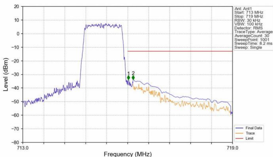
Band12_1.4MHz_16QAM_HCH_715.3MHz_RB_6_0_NTNV
