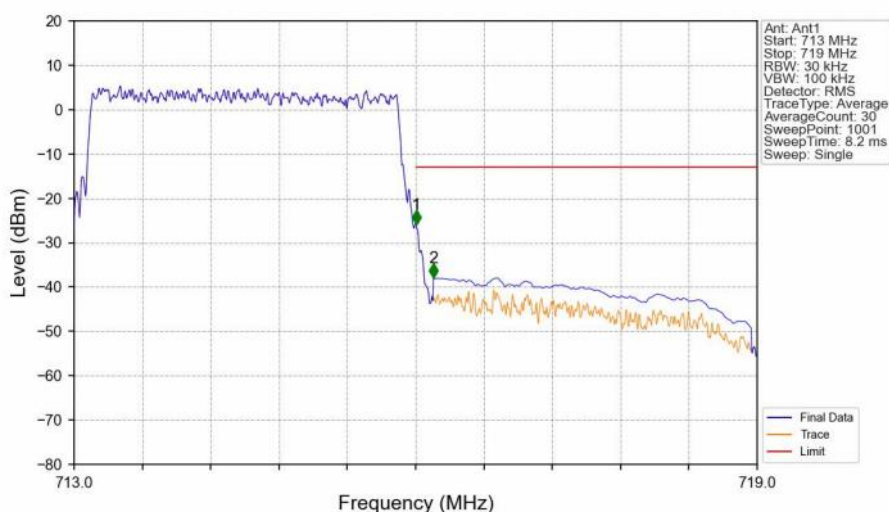
Band12_3MHz_QPSK_HCH_714.5MHz_RB_15_0_NTNV
