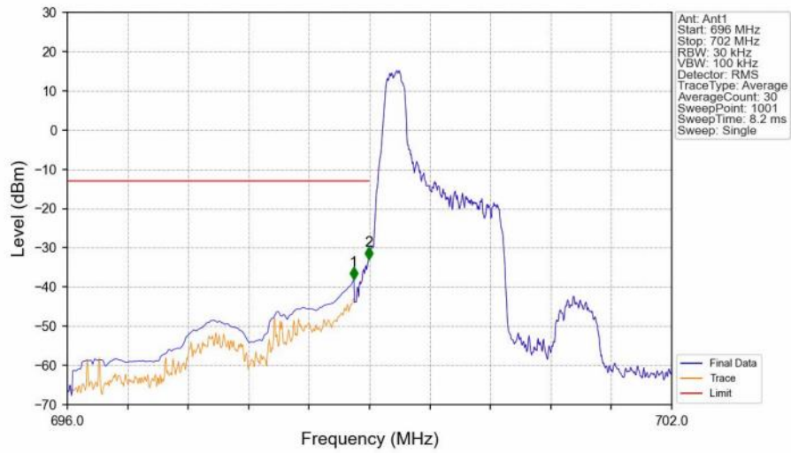
Band12_1.4MHz_16QAM_LCH_699.7MHz_RB_1_0_NTNV
