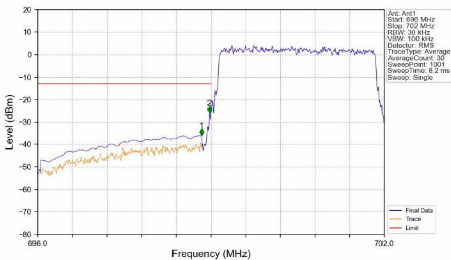
Band12_3MHz_16QAM_LCH_700.5MHz_RB_15_0_NTNV
