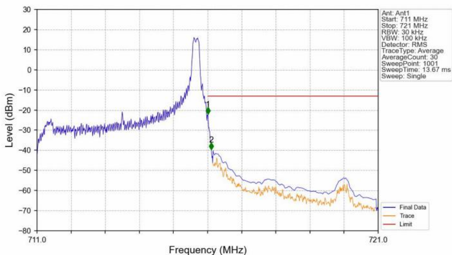
Band12_5MHz_QPSK_HCH_713.5MHz_RB_1_24_NTNV
