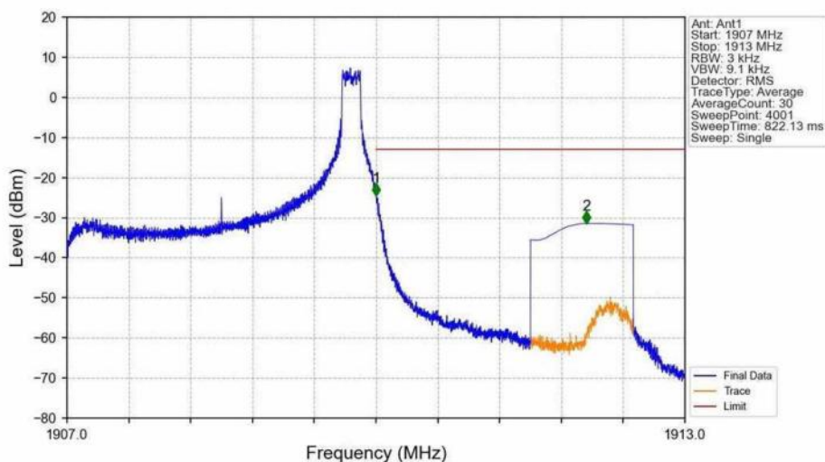
Band2_3MHz_16QAM_HCH_1908.5MHz_RB_1_14_NTNV
