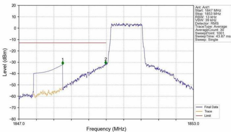
Band2_1.4MHz_16QAM_LCH_1850.7MHz_RB_6_0_NTNV
