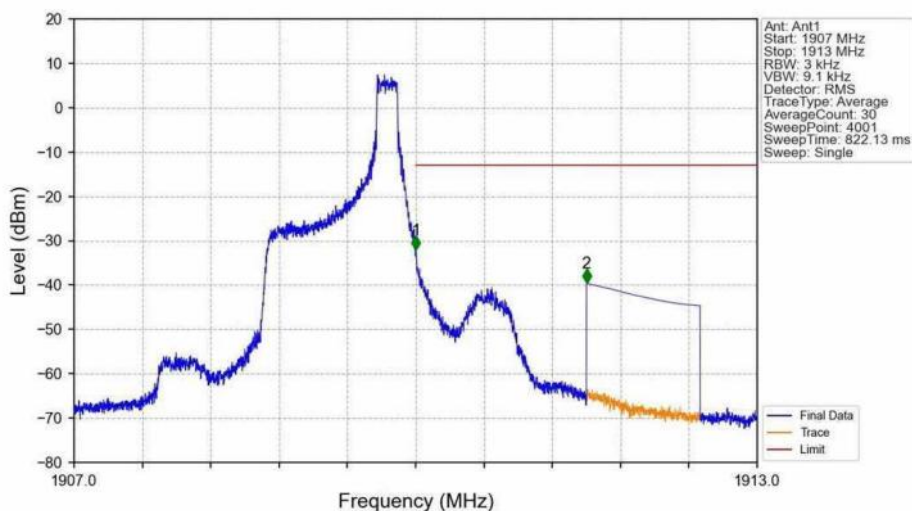
Band2_1.4MHz_16QAM_HCH_1909.3MHz_RB_1_5_NTNV
