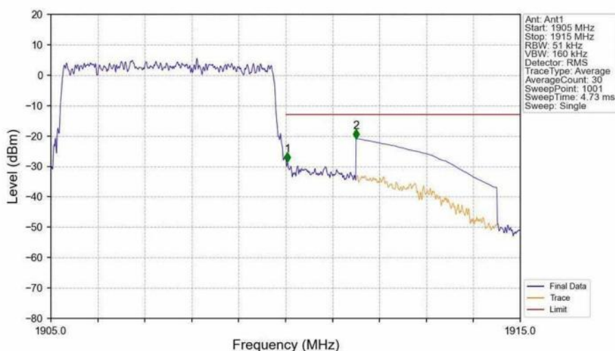
Band2_5MHz_16QAM_HCH_1907.5MHz_RB_25_0_NTNV
