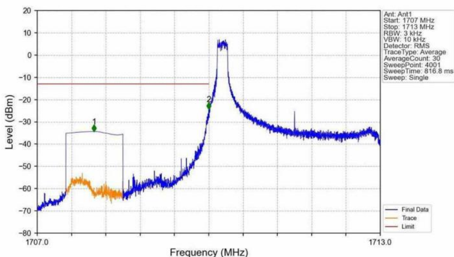
Band4_3MHz_16QAM_LCH_1711.5MHz_RB_1_0_NTNV
