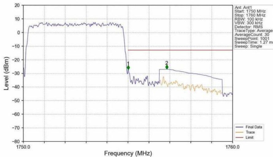
Band4_5MHz_16QAM_HCH_1752.5MHz_RB_25_0_NTNV
