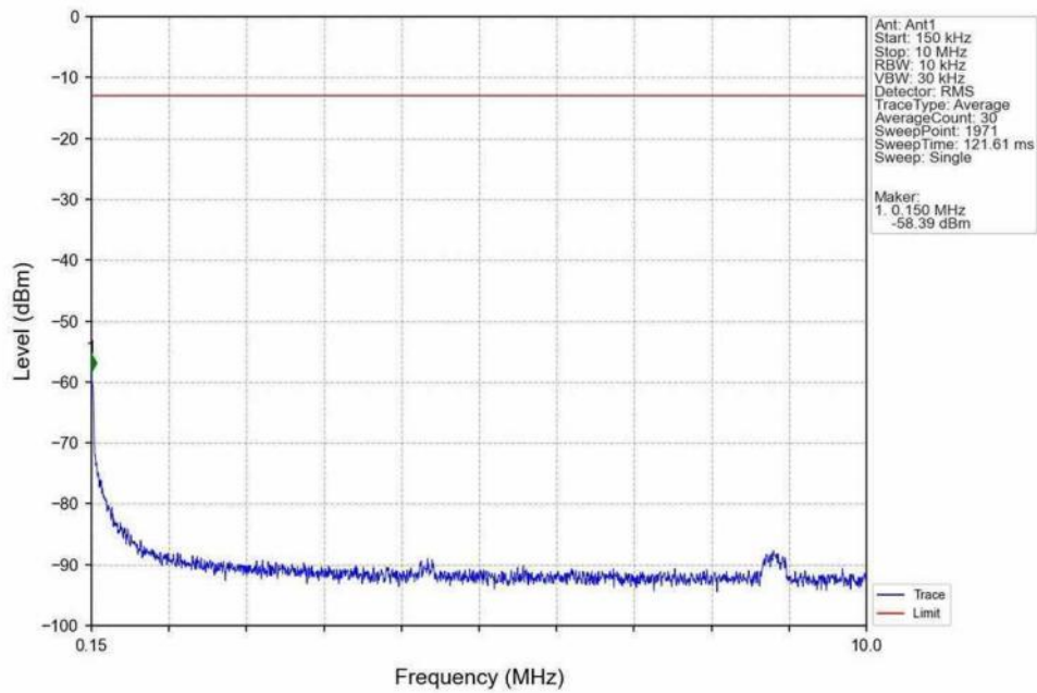
Band4_10MHz_16QAM_HCH_1750MHz_RB_1_0_NTNV
