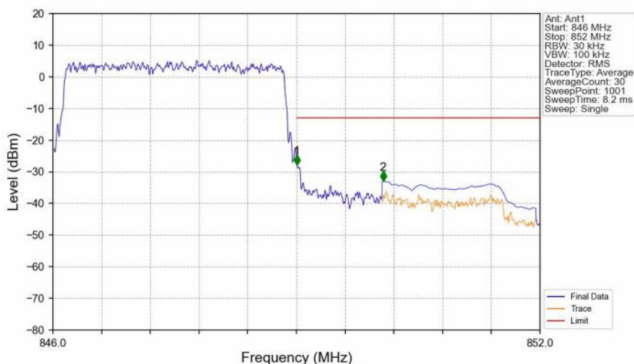
Band5_3MHz_QPSK_HCH_847.5MHz_RB_15_0_NTNV
