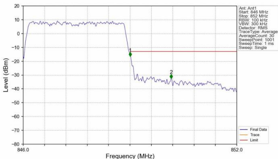
Band5_3MHz_16QAM_HCH_847.5MHz_RB_15_0_NTNV
