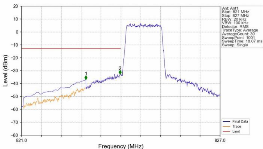
Band5_1.4MHz_16QAM_LCH_824.7MHz_RB_6_0_NTNV
