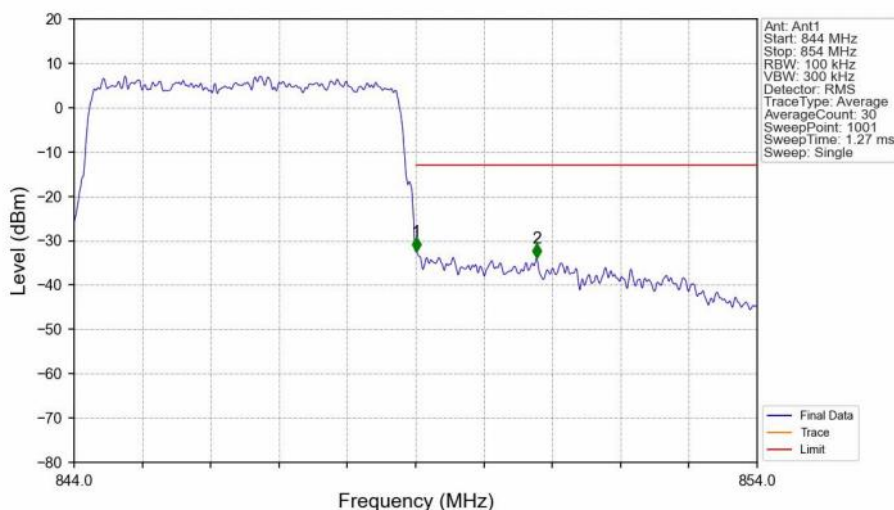
Band5_5MHz_16QAM_HCH_846.5MHz_RB_25_0_NTNV
