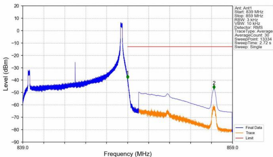
Band5_10MHz_16QAM_HCH_844MHz_RB_1_49_NTNV
