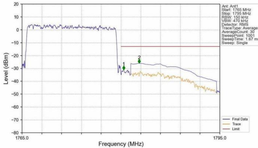
Band66_15MHz_16QAM_HCH_1772.5MHz_RB_75_0_NTNV
