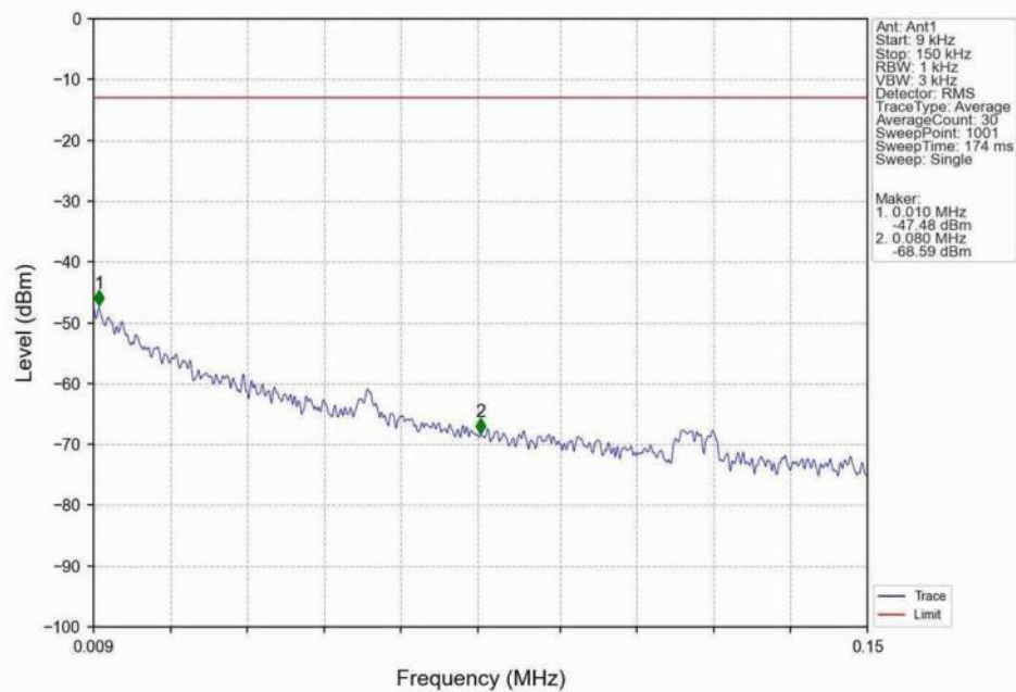
Band66_10MHz_16QAM_HCH_1775MHz_RB_1_0 NTN
