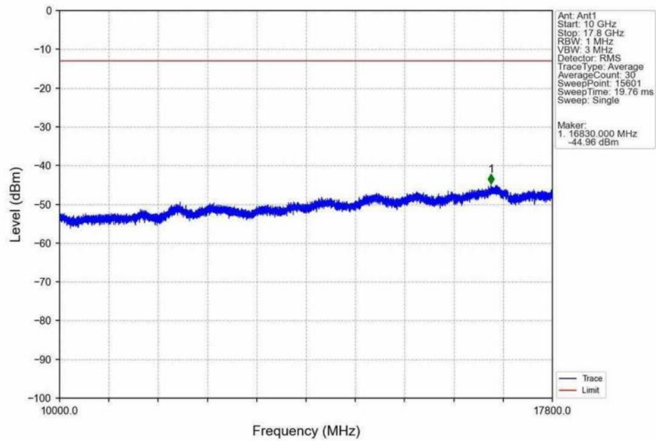
Band66_10MHz_16QAM_HCH_1775MHz_RB_1_0 NTN
