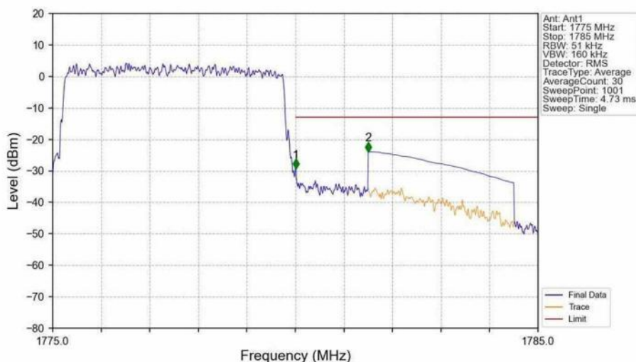
Band66_5MHz_16QAM_HCH_1777.5MHz_RB_25_0_NTNV
