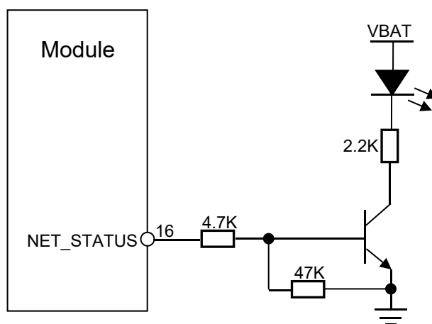
Figure 3.5.1-1 NET_STATUS Circuit
