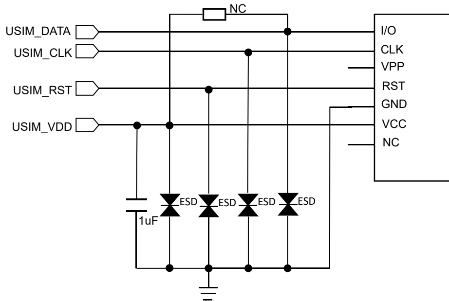
Figure 3.2.2-1 (U)SIM Circuit
