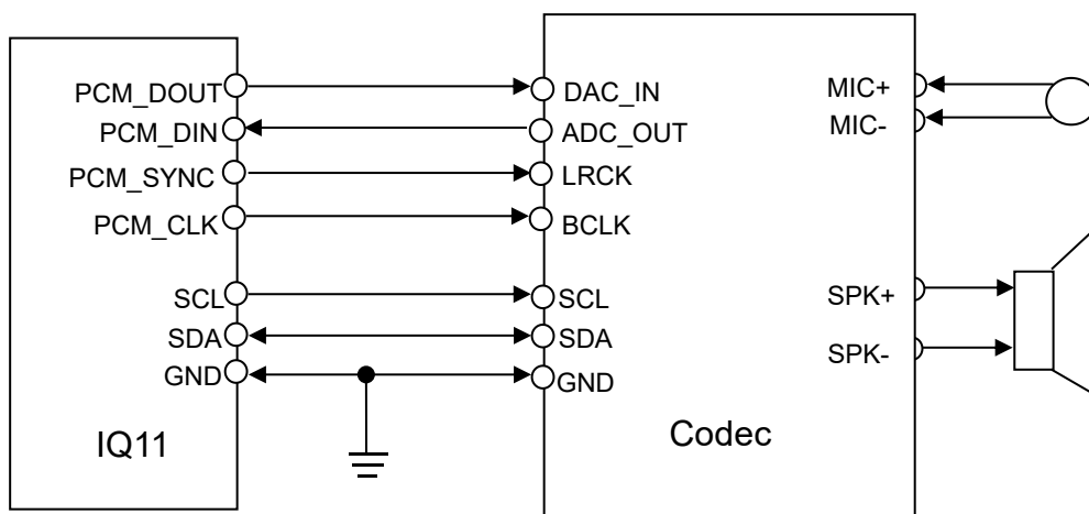
Figure 3.5.1-1 PCM Application Circuit (IQ11 module as PCM master device)
