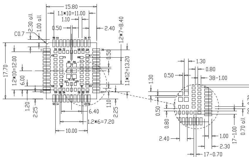
Figure 2.3.4-1 Recommend Pad (Top view, Unit: mm)
