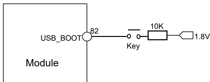
Figure 3.3.2-1 The USB_BOOT Circuit
