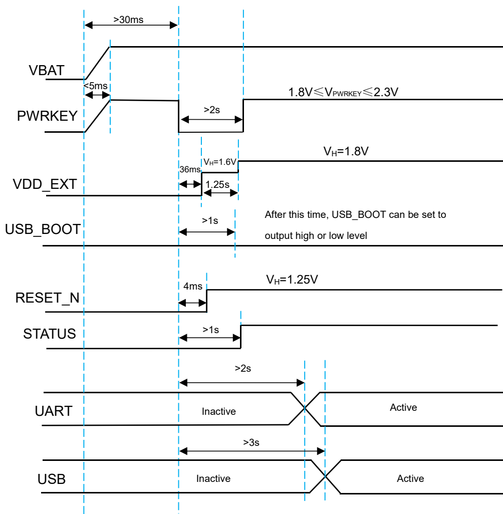
Figure 4.6-1 Power Sequence Diagram
