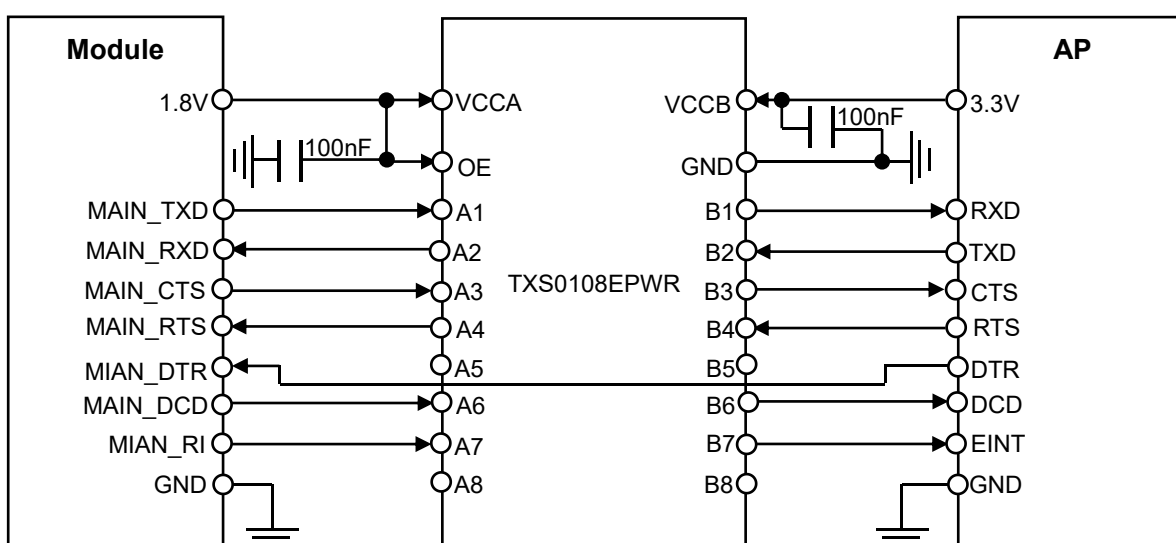
Figure 3.4.2-3 Level Conversion Circuit
