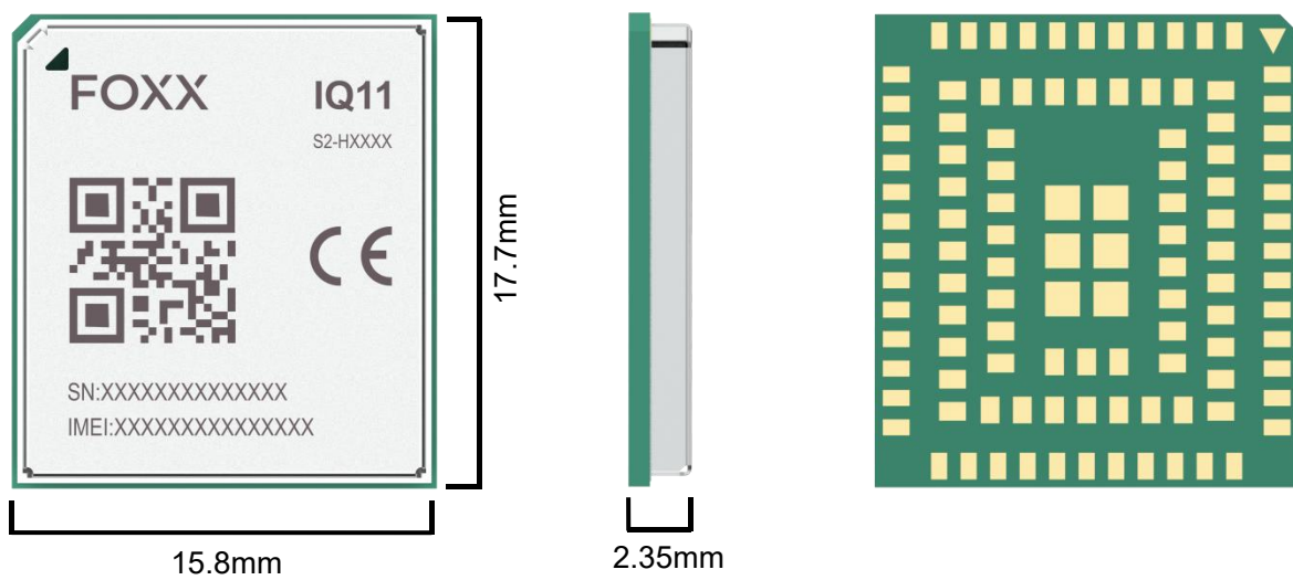
Figure 2.3.1-1 Mechanical Dimensions (Top view, Side view, Back view)
