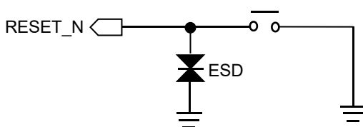
Figure 3.1.3-1 System Reset
