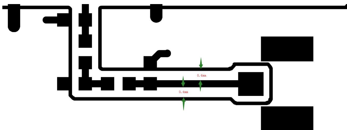
Figure 5.2-2 Antenna Path Reference Design
