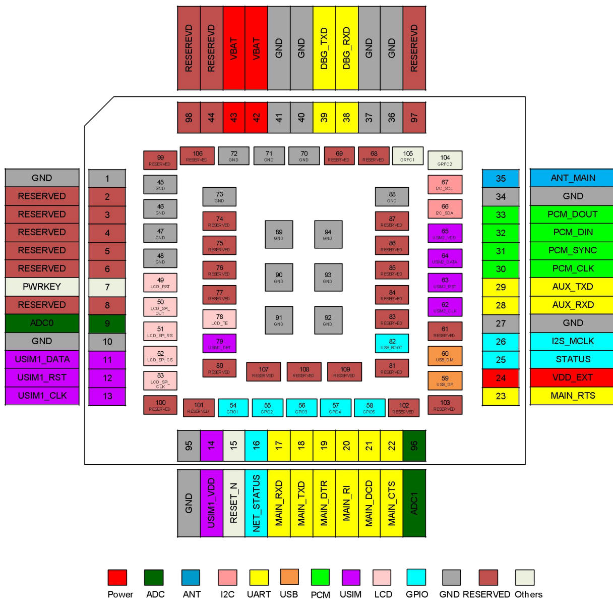
Figure 2.1-1 IQ11 Pin (Top View)
