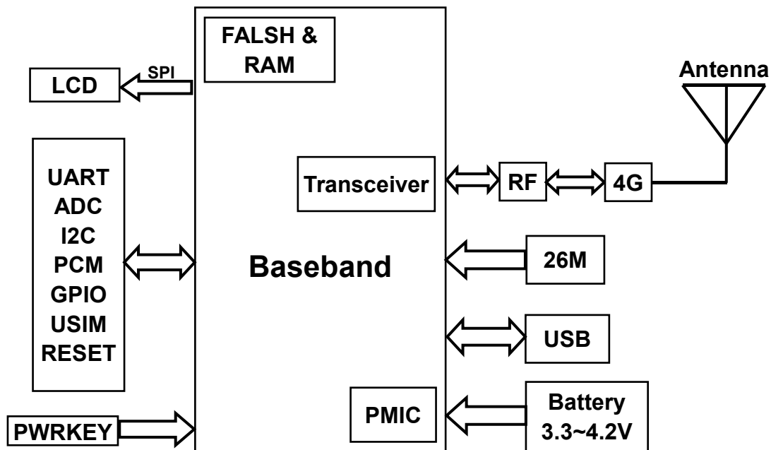
Figure 1.1-1 Functional Block Diagram
