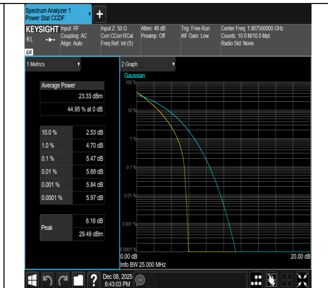
Band25-15MHz-64QAM-26115-75RB#0-PASS
