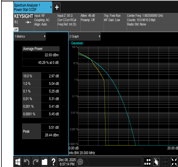
Band25-1.4MHz-16QAM-26683-1RB#0-PASS
