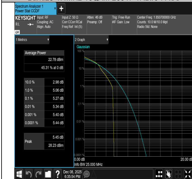
Band25-1.4MHz-16QAM-26365-1RB#0-PASS
