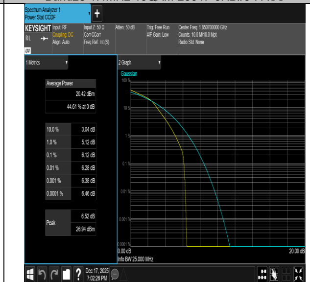
Band25-1.4MHz-16QAM-26365-6RB#0-PASS
