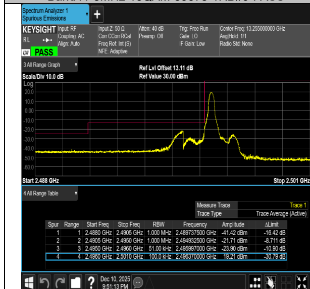
Band41-5MHz-16QAM-41565-1RB#24-PASS
