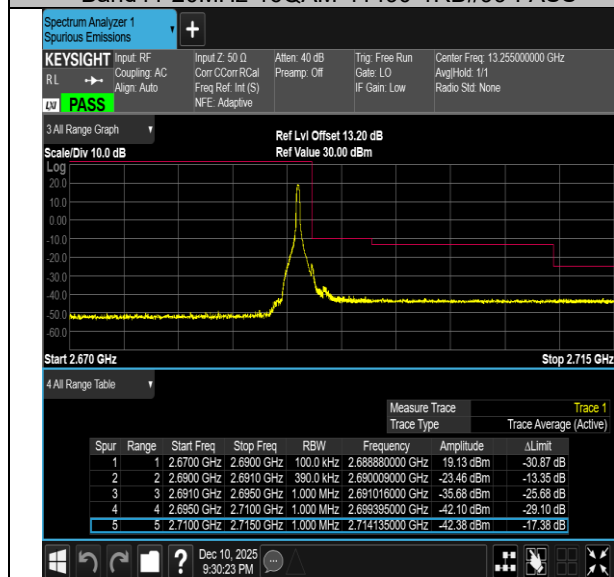
Band41-20MHz-16QAM-41490-1RB#99-PASS
