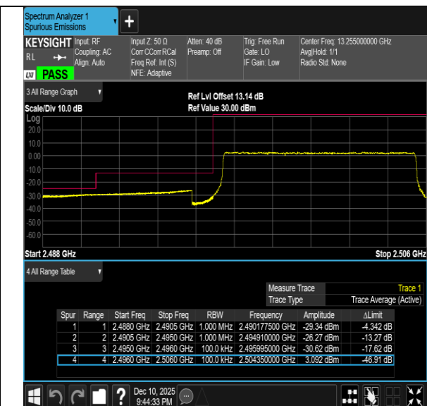
Band41-10MHz-QPSK-41540-50RB#0-PASS
