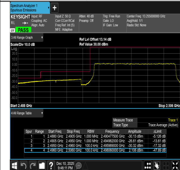
Band41-10MHz-16QAM-41540-50RB#0-PASS
