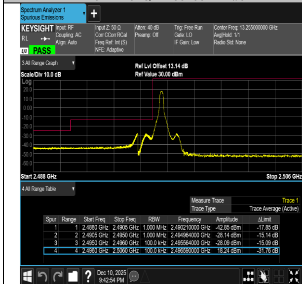
Band41-10MHz-64QAM-41540-1RB#49-PASS
