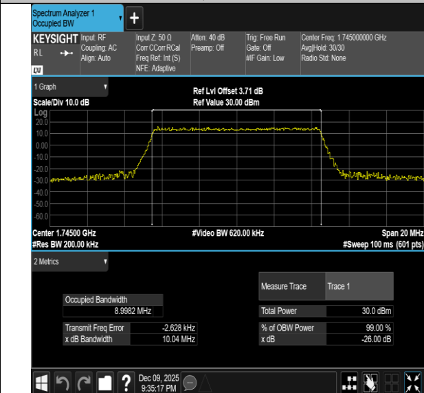
Band66-10MHz-16QAM-132022-50RB#0-PASS
