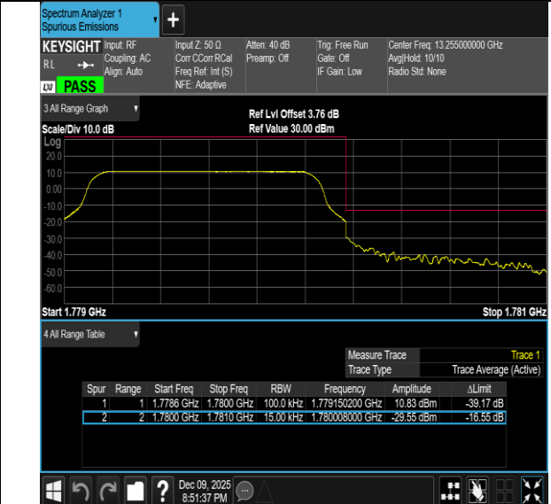
Band66-1.4MHz-16QAM-131979-6RB#0-PASS
