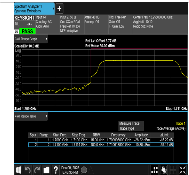
Band66-1.4MHz-64QAM-132665-6RB#0-PASS
