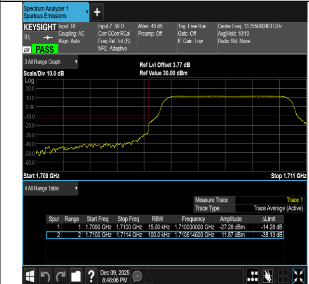
Band66-1.4MHz-16QAM-132665-6RB#0-PASS
