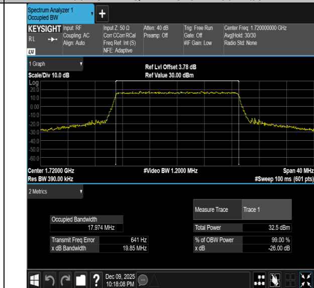
Band66-20MHz-QPSK-132572-100RB#0-PASS
