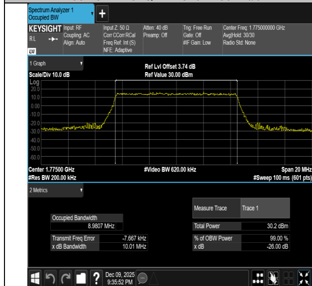
Band66-10MHz-16QAM-132322-50RB#0-PASS
