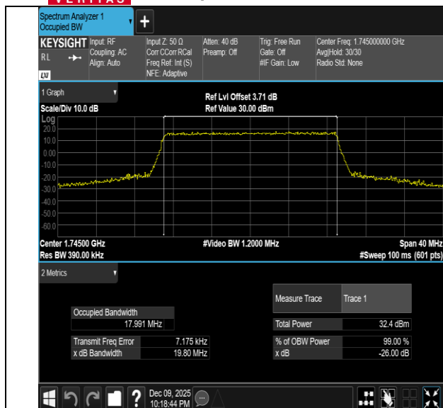
Band66-20MHz-64QAM-132072-100RB#0-PASS
