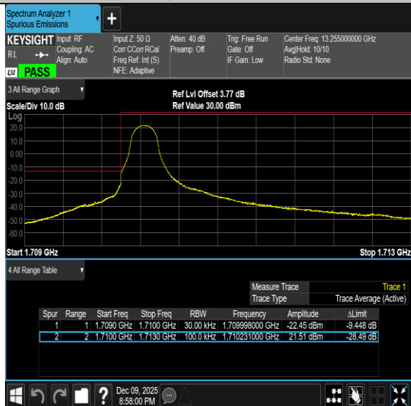
Band66-3MHz-QPSK-132657-1RB#14-PASS
