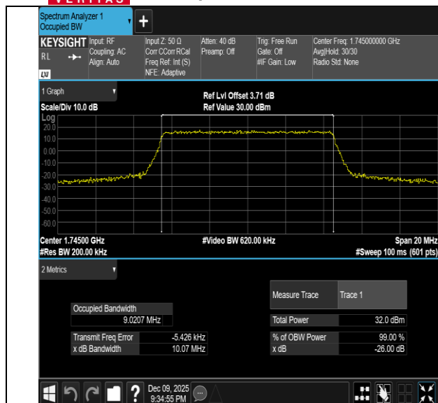
Band66-10MHz-64QAM-132022-50RB#0-PASS
