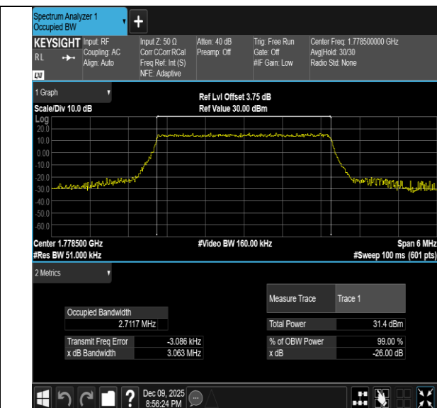
Band66-3MHz-64QAM-132322-15RB#0-PASS
