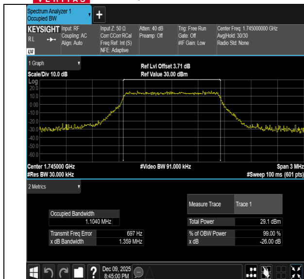
Band66-1.4MHz-16QAM-131979-6RB#0-PASS
