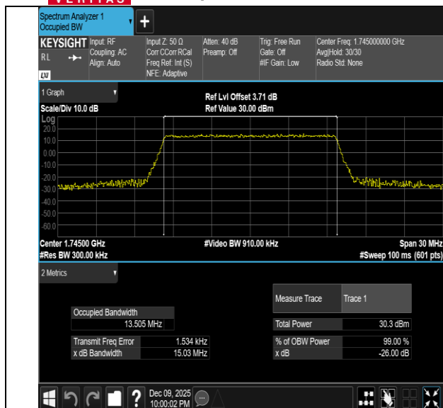
Band66-15MHz-16QAM-132047-75RB#0-PASS
