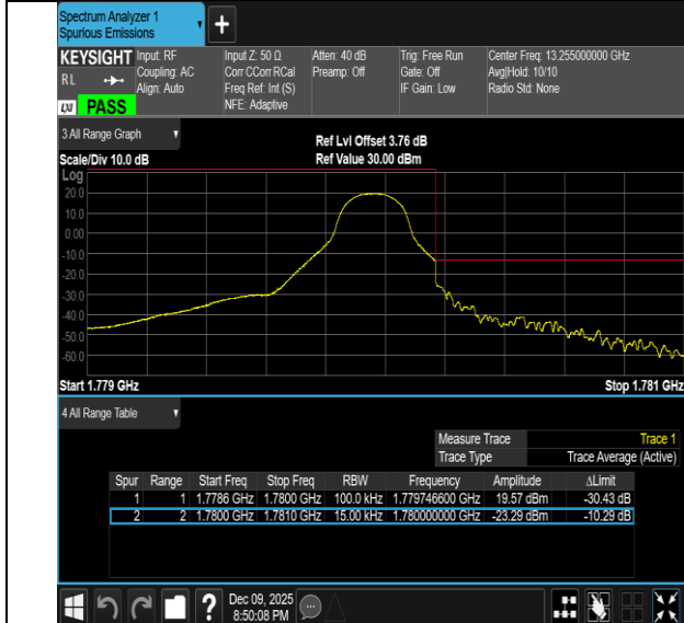
Band66-1.4MHz-16QAM-131979-1RB#0-PASS
