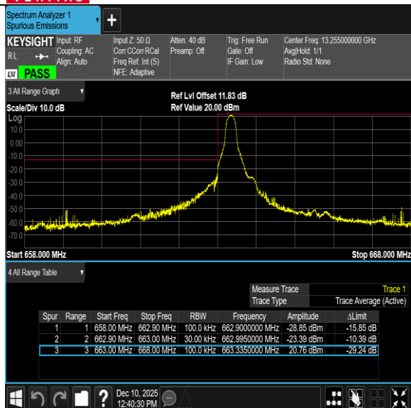
Band71-5MHz-QPSK-133447-1RB#24-PASS
