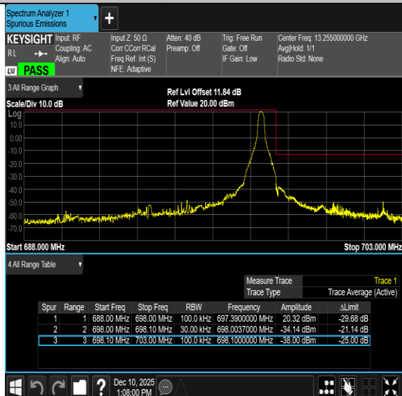
Band71-10MHz-64QAM-133172-1RB#0-PASS
