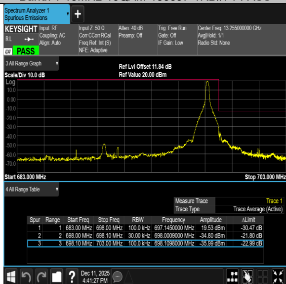
Band71-20MHz-QPSK-133222-1RB#0-PASS
