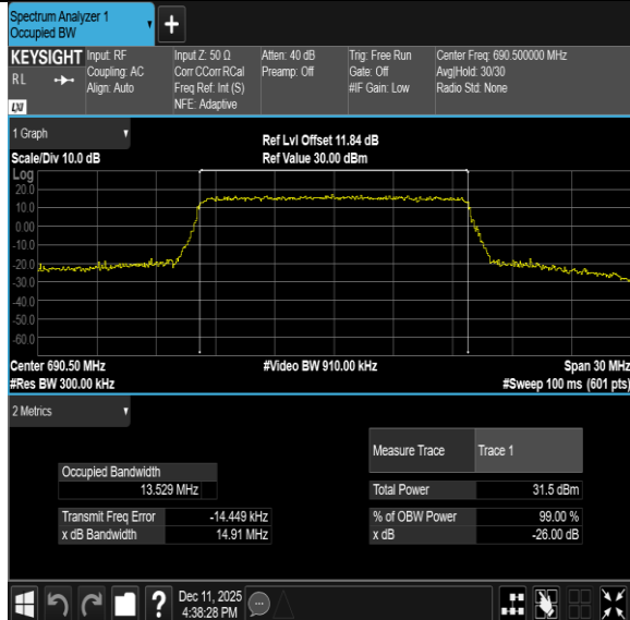
Band71-15MHz-64QAM-133297-75RB#0-PASS
