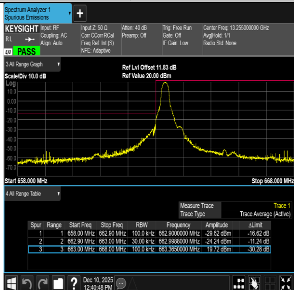
Band71-5MHz-16QAM-133447-1RB#24-PASS
