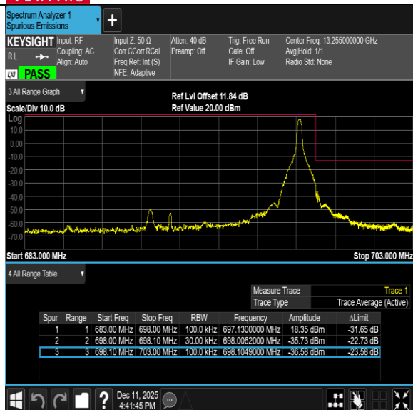
Band71-15MHz-16QAM-133197-1RB#0-PASS
