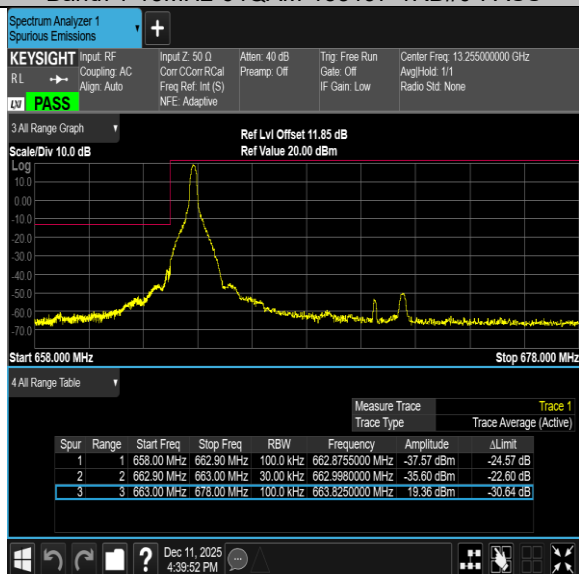
Band71-15MHz-64QAM-133397-1RB#74-PASS
