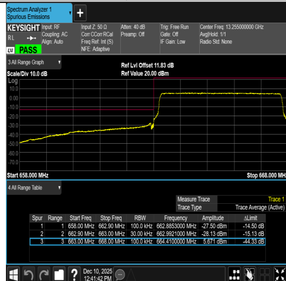
Band71-5MHz-16QAM-133447-25RB#0-PASS
