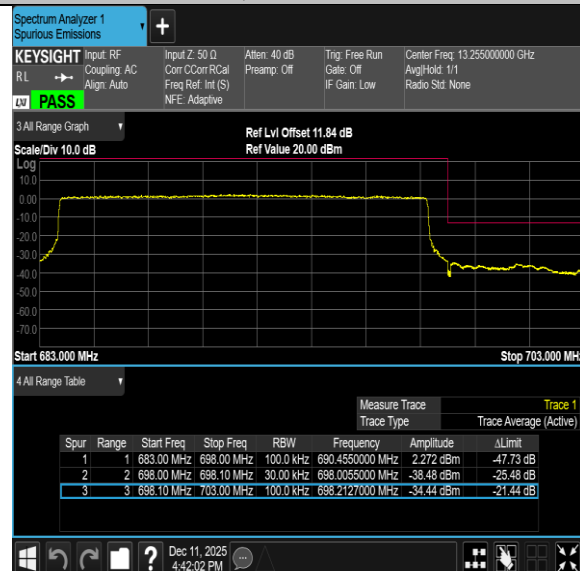
Band71-15MHz-64QAM-133197-75RB#0-PASS
