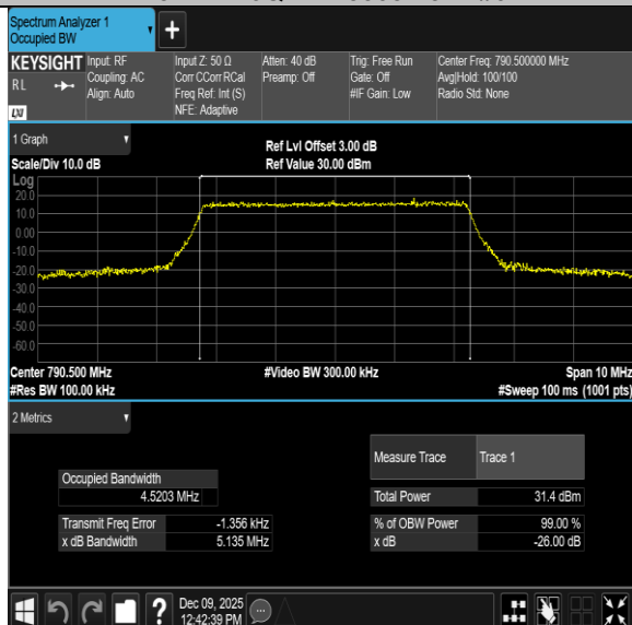
Band14-5MHz-16QAM-23355-25RB#0-PASS
