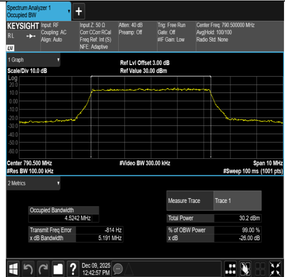
Band14-5MHz-64QAM-23355-25RB#0-PASS
