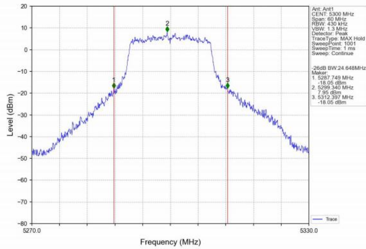
802.11n(HT20)_MCH_5300MHz_Ant1_NTNV
