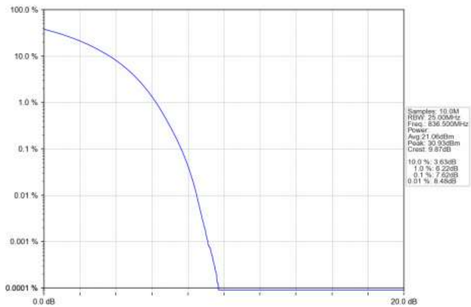
n5_15kHz_SISO_NTNV_20MHz_CP-OFDM_QPSK_836.5MHz_Outer_Full_Ant1
