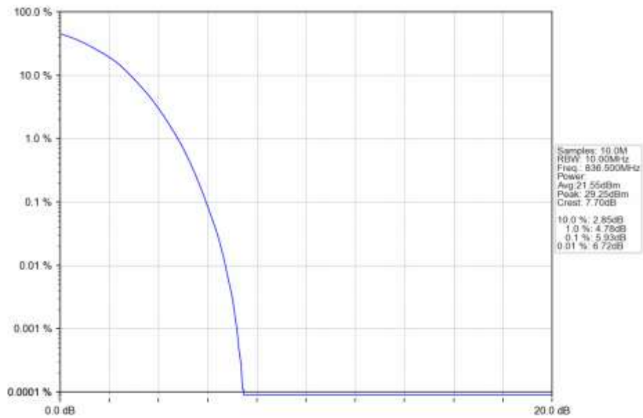
n5 30kHz SISO NTN 10MHz DFT-s-OFDM 64 QAM 836.5MHz Outer Full Ant1
