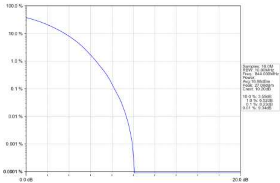
n5_15kHz_SISO_NTNV_10MHz_CP-OFDM_256_QAM_844MHz_Outer_Full_Ant1
