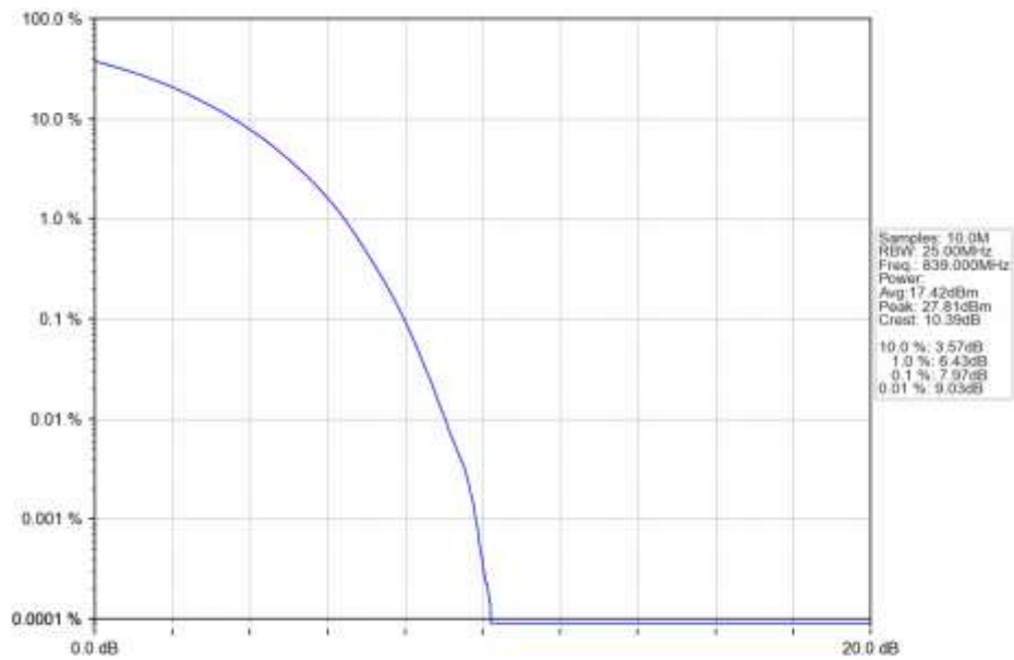
n5_15kHz_SISO_NTNV_20MHz_CP-OFDM_256_QAM_839MHz_Outer_Full_Ant1
