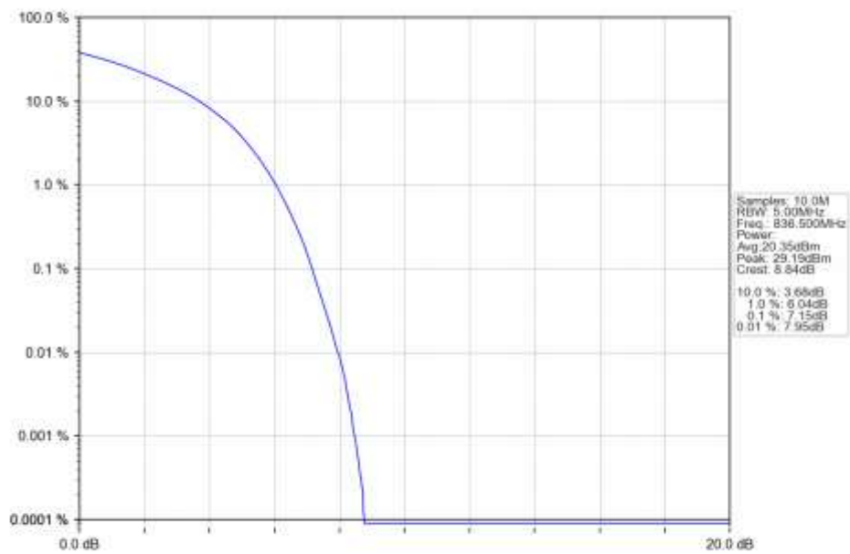
n5_15kHz_SISO_NTNV_5MHz_CP-OFDM_64_QAM_836.5MHz_Outer_Full_Ant1
