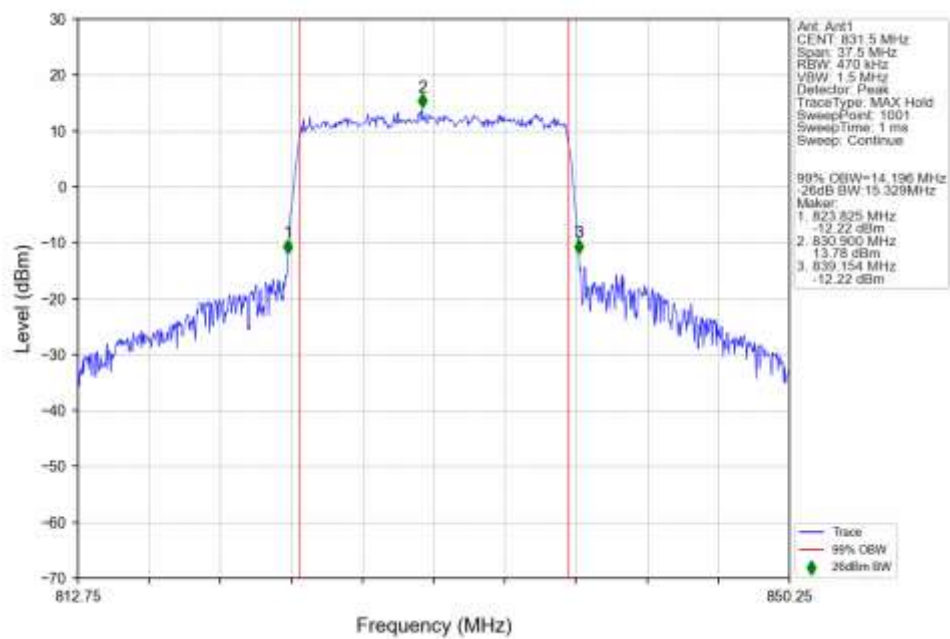
n5_15kHz_SISO_NTNV_15MHz_CP-OFDM_256_QAM_831.5MHz_Outer_Full_Ant1
