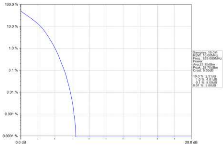
n5_30kHz_SISO_NTNV_10MHz_DFT-s-OFDM QPSK_829MHz_Outer_Full_Ant1
