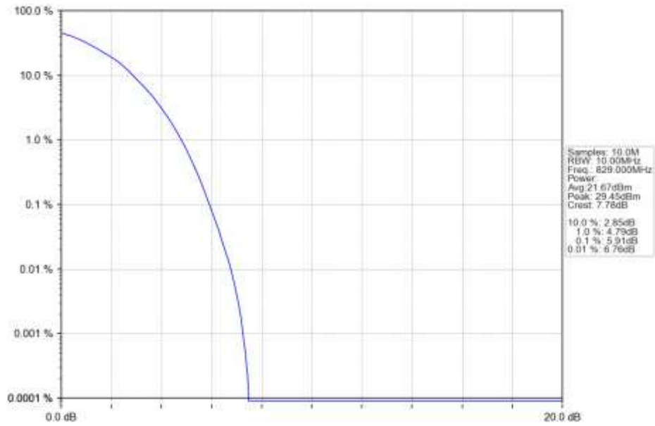
n5 30kHz SISO NTN 10MHz DFT-s-OFDM 64 QAM 829MHz Outer Full Ant1
