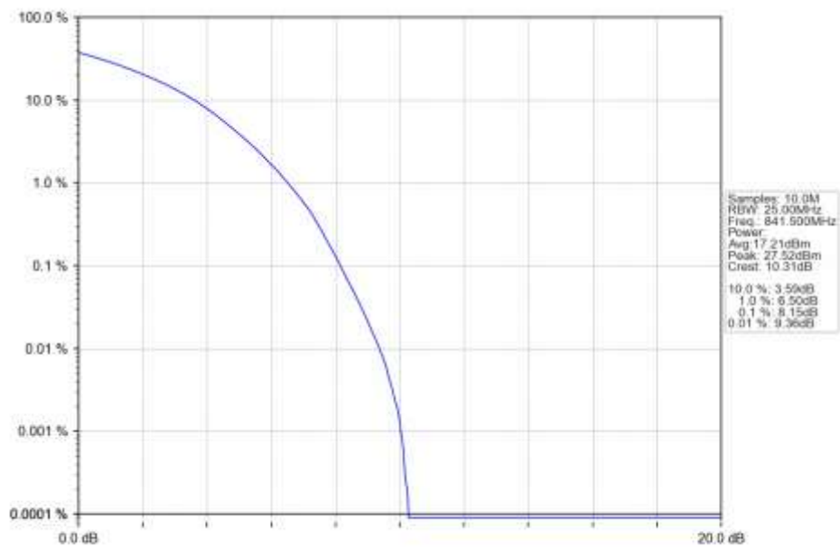
n5_15kHz_SISO_NTNV_15MHz_CP-OFDM_256_QAM_841.5MHz_Outer_Full_Ant1
