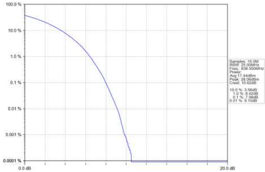
n5_15kHz_SISO_NTNV_20MHz_CP-OFDM_256_QAM_836.5MHz_Outer_Full_Ant1
