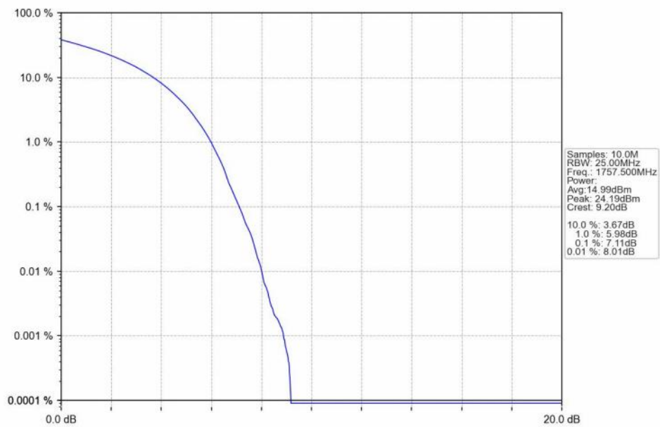
n66_15kHz_SISO_NTNV_45MHz_DFT-s-OFDM_16_QAM_1757.5MHz_Outer_Full_Ant1
