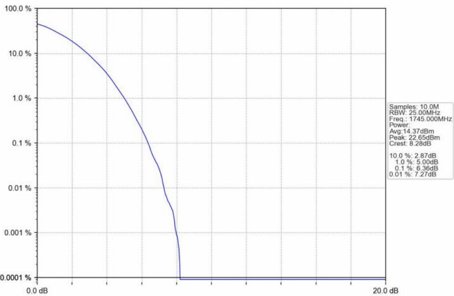
n66_30kHz_SISO_NTNV_20MHz_DFT-s-OFDM_256_QAM_1745MHz_Outer_Full_Ant1
