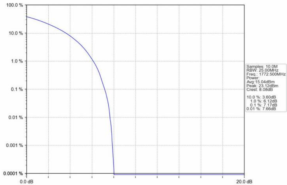
n66_30kHz_SISO_NTNV_15MHz_CP-OFDM_16_QAM_1772.5MHz_Outer_Full_Ant1
