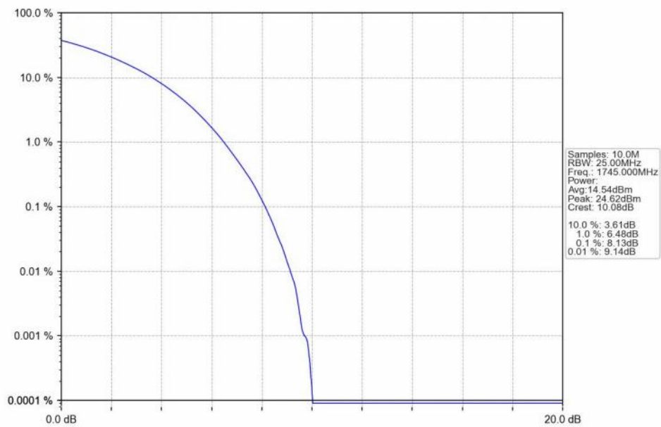
n66_15kHz_SISO_NTNV_45MHz_CP-OFDM QPSK_1745MHz_Outer_Full_Ant1
