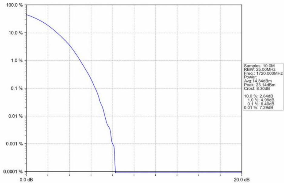
n66_30kHz_SISO_NTNV_20MHz_DFT-s-OFDM 256 QAM_1720MHz_Outer_Full_Ant1
