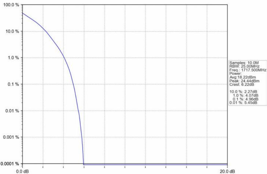
n66_30kHz_SISO_NTNV_15MHz_DFT-s-OFDM QPSK_1717.5MHz_Outer_Full_Ant1
