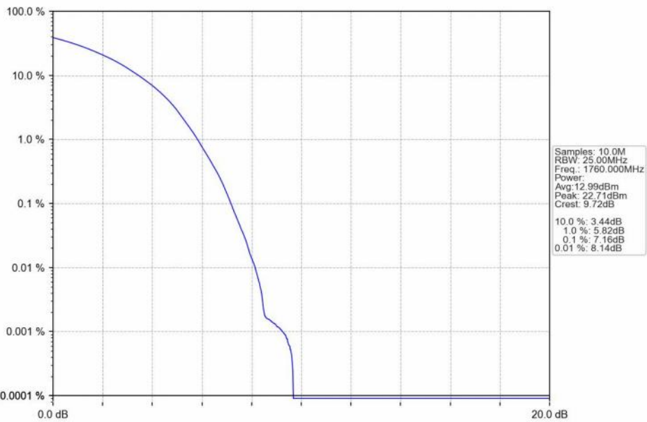
n66_15kHz_SISO_NTNV_40MHz_DFT-s-OFDM_256_QAM_1760MHz_Outer_Full_Ant1
