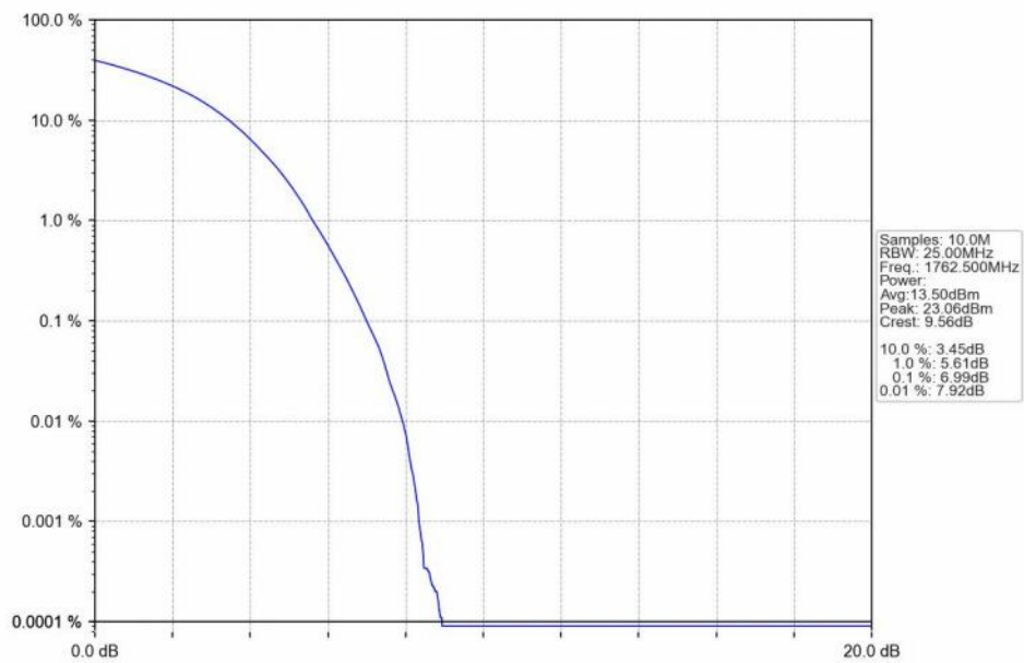
n66_15kHz_SISO_NTNV_35MHz_DFT-s-OFDM_256_QAM_1762.5MHz_Outer_Full_Ant1
