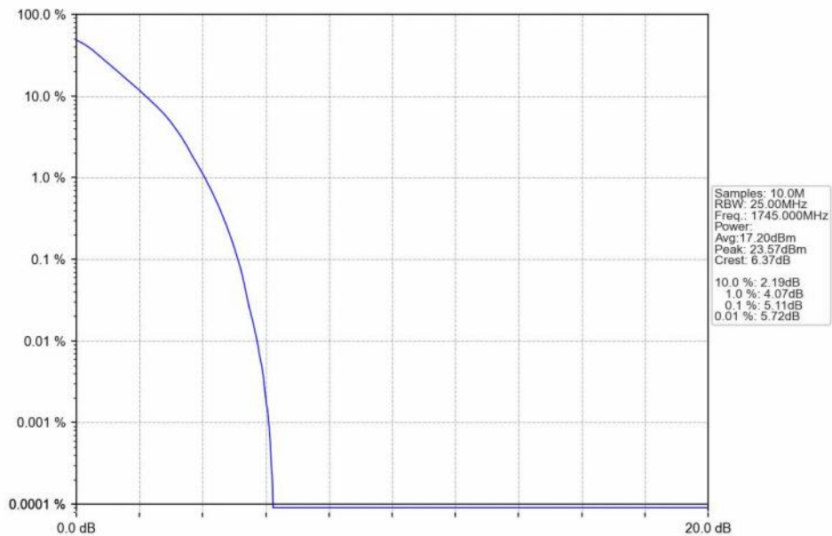
n66_15kHz_SISO_NTNV_20MHz_DFT-s-OFDM QPSK_1745MHz_Outer_Full_Ant1
