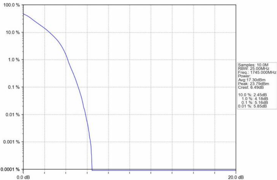
n66_15kHz_SISO_NTNV_25MHz_DFT-s-OFDM QPSK_1745MHz_Outer_Full_Ant1
