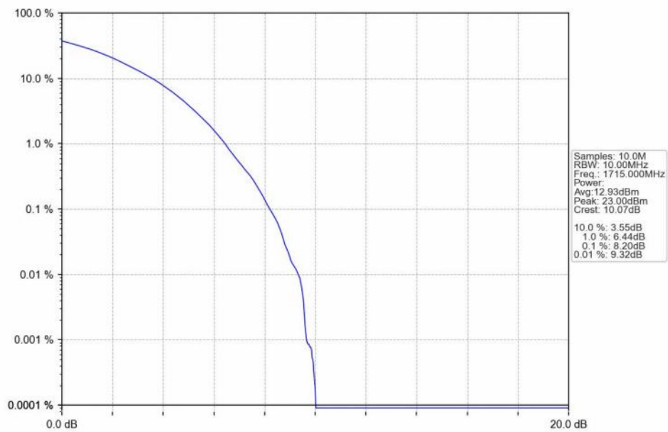
n66_30kHz_SISO_NTNV_10MHz_CP-OFDM 256 QAM_1715MHz_Outer_Full_Ant1
