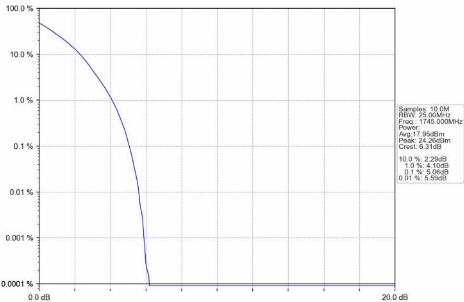
n66_30kHz_SISO_NTNV_15MHz_DFT-s-OFDM QPSK_1745MHz_Outer_Full_Ant1
