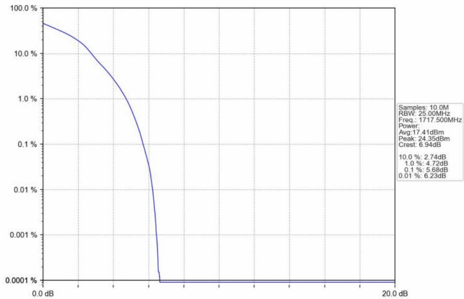
n66_30kHz_SISO_NTNV_15MHz_DFT-s-OFDM 16 QAM_1717.5MHz_Outer_Full_Ant1
