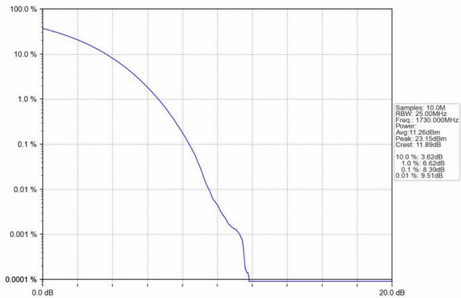
n66_15kHz_SISO_NTNV_40MHz_CP-OFDM 256 QAM_1730MHz_Outer_Full_Ant1
