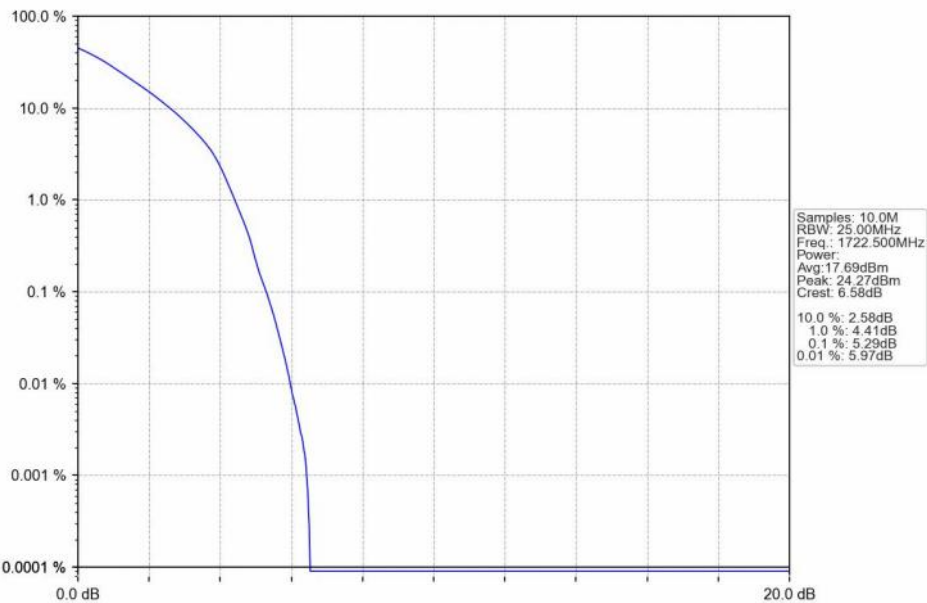
n66_15kHz_SISO_NTNV_25MHz_DFT-s-OFDM QPSK_1722.5MHz_Outer_Full_Ant1
