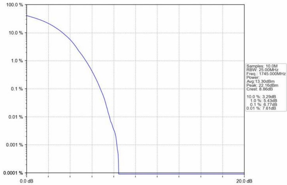
n66_15kHz_SISO_NTNV_35MHz_DFT-s-OFDM_256_QAM_1745MHz_Outer_Full_Ant1
