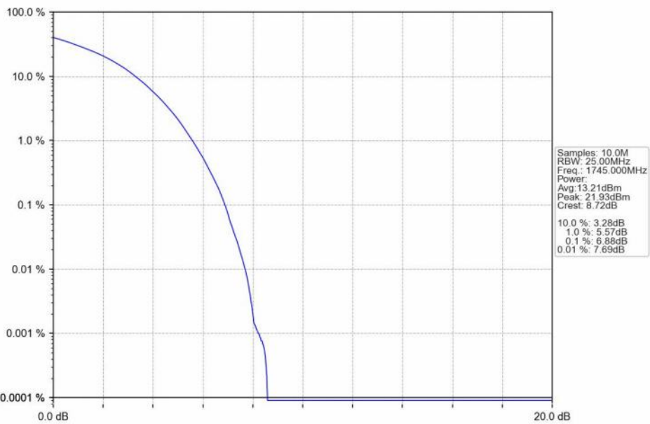
n66_15kHz_SISO_NTNV_40MHz_DFT-s-OFDM_256_QAM_1745MHz_Outer_Full_Ant1
