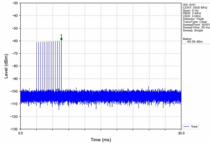
Signal Calibration 802.11a 2C 5500MHz RadarType5 Trial0
