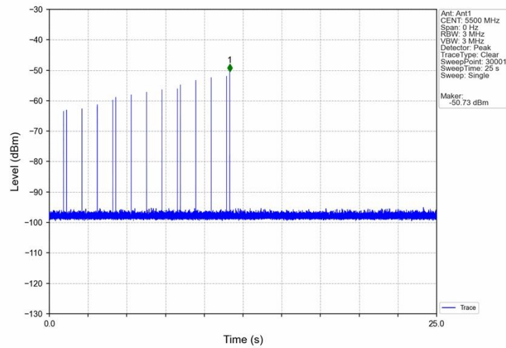
Signal Calibration 802.11a 2C 5500MHz RadarType5 Trial0
