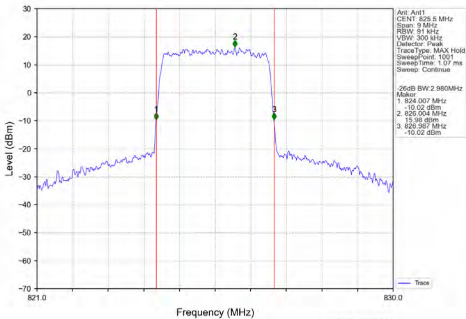
Band26b 3MHz 16QAM LCH 825.5MHz RB 15 0 NTNV
