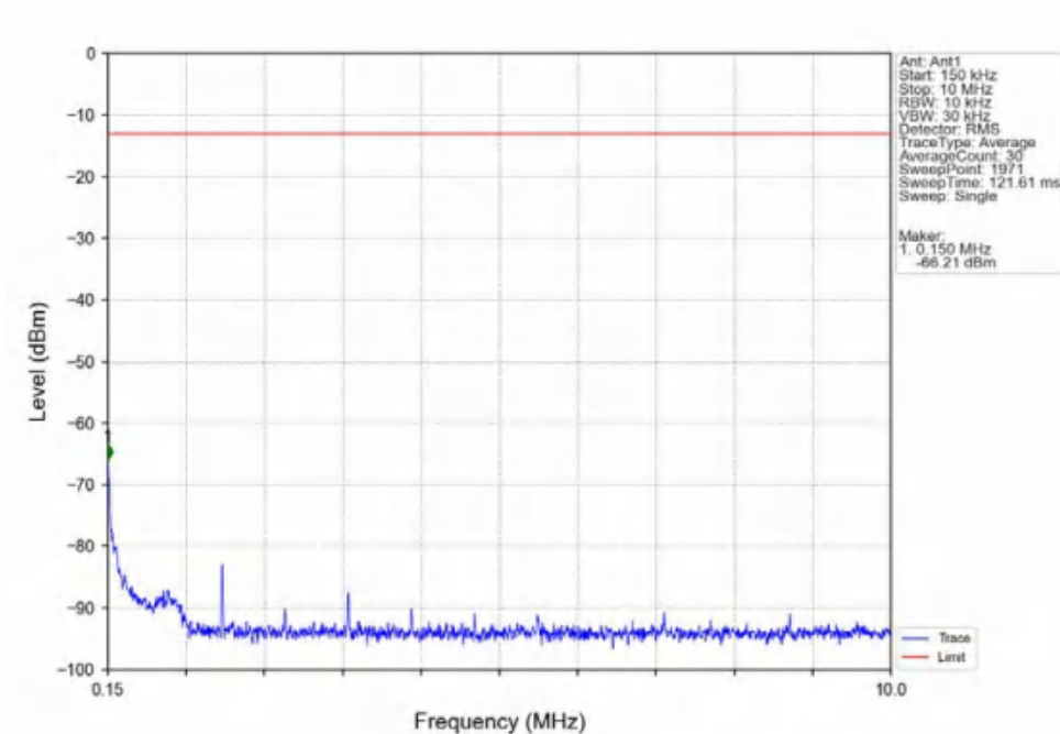
Band2_1.4MHz_16QAM_MCH_1880MHz_RB_1_0_NTNV
