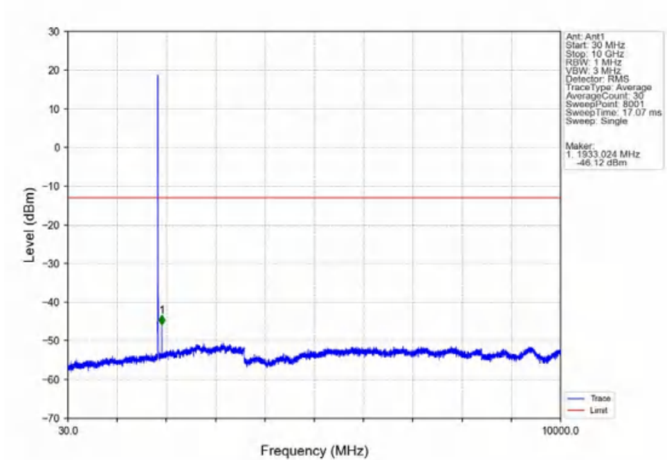
Band2_5MHz_QPSK_LCH_1852.5MHz_RB_1_0_NTNV
