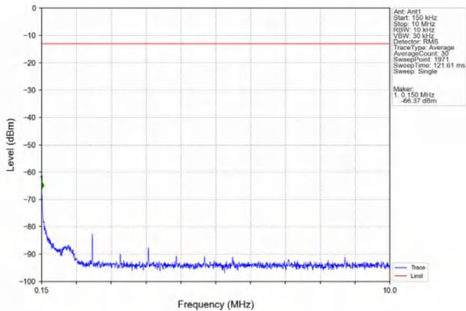
Band2_1.4MHz_16QAM_LCH_1850.7MHz_RB_1_0_NTNV
