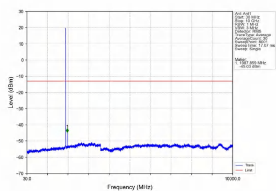
Band2_3MHz_16QAM_HCH_1908.5MHz_RB_1_0_NTNV
