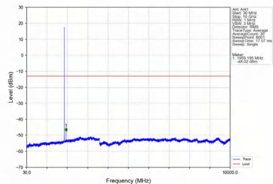
Band2_1.4MHz_16QAM_MCH_1880MHz_RB_1_0_NTNV
