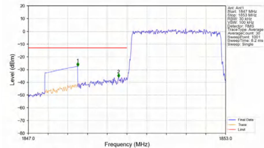
Band2_3MHz_16QAM_LCH_1851.5MHz_RB_15_0_NTNV
