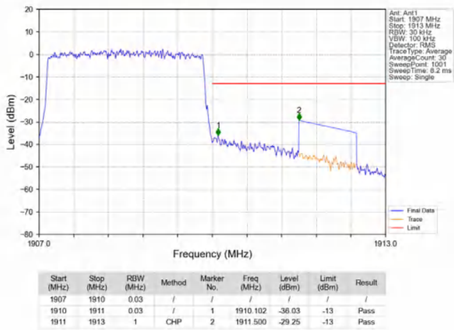
Band2_3MHz_16QAM_HCH_1908.5MHz_RB_15_0_NTNV
