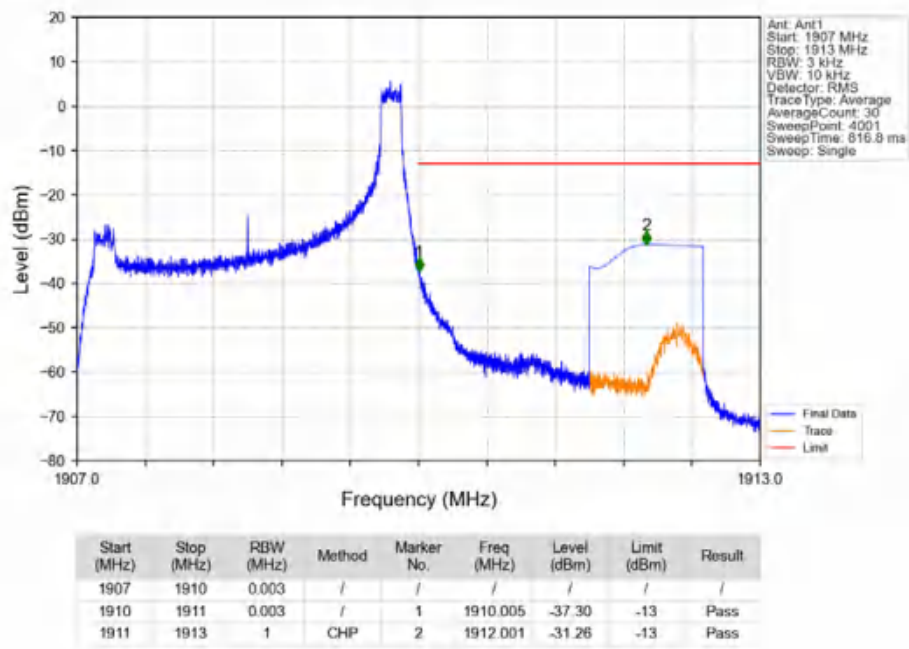
Band2_3MHz_16QAM_HCH_1908.5MHz_RB_15_0_NTNV
