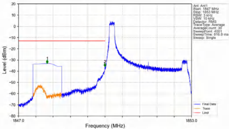
Band2_3MHz_16QAM_LCH_1851.5MHz_RB_1_0_NTNV
