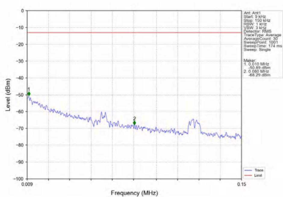
Band2_5MHz_16QAM_LCH_1852.5MHz_RB_1_0_NTNV
