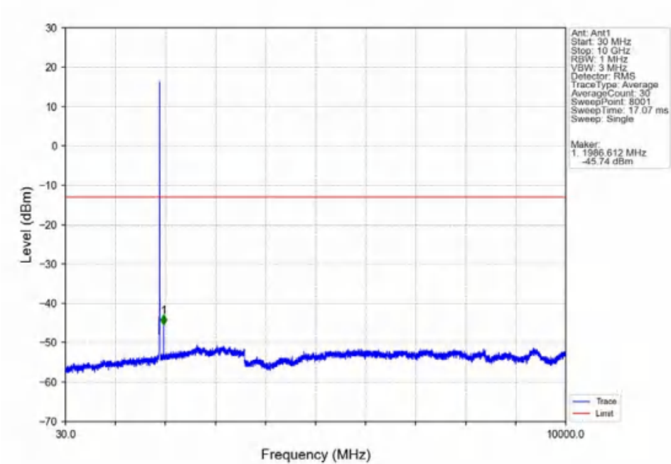
Band2_5MHz_16QAM_HCH_1907.5MHz_RB_1_0_NTNV
