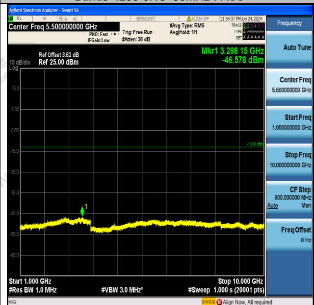
Band5-4233-1000~10000MHz-PASS
