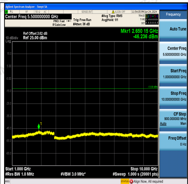
Band5-4182-1000~10000MHz-PASS
