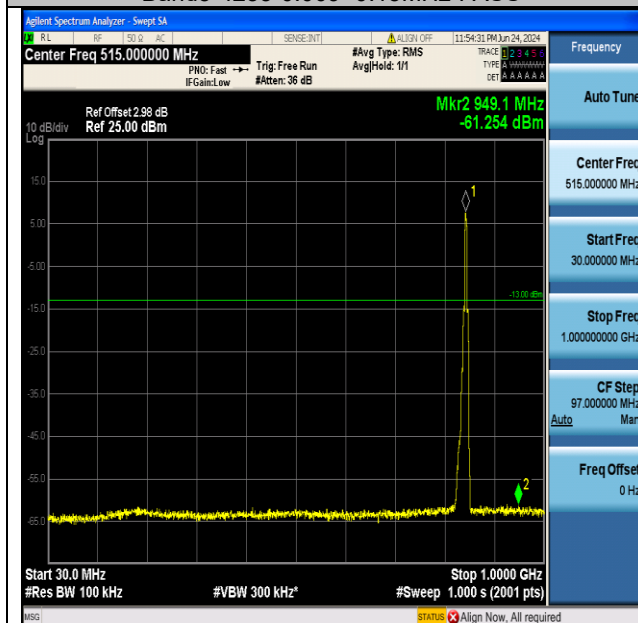
Band5-4233-30~1000MHz-PASS
