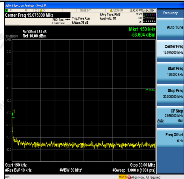
Band2-9538-0.15~30MHz-PASS
