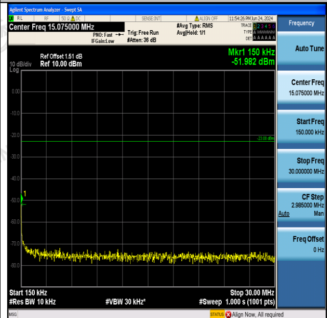
Band5-4233-0.15~30MHz-PASS
