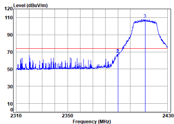
11ax_20M_TX_CH_01_Vertical-Peak
