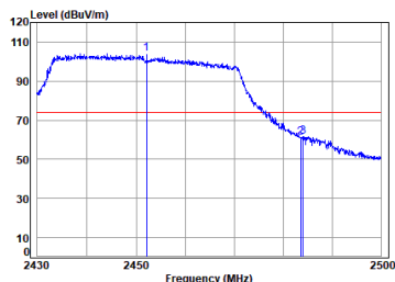
11ax_40M_TX_CH_09_Vertical-Peak
