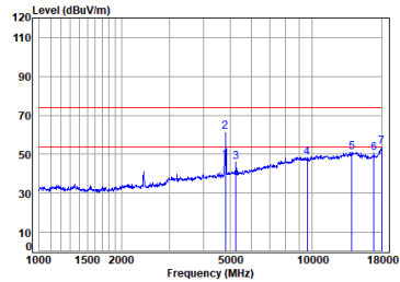
11ax_20M_TX_CH_01_Vertical
