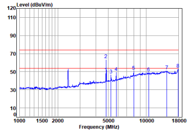
11g_TX_CH_01_Vertical
