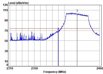
11ax_40M_TX_CH_03_Horizontal-Peak
