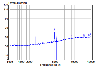
11g_TX_CH_11_Vertical
