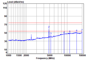
11ax_20M_TX_CH_06_Vertical
