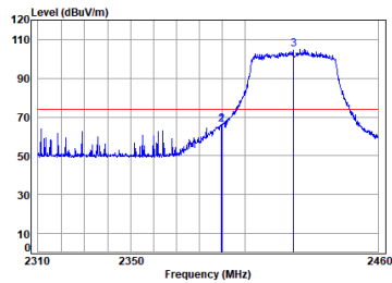
11ax_40M_TX_CH_03_Vertical-Peak
