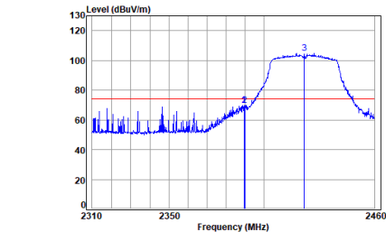
11n_HT(40M)_TX_CH_03_Horizontal-Peak
