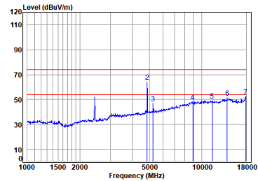
11g_TX_CH_06_Vertical
