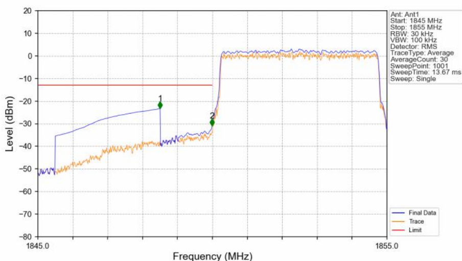
Band2_5MHz_16QAM_LCH_1852.5MHz_RB_25_0_NTNV
