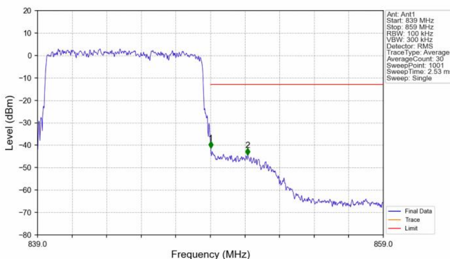
Band5_10MHz_16QAM_HCH_844MHz_RB_50_0_NTNV
