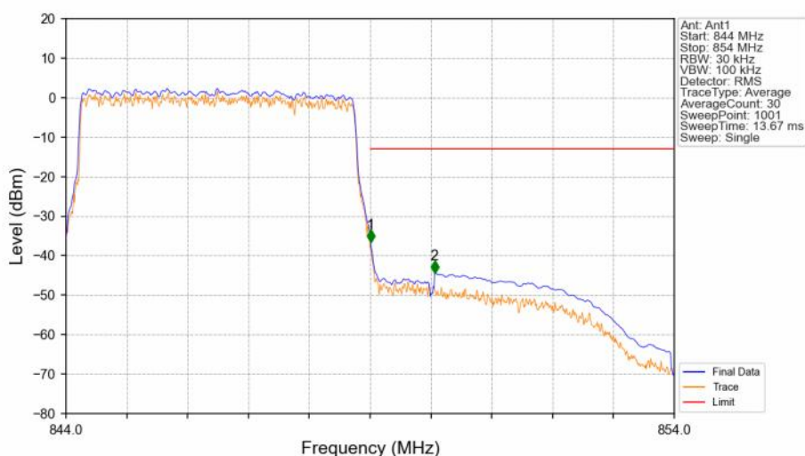
Band5_5MHz_QPSK_HCH_846.5MHz_RB_25_0_NTNV
