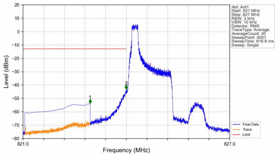
Band5_1.4MHz_16QAM_LCH_824.7MHz_RB_1_0_NTNV
