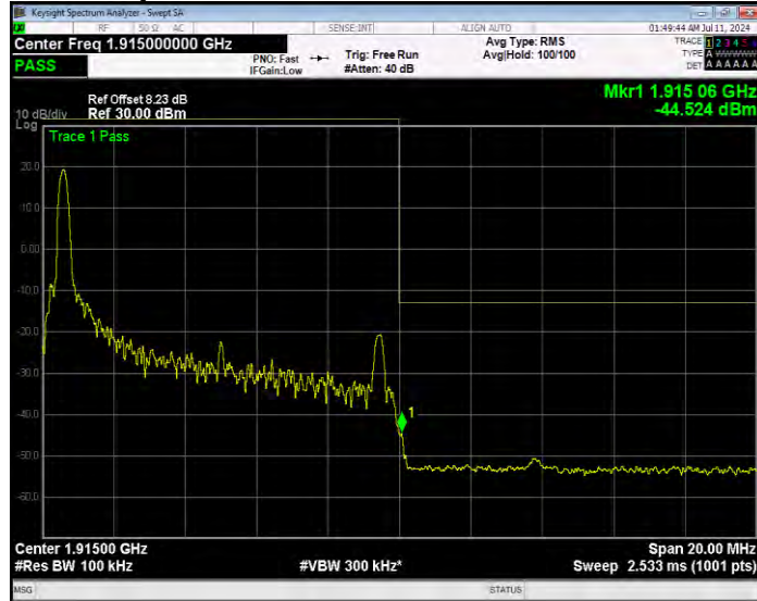
Band25 QPSK BW=10MHz Channel=26640 RB Size=1 Position=#Max Extended
