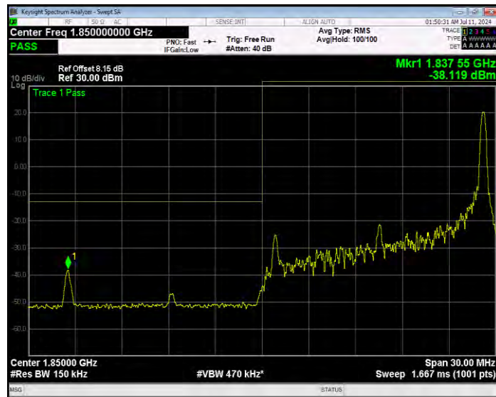
Band25 QPSK BW=15MHz Channel=26115 RB Size=75 Position=#0 Extended
