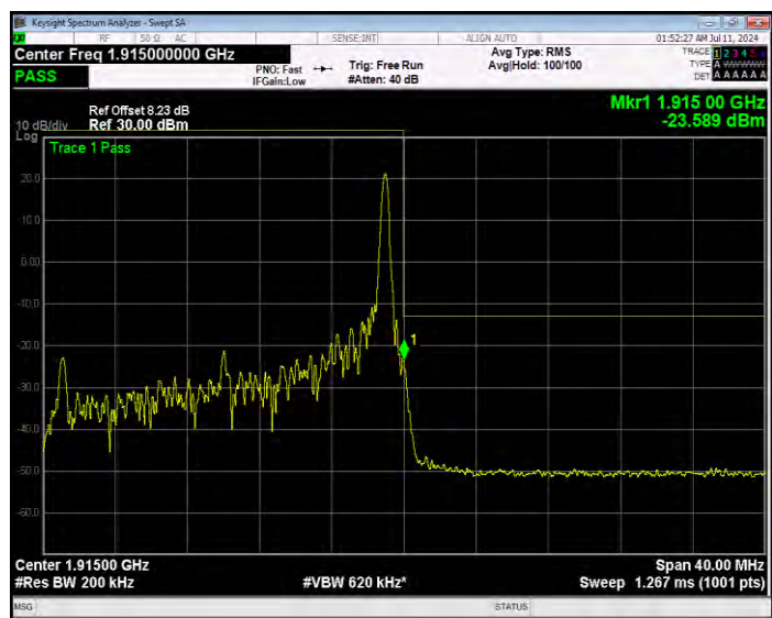
Band25 QPSK BW=20MHz Channel=26590 RB Size=100 Position=#0 Extended
