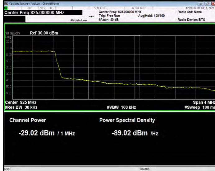
Band26(814-824) QPSK BW=1.4MHz Channel=26783 RB Size=6 Position=#0 Normal
