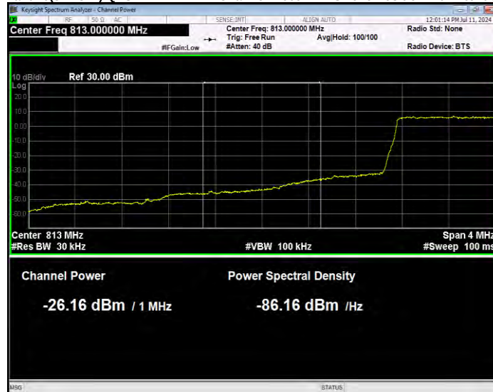
Band26(814-824) QPSK BW=1.4MHz Channel=26697 RB Size=6 Position=#0 Normal
