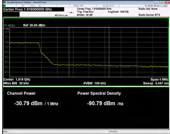
Band25 QPSK BW=5MHz Channel=26665 RB Size=25 Position=#0 Normal
