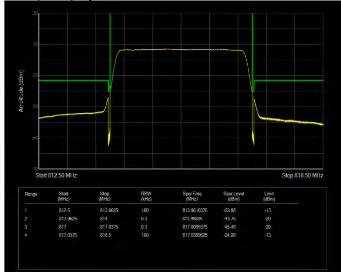
Band26(814-824) 16QAM BW=3MHz Channel=26775 RB Size=1 Position=#0 Extended
