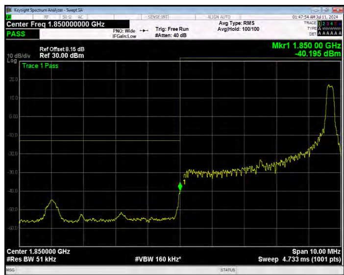
Band25 QPSK BW=5MHz Channel=26065 RB Size=25 Position=#0 Extended
