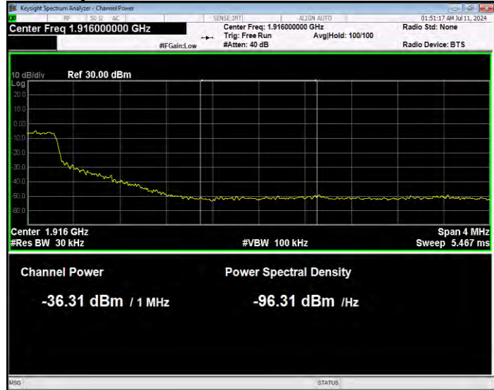
Band25 QPSK BW=15MHz Channel=26615 RB Size=75 Position=#0 Normal
