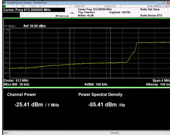
Band26(814-824) 16QAM BW=3MHz Channel=26705 RB Size=15 Position=#0 Normal
