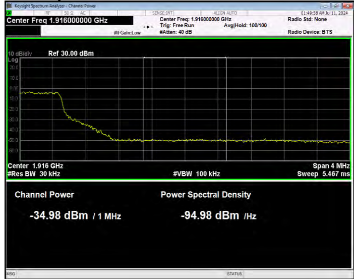
Band25 QPSK BW=10MHz Channel=26640 RB Size=50 Position=#0 Normal
