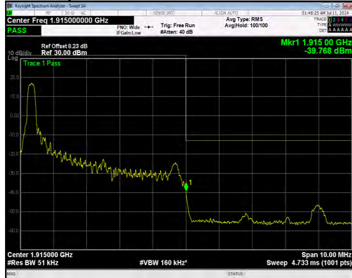
Band25 QPSK BW=5MHz Channel=26665 RB Size=1 Position=#Max Extended
