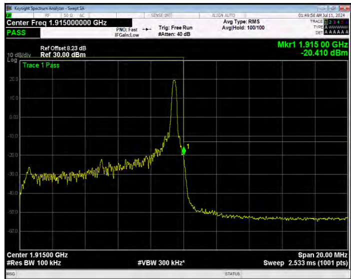
Band25 QPSK BW=10MHz Channel=26640 RB Size=50 Position=#0 Extended
