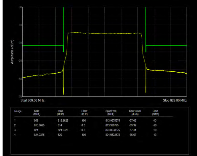
Band26(814-824) 16QAM BW=3MHz Channel=26705 RB Size=1 Position=#0 Extended
