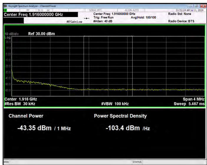
Band25 QPSK BW=20MHz Channel=26590 RB Size=1 Position=#0 Normal
