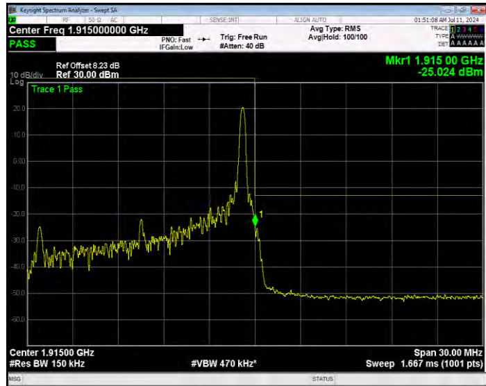
Band25 QPSK BW=15MHz Channel=26615 RB Size=75 Position=#0 Extended
