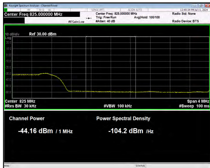
Band26(814-824) 16QAM BW=5MHz Channel=26765 RB Size=1 Position=#0 Normal
