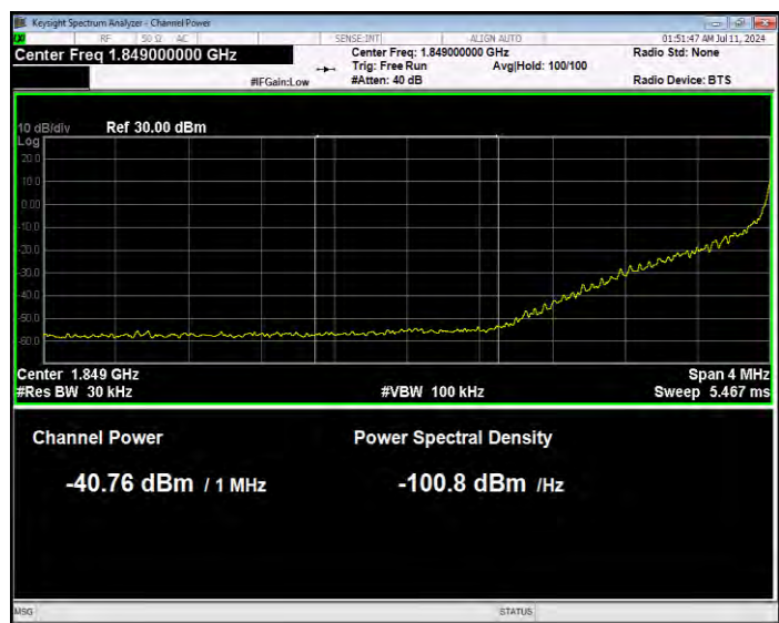
Band25 QPSK BW=20MHz Channel=26140 RB Size=1 Position=#0 Normal
