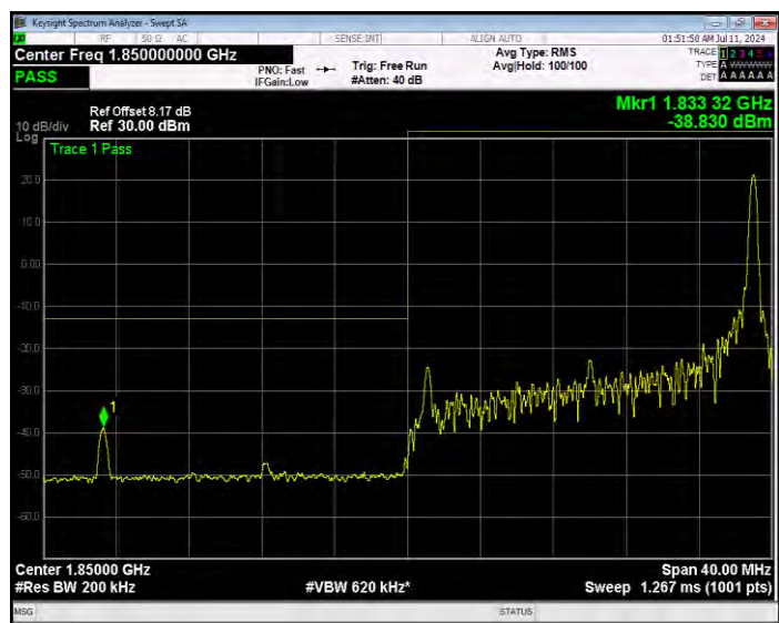
Band25 QPSK BW=20MHz Channel=26140 RB Size=100 Position=#0 Extended
