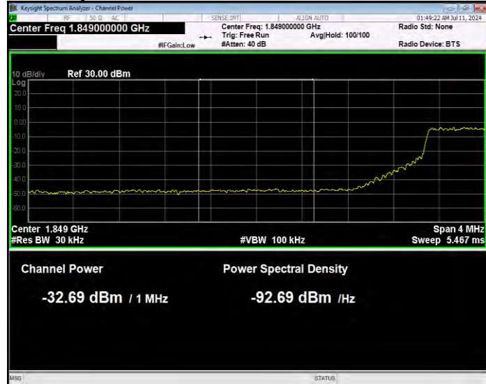
Band25 QPSK BW=10MHz Channel=26090 RB Size=50 Position=#0 Normal
