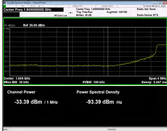
Band25 QPSK BW=15MHz Channel=26115 RB Size=75 Position=#0 Normal
