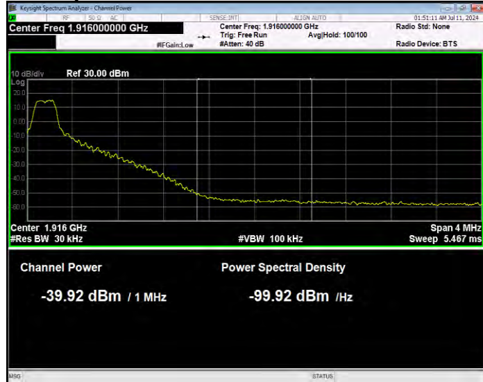
Band25 QPSK BW=15MHz Channel=26615 RB Size=1 Position=#Max Normal
