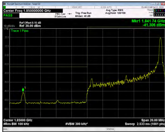
Band25 QPSK BW=10MHz Channel=26090 RB Size=50 Position=#0 Extended
