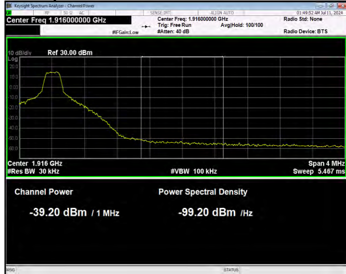
Band25 QPSK BW=10MHz Channel=26640 RB Size=1 Position=#Max Normal
