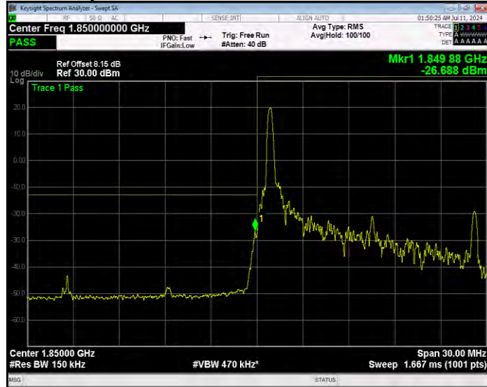
Band25 QPSK BW=15MHz Channel=26115 RB Size=1 Position=#Max Extended
