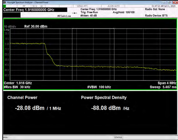
Band25 QPSK BW=3MHz Channel=26675 RB Size=15 Position=#0 Normal
