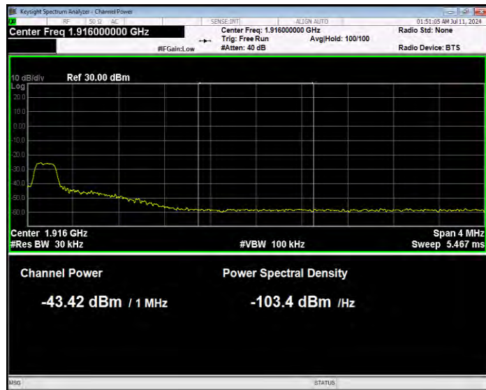
Band25 QPSK BW=15MHz Channel=26615 RB Size=1 Position=#0 Normal
