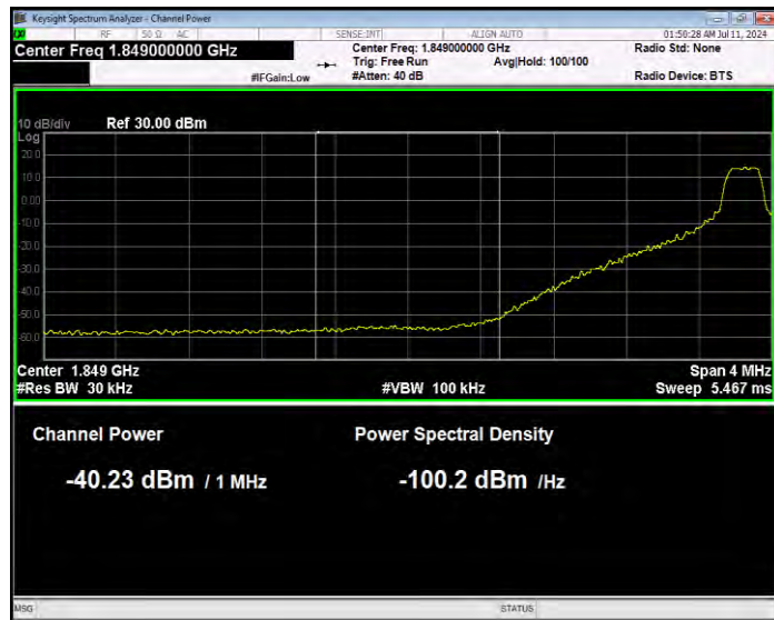
Band25 QPSK BW=15MHz Channel=26115 RB Size=1 Position=#0 Normal
