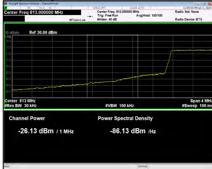
Band26(814-824) 16QAM BW=1.4MHz Channel=26697 RB Size=6 Position=#0 Normal
