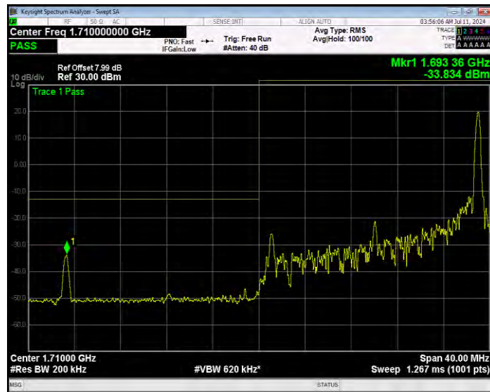
Band66 16QAM BW=20MHz Channel=132072 RB Size=100 Position=#0 Extended
