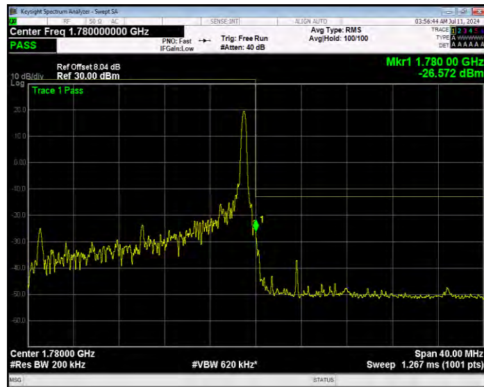
Band66 16QAM BW=20MHz Channel=132572 RB Size=100 Position=#0 Extended
