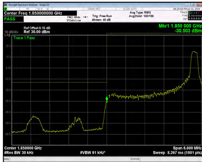
Band2 QPSK BW=3MHz Channel=18615 RB Size=15 Position=#0 Extended
