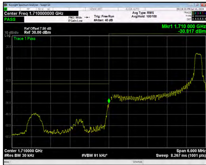
Band4 16QAM BW=3MHz Channel=19965 RB Size=15 Position=#0 Extended
