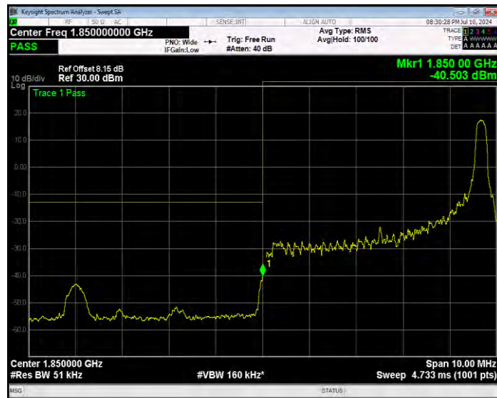
Band2 QPSK BW=5MHz Channel=18625 RB Size=25 Position=#0 Extended
