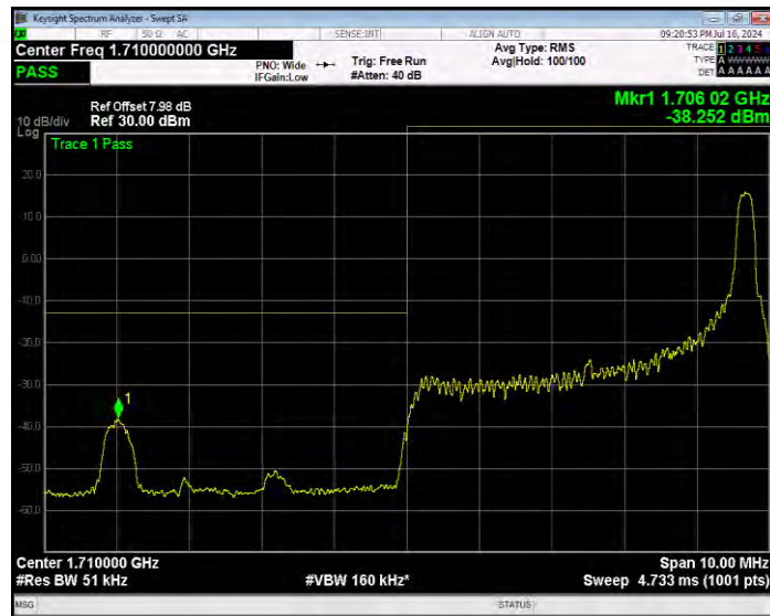
Band4 16QAM BW=5MHz Channel=19975 RB Size=25 Position=#0 Extended
