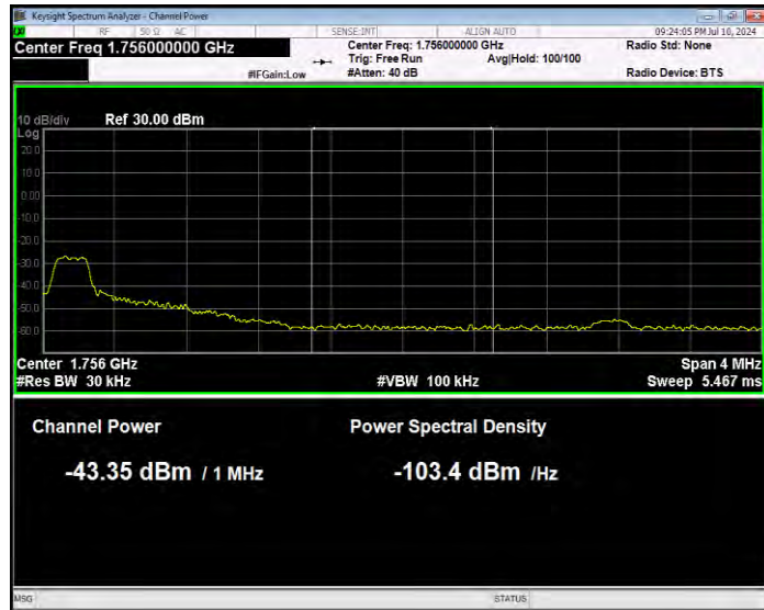
Band4 16QAM BW=15MHz Channel=20325 RB Size=1 Position=#0 Normal
