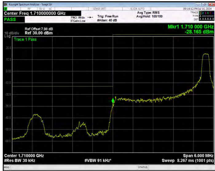
Band4 QPSK BW=3MHz Channel=19965 RB Size=15 Position=#0 Extended
