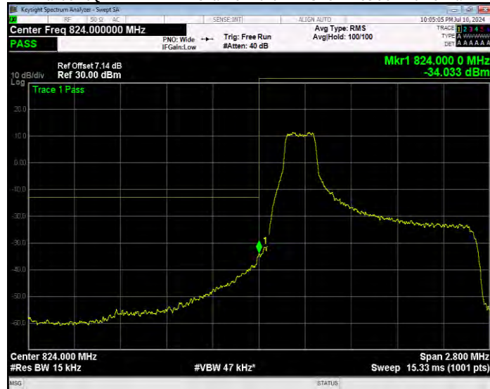
Band5 16QAM BW=1.4MHz Channel=20407 RB Size=1 Position=#Max Extended
