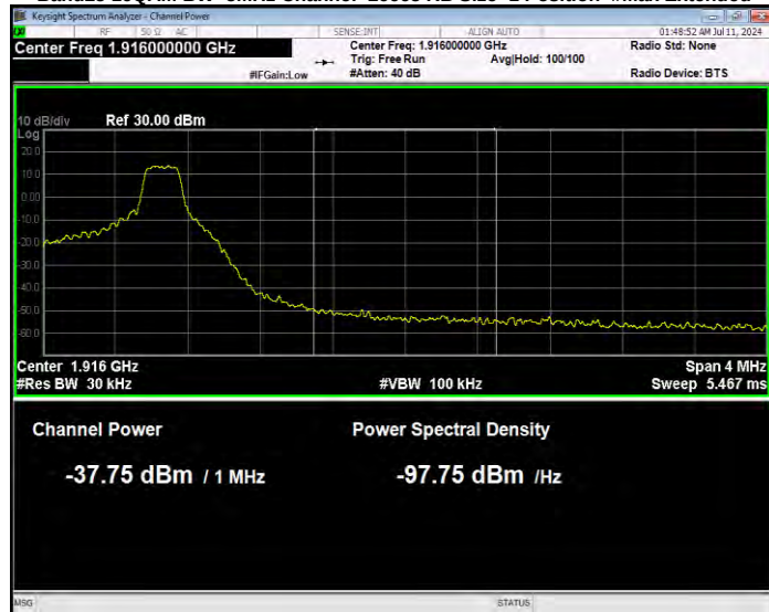
Band25 16QAM BW=5MHz Channel=26665 RB Size=1 Position=#Max Normal
