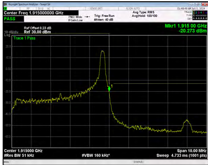
Band25 16QAM BW=5MHz Channel=26665 RB Size=25 Position=#0 Extended
