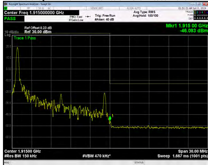
Band25 16QAM BW=15MHz Channel=26615 RB Size=1 Position=#Max Extended
