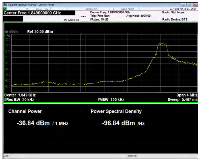
Band25 16QAM BW=3MHz Channel=26055 RB Size=1 Position=#0 Normal
