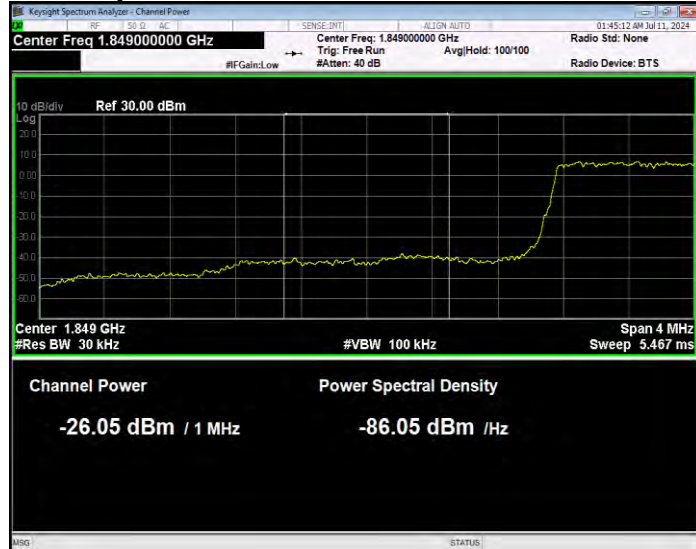
Band25 QPSK BW=1.4MHz Channel=26047 RB Size=6 Position=#0 Normal
