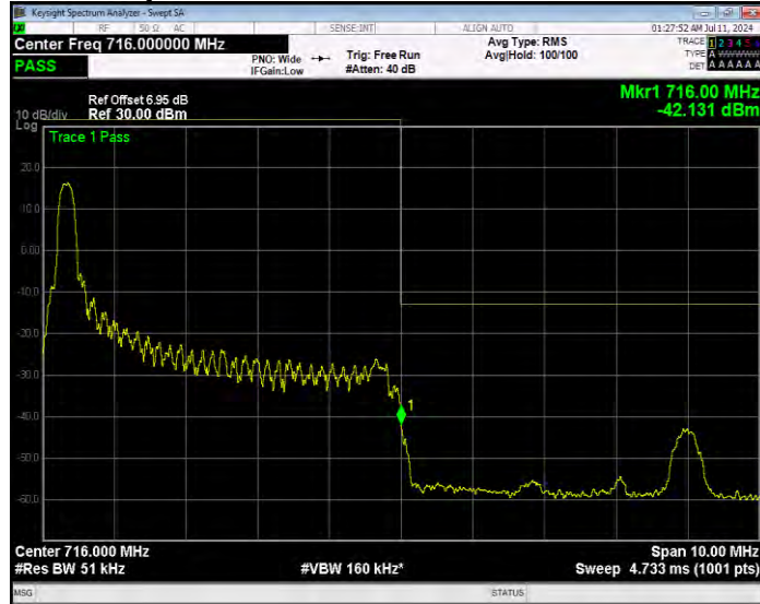
Band17 QPSK BW=5MHz Channel=23825 RB Size=1 Position=#Max Extended
