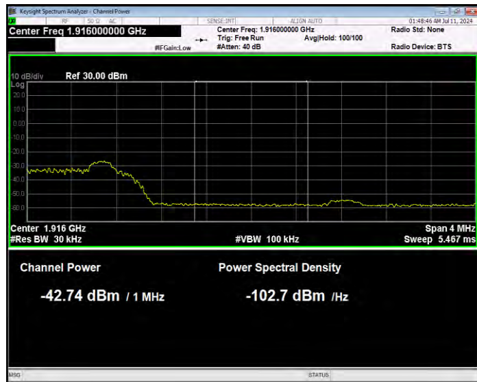
Band25 16QAM BW=5MHz Channel=26665 RB Size=1 Position=#0 Normal
