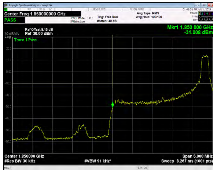
Band25 16QAM BW=3MHz Channel=26055 RB Size=15 Position=#0 Extended
