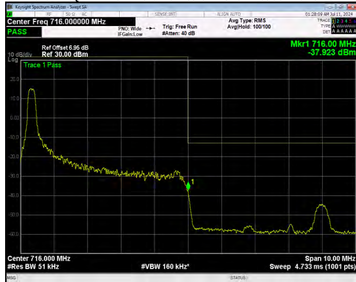
Band17 16QAM BW=5MHz Channel=23825 RB Size=1 Position=#Max Extended
