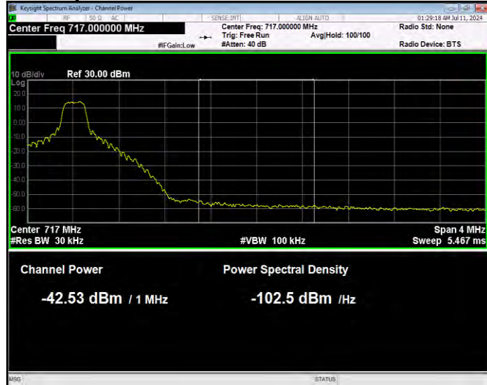
Band17 QPSK BW=10MHz Channel=23800 RB Size=1 Position=#Max Normal
