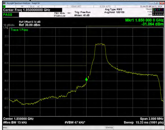
Band25 QPSK BW=1.4MHz Channel=26047 RB Size=1 Position=#Max Extended
