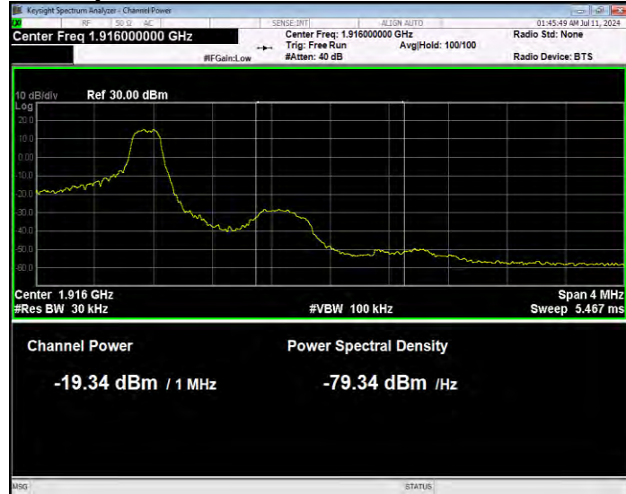
Band25 QPSK BW=1.4MHz Channel=26683 RB Size=1 Position=#Max Normal
