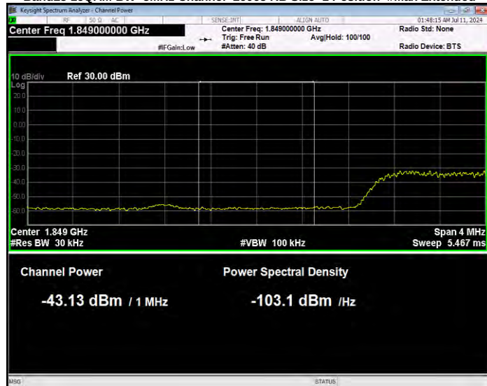
Band25 16QAM BW=5MHz Channel=26065 RB Size=1 Position=#Max Normal
