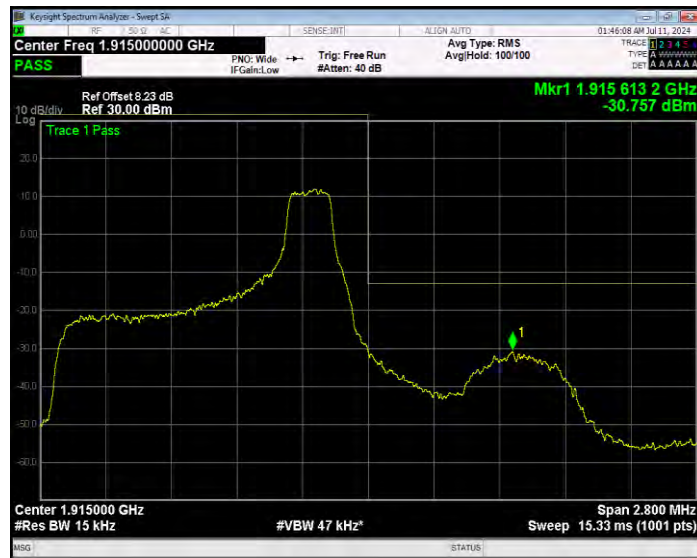
Band25 16QAM BW=1.4MHz Channel=26683 RB Size=6 Position=#0 Extended
