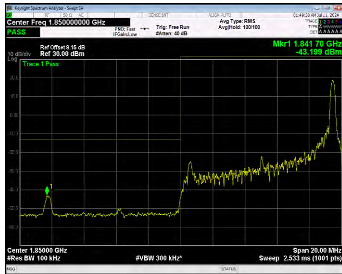
Band25 16QAM BW=10MHz Channel=26090 RB Size=50 Position=#0 Extended
