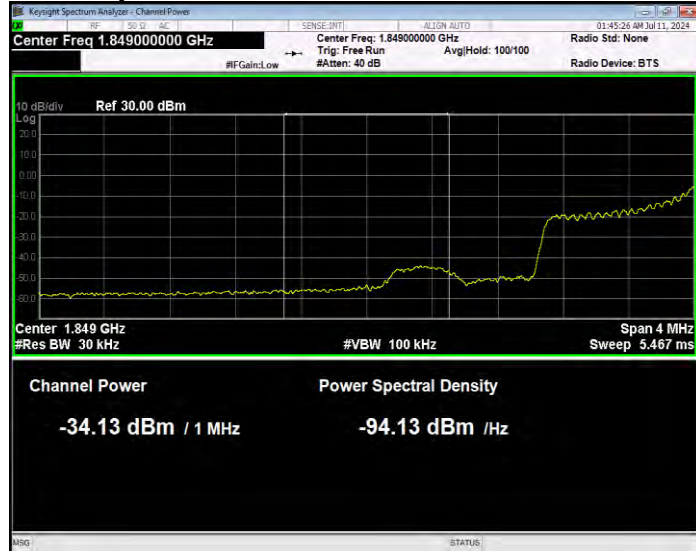
Band25 16QAM BW=1.4MHz Channel=26047 RB Size=1 Position=#Max Normal
