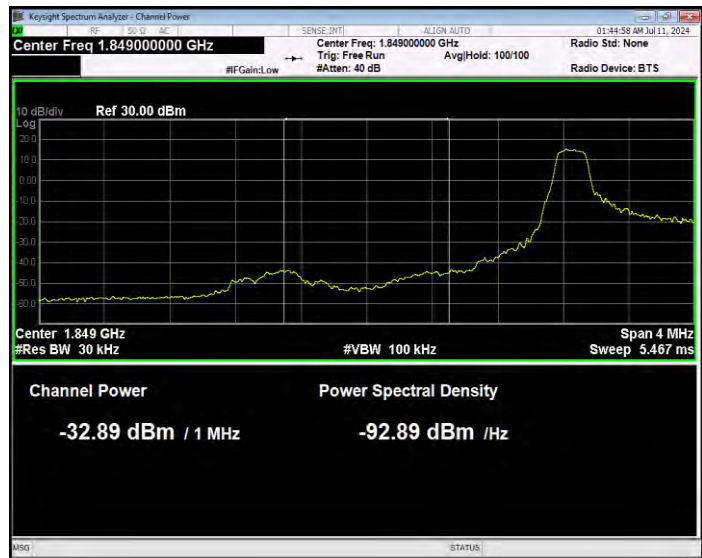
Band25 QPSK BW=1.4MHz Channel=26047 RB Size=1 Position=#0 Normal
