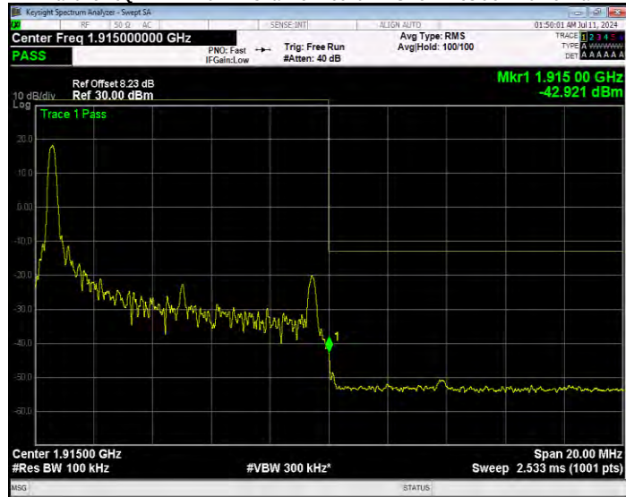
Band25 16QAM BW=10MHz Channel=26640 RB Size=1 Position=#Max Extended
