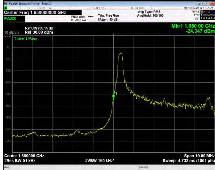
Band25 16QAM BW=5MHz Channel=26065 RB Size=1 Position=#Max Extended
