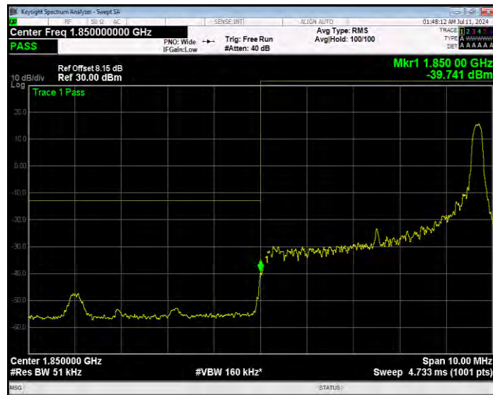
Band25 16QAM BW=5MHz Channel=26065 RB Size=25 Position=#0 Extended
