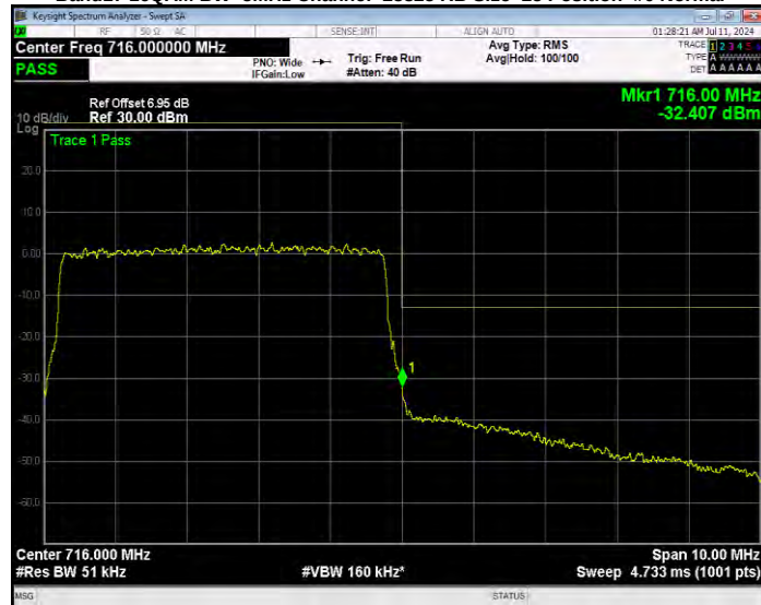
Band17 QPSK BW=10MHz Channel=23780 RB Size=1 Position=#0 Extended
