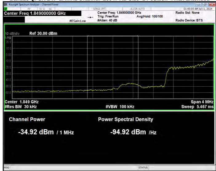
Band25 QPSK BW=1.4MHz Channel=26047 RB Size=1 Position=#Max Normal
