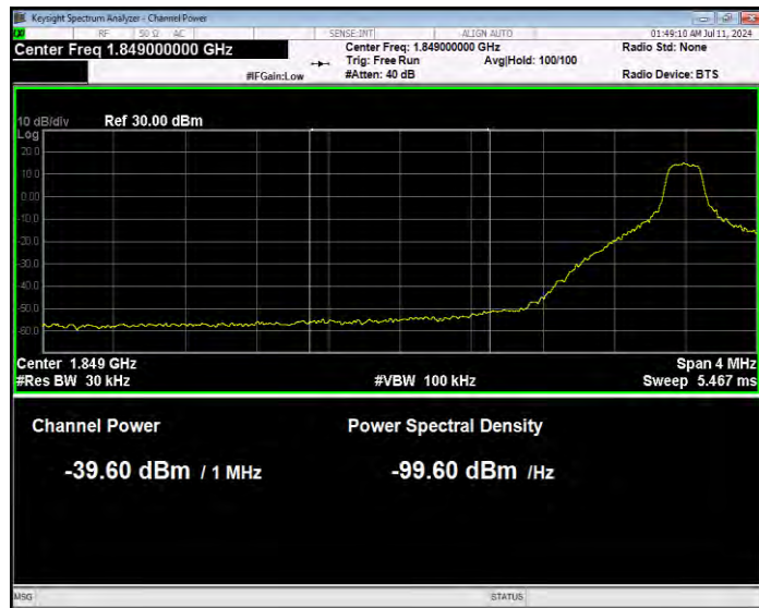
Band25 QPSK BW=10MHz Channel=26090 RB Size=1 Position=#0 Normal
