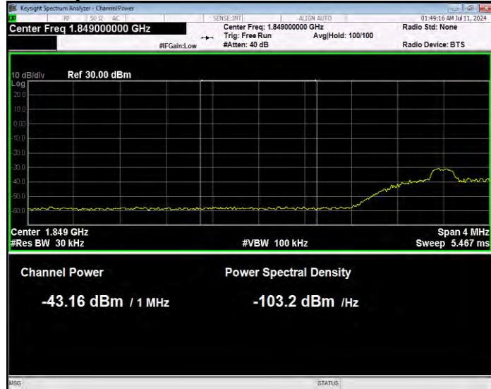
Band25 QPSK BW=10MHz Channel=26090 RB Size=1 Position=#Max Normal
