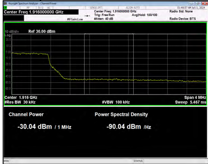
Band25 16QAM BW=5MHz Channel=26665 RB Size=25 Position=#0 Normal
