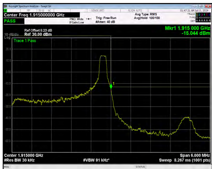
Band25 16QAM BW=3MHz Channel=26675 RB Size=15 Position=#0 Extended
