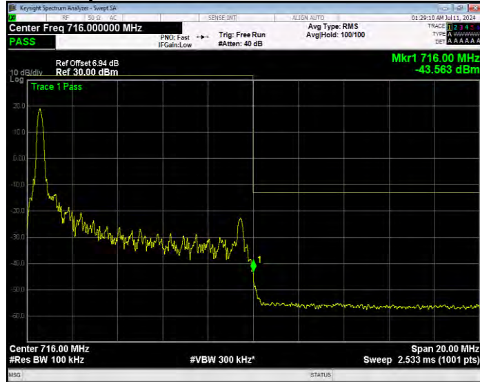
Band17 QPSK BW=10MHz Channel=23800 RB Size=1 Position=#Max Extended
