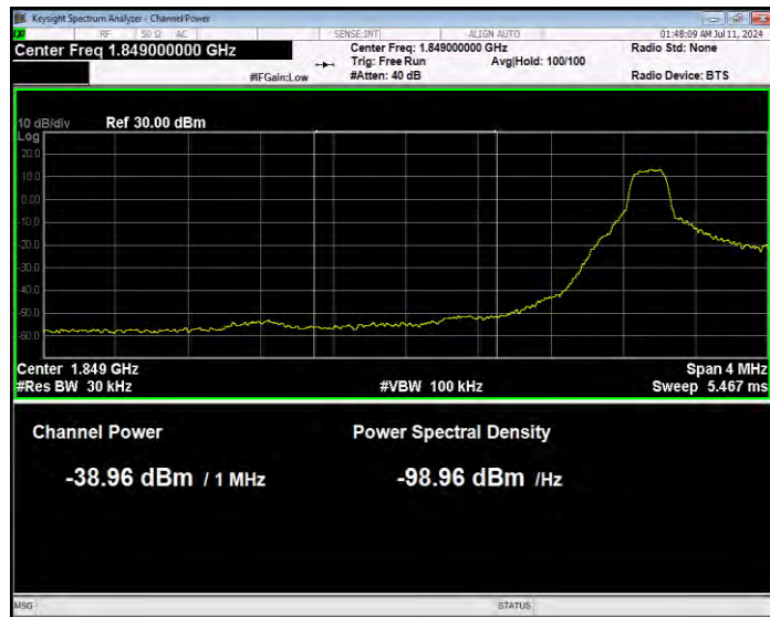
Band25 16QAM BW=5MHz Channel=26065 RB Size=1 Position=#0 Normal
