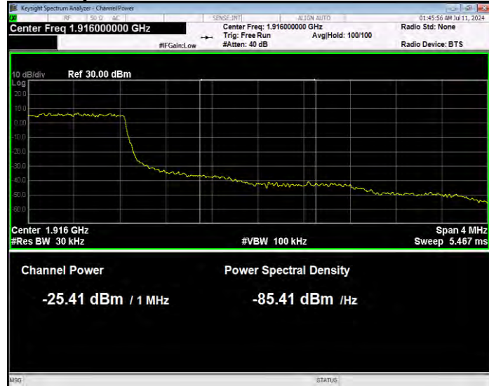
Band25 QPSK BW=1.4MHz Channel=26683 RB Size=6 Position=#0 Normal
