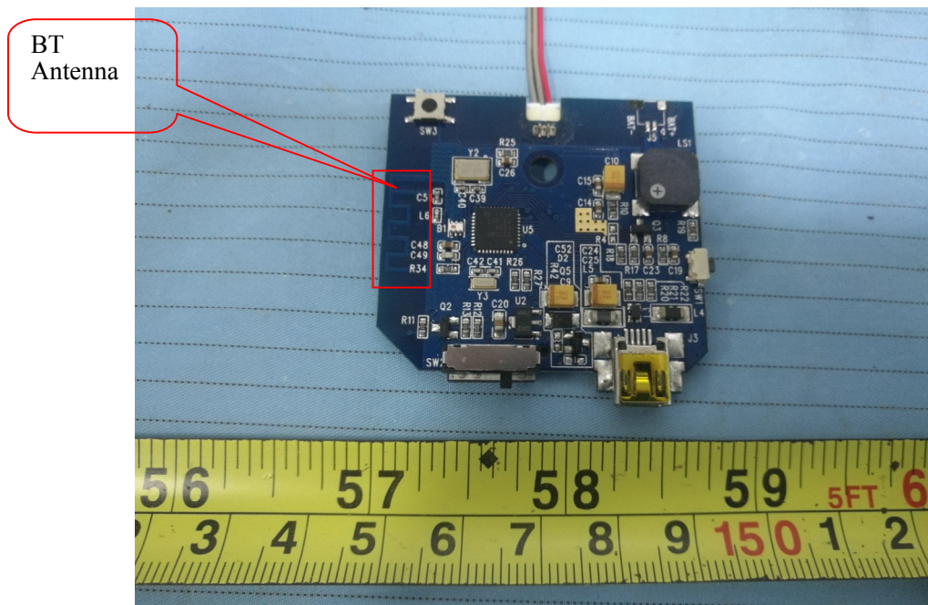
EUT – Printed Circuit Board 1 Bottom View
