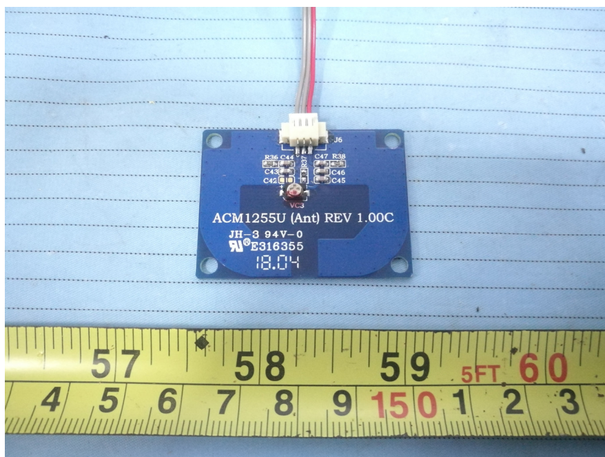
EUT – Printed Circuit Board 2 Bottom View
