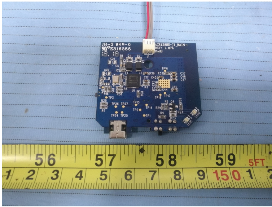
EUT – Printed Circuit Board 1 Top View
