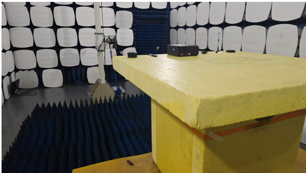
Radiated Spurious Emission, Above 1GHz
