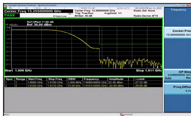
Band2-1.4MHz-16QAM-19193-1RB#0-PASS
