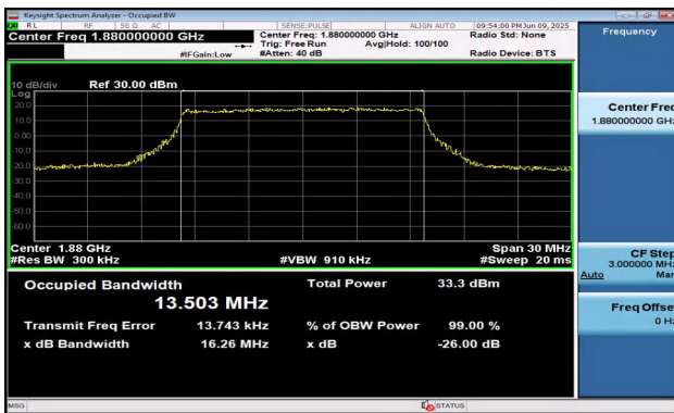
Band2-15MHz-QPSK-18900-75RB#0-PASS
