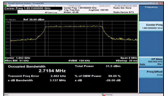
Band2-3MHz-16QAM-18615-15RB#0-PASS
