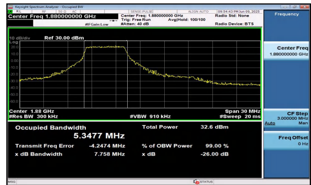
Band2-15MHz-16QAM-18900-27RB#0-PASS
