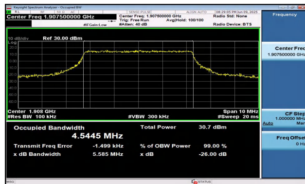
Band2-5MHz-16QAM-19175-25RB#0-PASS
