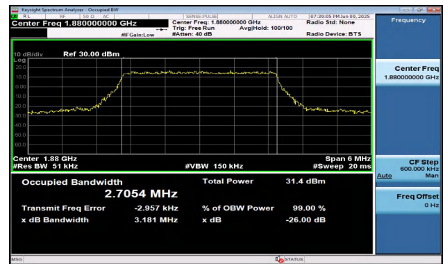
Band2-3MHz-16QAM-18900-15RB#0-PASS
