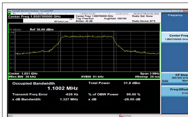
Band2-1.4MHz-QPSK-18607-6RB#0-PASS
