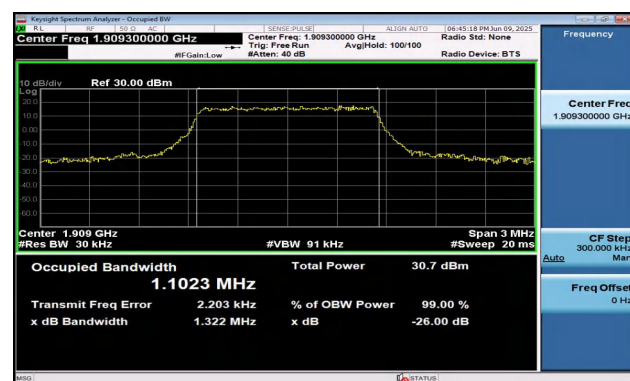
Band2-1.4MHz-16QAM-19193-6RB#0-PASS
