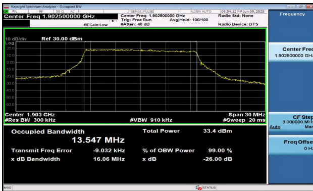
Band2-15MHz-QPSK-19125-75RB#0-PASS
