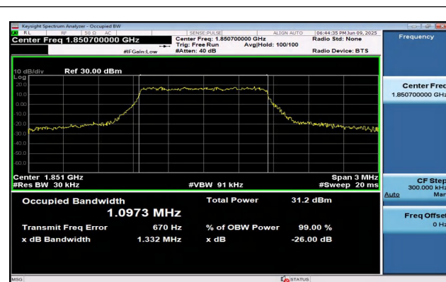
Band2-1.4MHz-16QAM-18607-6RB#0-PASS
