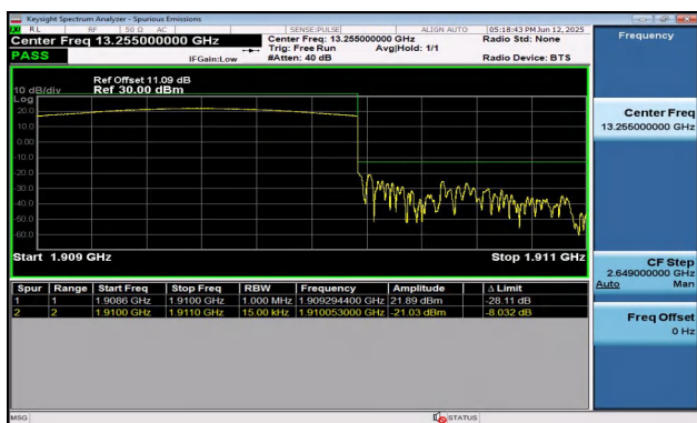
Band2-1.4MHz-QPSK-19193-6RB#0-PASS
