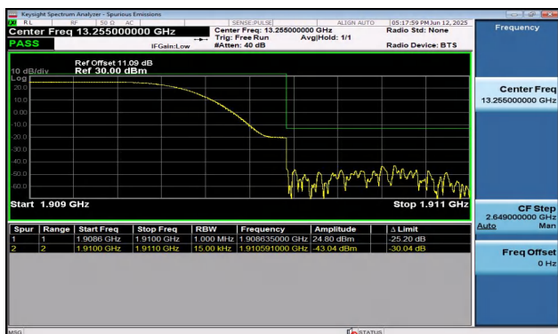
Band2-1.4MHz-QPSK-19193-1RB#0-PASS
