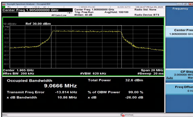
Band2-10MHz-QPSK-19150-50RB#0-PASS
