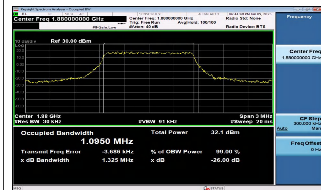
Band2-1.4MHz-QPSK-18900-6RB#0-PASS
