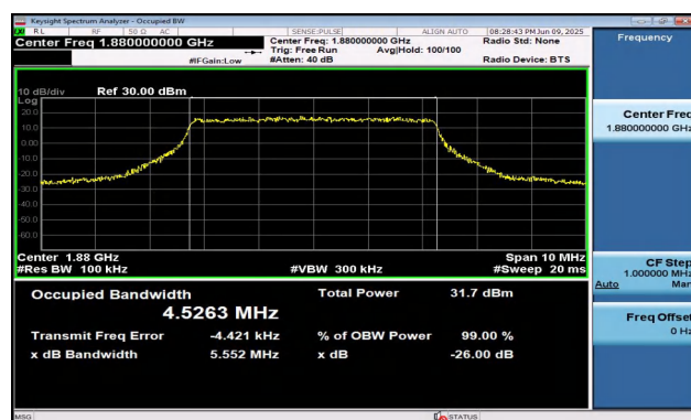
Band2-5MHz-16QAM-18900-25RB#0-PASS
