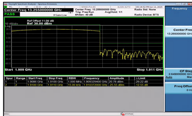
Band2-1.4MHz-16QAM-19193-6RB#0-PASS
