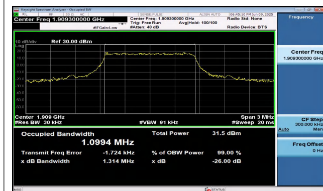
Band2-1.4MHz-QPSK-19193-6RB#0-PASS
