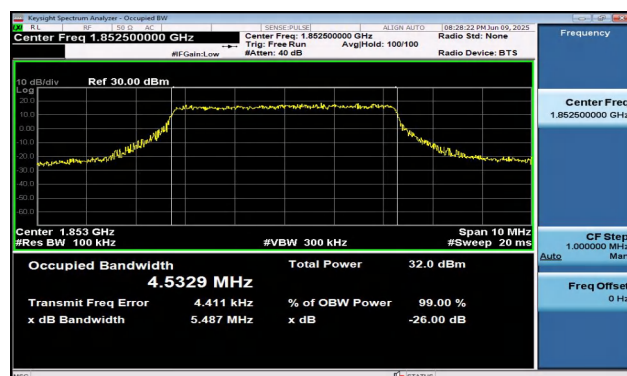
Band2-5MHz-16QAM-18625-25RB#0-PASS
