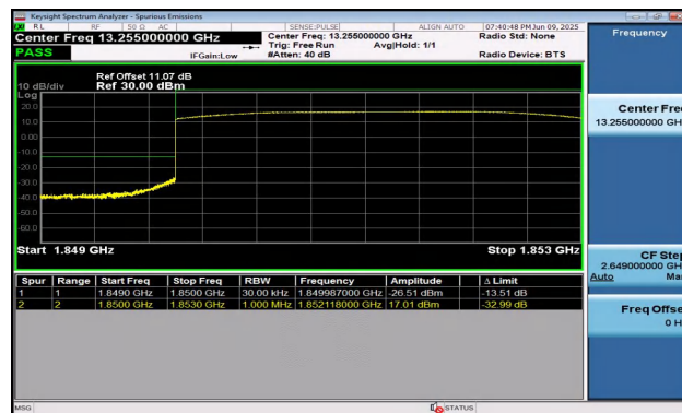
Band2-3MHz-16QAM-18615-15RB#0-PASS
