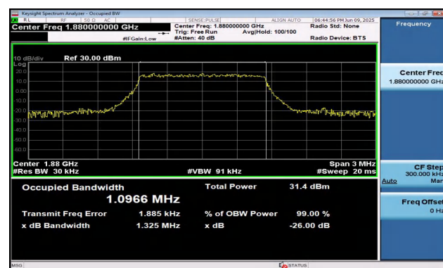
Band2-1.4MHz-16QAM-18900-6RB#0-PASS
