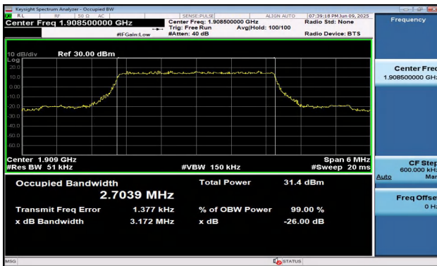
Band2-3MHz-QPSK-19185-15RB#0-PASS
