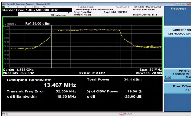
Band2-15MHz-QPSK-18675-75RB#0-PASS
