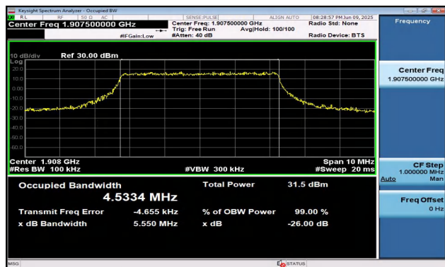
Band2-5MHz-QPSK-19175-25RB#0-PASS
