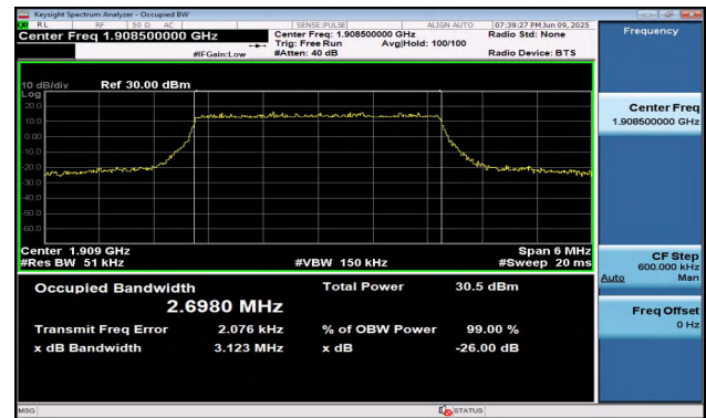
Band2-3MHz-16QAM-19185-15RB#0-PASS
